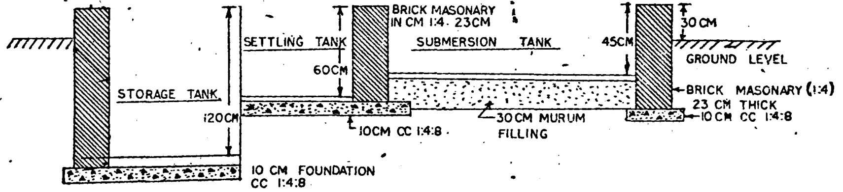
CROSS SECTION
