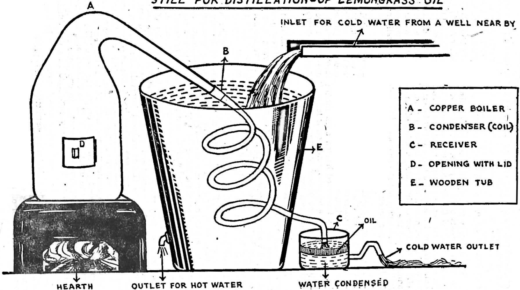
Fig. 32. Home-made country still for distillation of lemongrass oil
