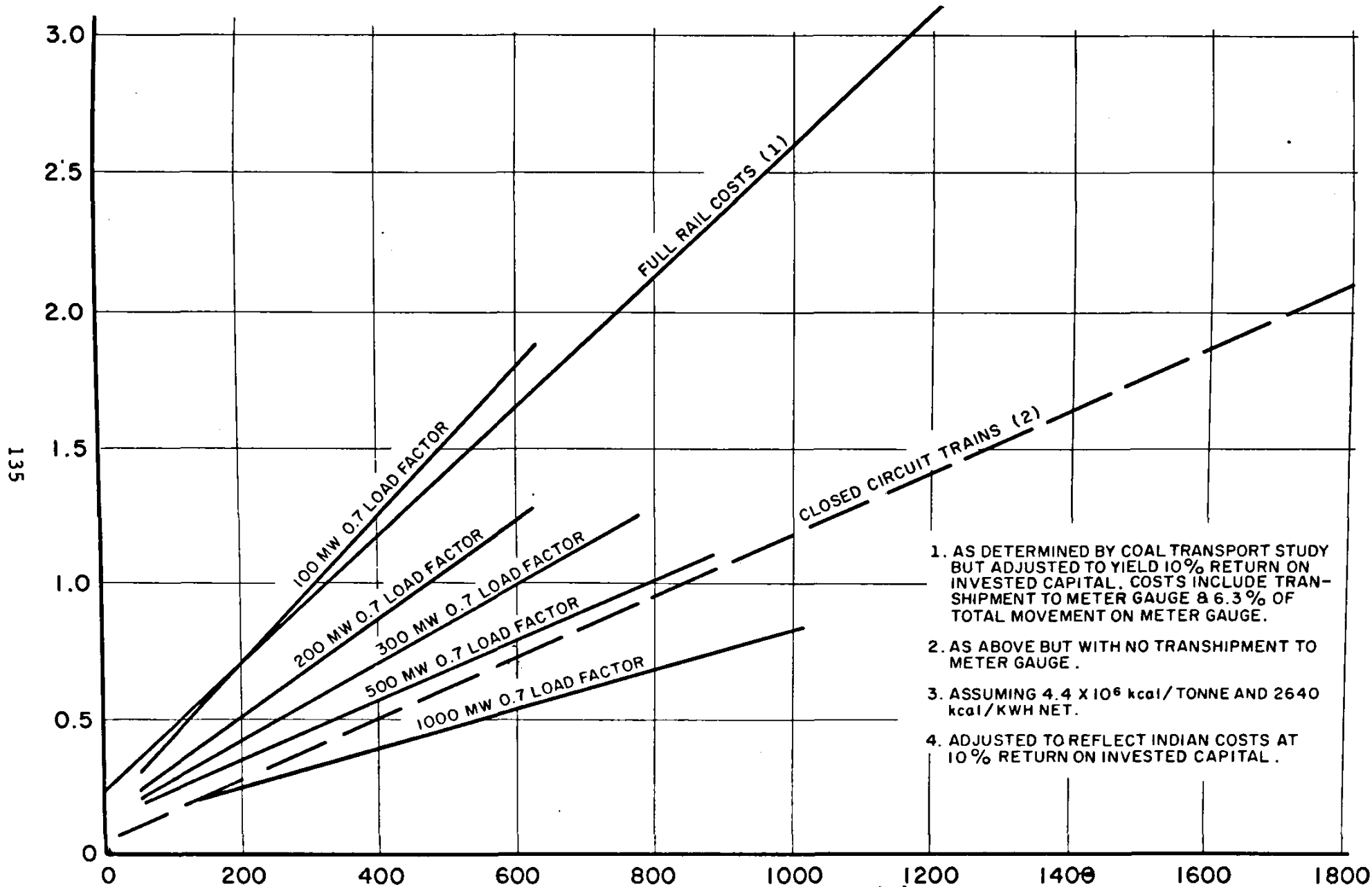
FIGURE 12-RAIL FREIGHT AT 1962/3 COSTS IN np / KWH (3) VS. EHV TRANSMISSION COSTS IN np/KWH (4)
