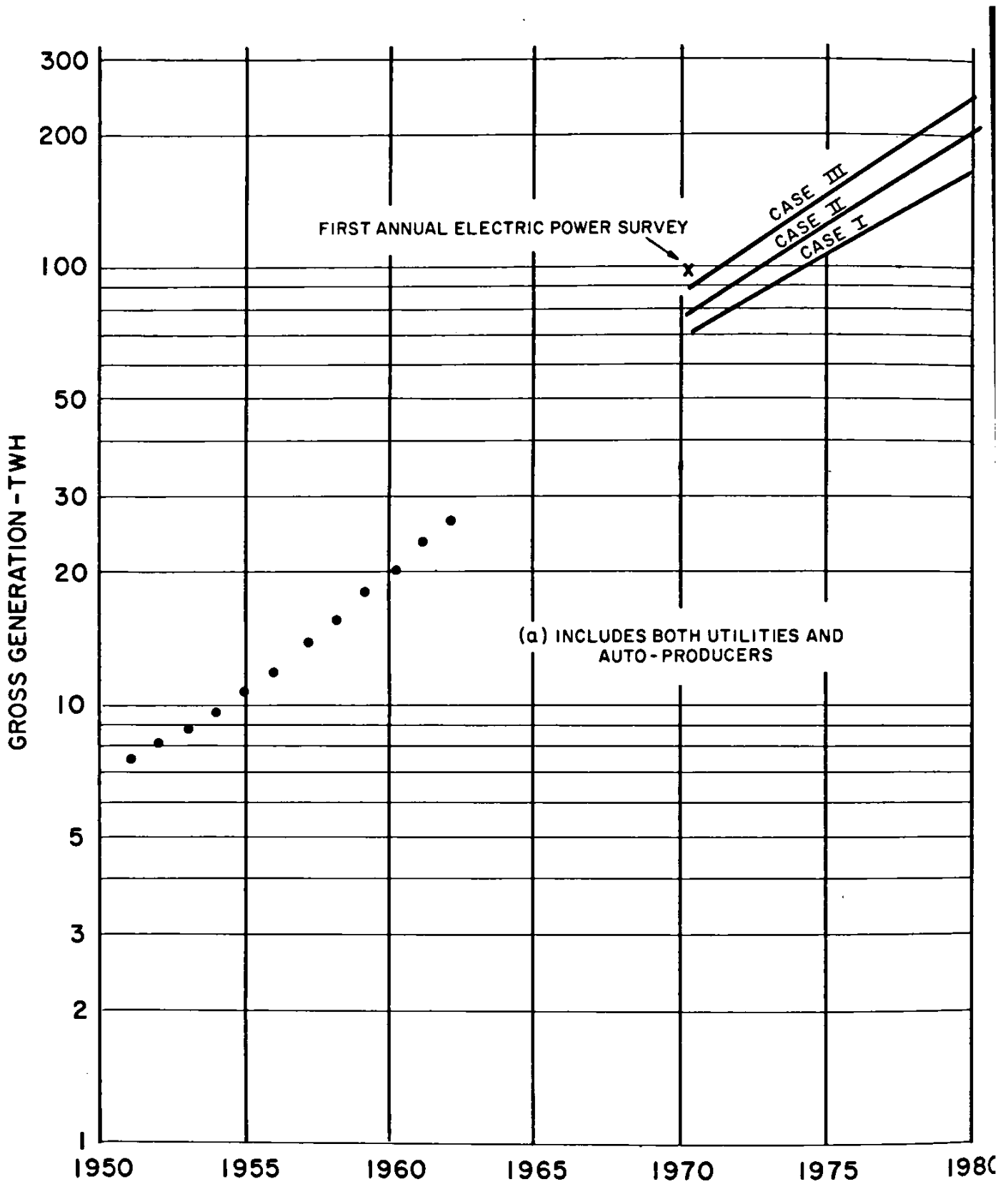
FIGURE 13-ESTIMATED ELECTRICITY REQUIREMENTS (a) 1951 TO 1980/1 (GROSS GENERATION TWH )
