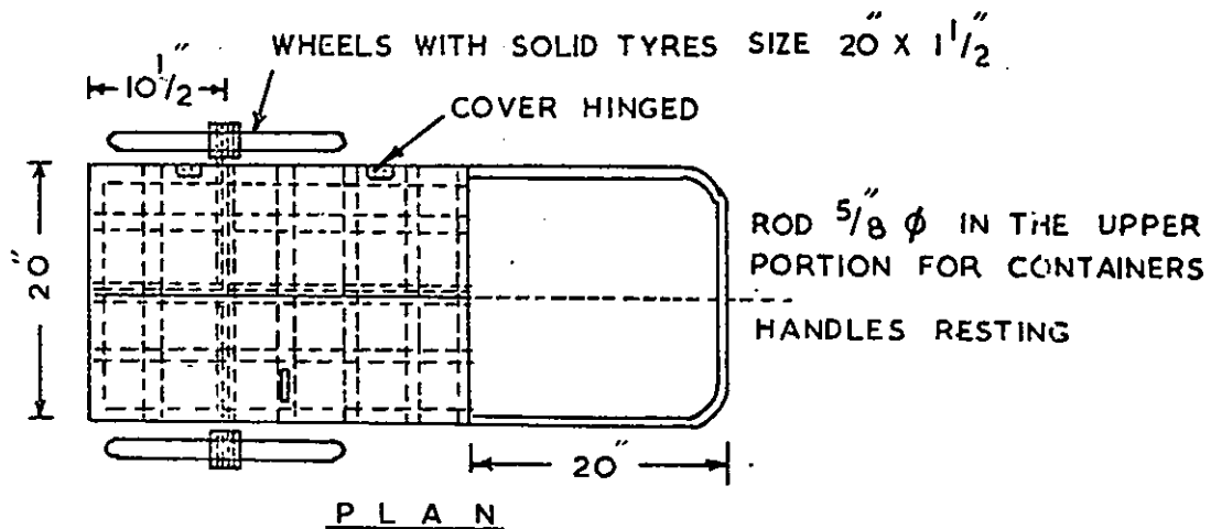
WHEEL BARROW CLOSED TYPE CAPACITY 17 GALLONS
