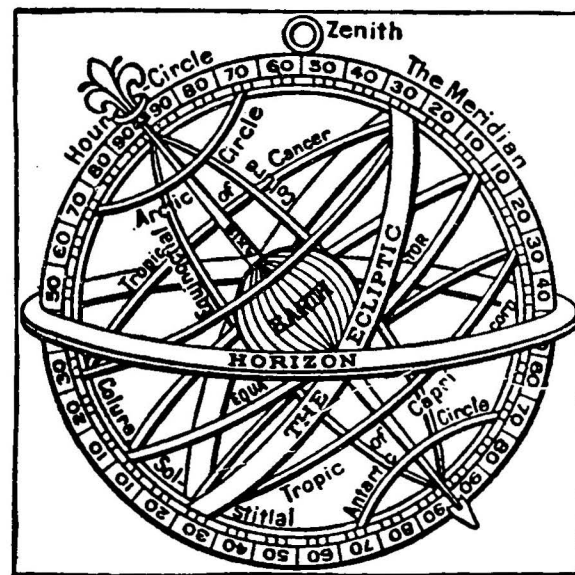
Fig. 18—Armillary sphere. (Reproduced from Encyclopaedia Britannica ).
