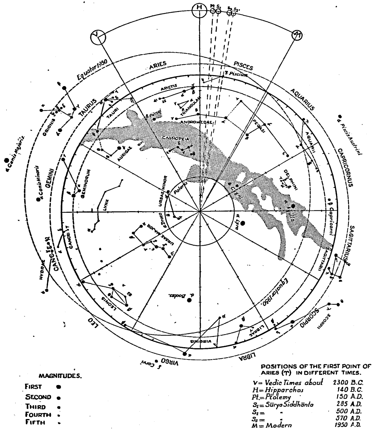
Fig. 19—The Zodiac through ages.
