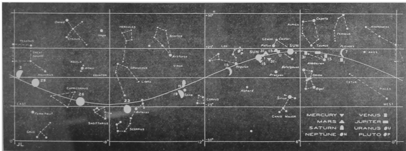
Fig. 3—Showing the positions of the sun, moon and planets among the stars in July, 1953.
