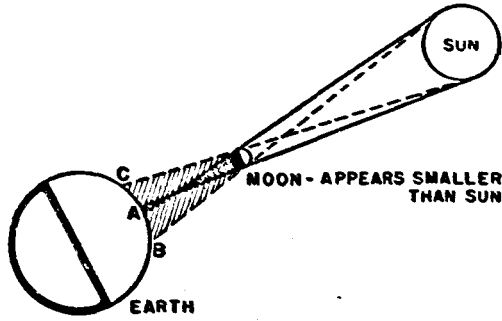
Fig. 5—Showing an annular eclipse of the sun.
