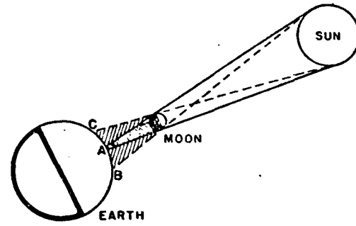
Fig. 6—Showing a total eclipse of the sun.
