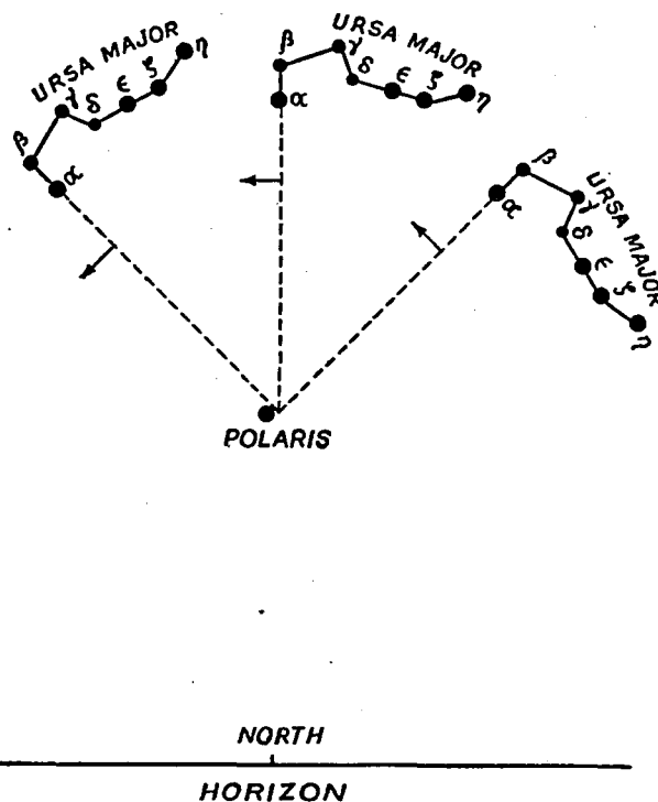
Fig. 8—Showing the positions of Ursa Major ( Saptarṣi ) at interval of 3 hours.
