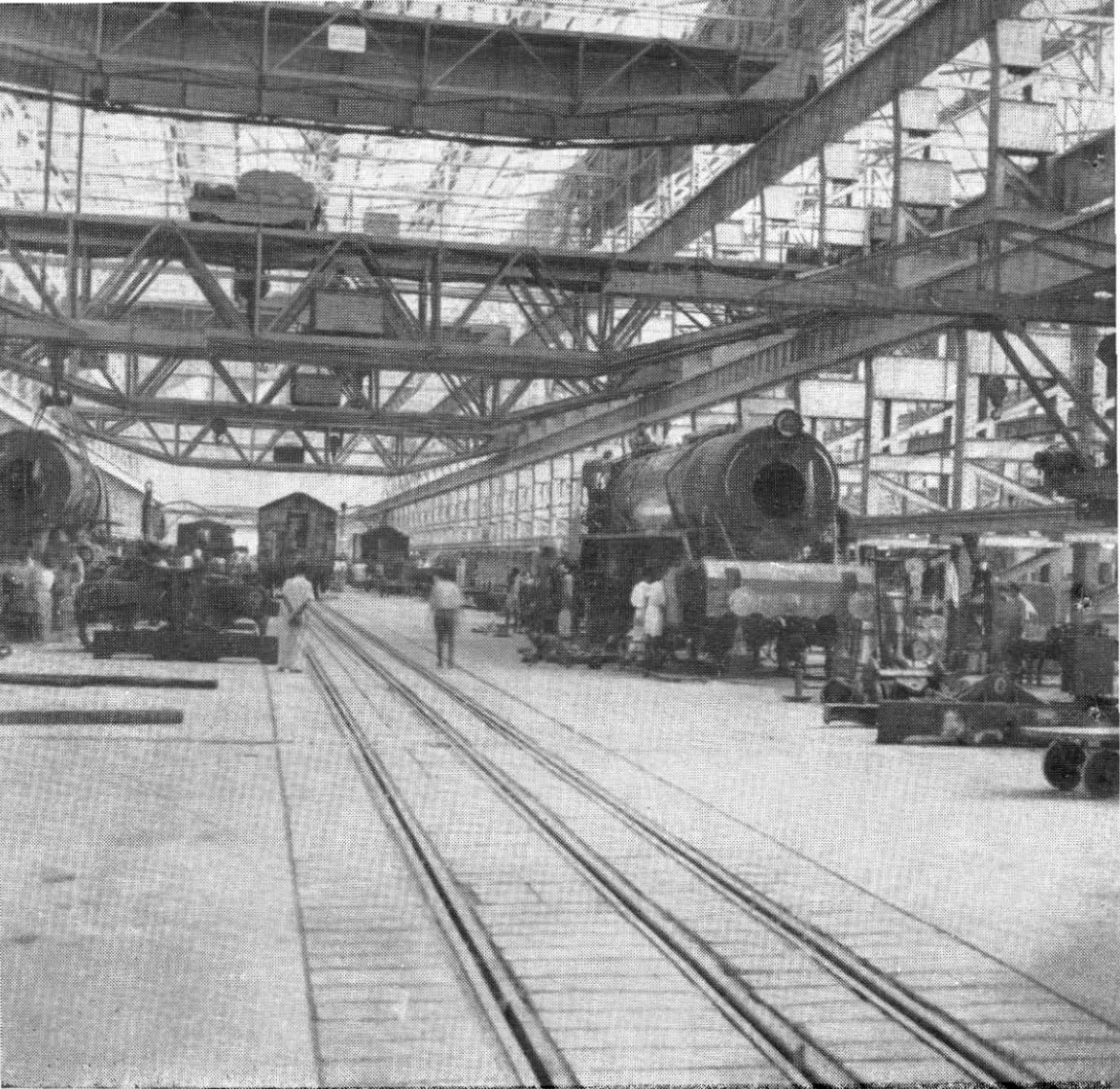
An assembly shop at the Chittaranjan Locomotive Factory
