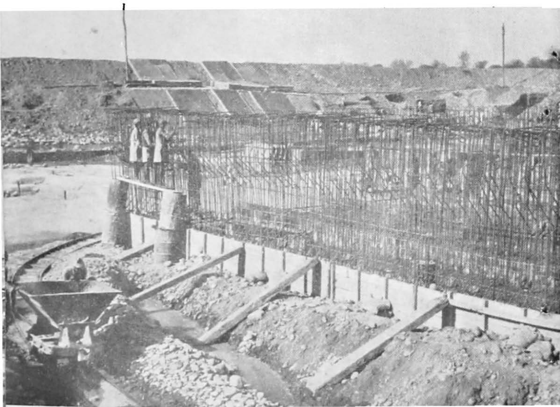
Bhakra Nangal Project. Construction of cross drainage works for hill streams
