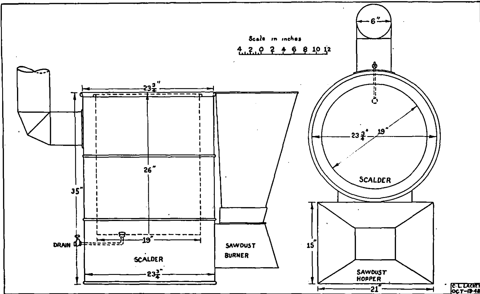
FIG. 10—Scalding for No. 1 Cannery
