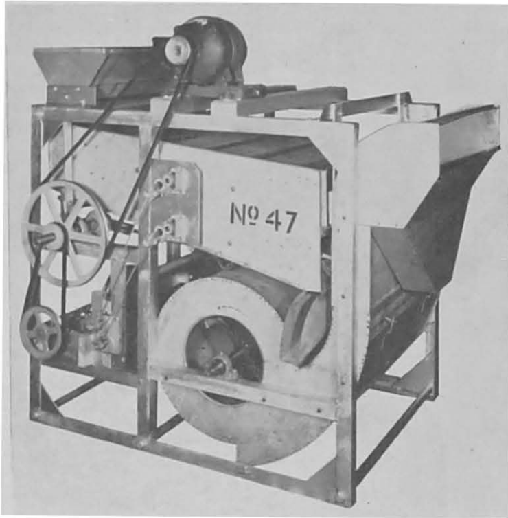
FIG. 39—Pea Cleaner
