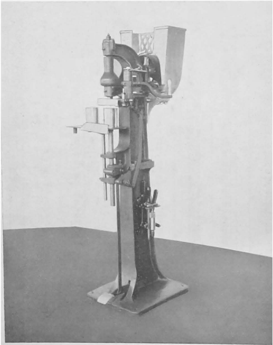
FIG. 4—Hand-operated Capper for No. 1 Size Cannery
