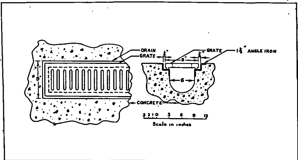
FIG. 1—Detail of Floor Drain
