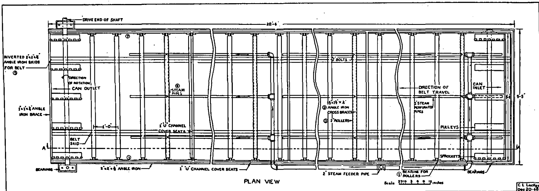
FIG. 23—Plan View of Cooker for No. 3 Cannery
