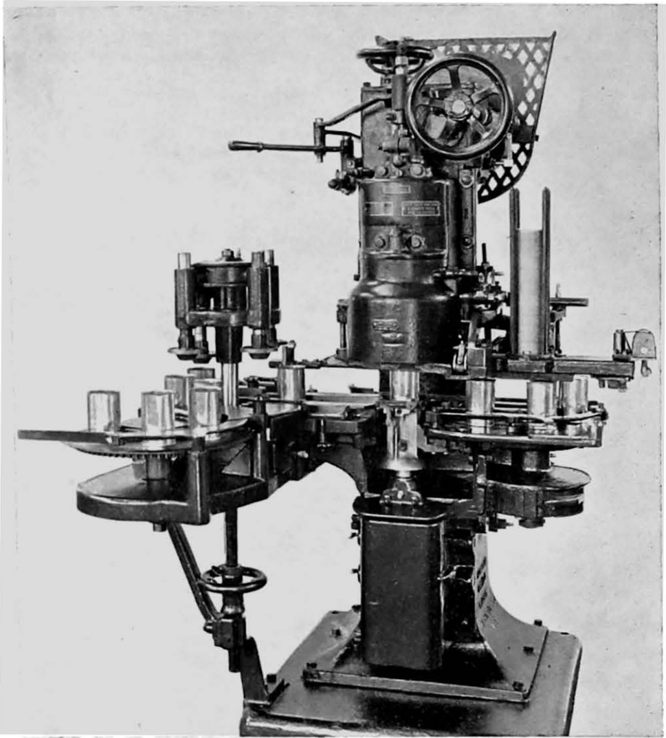
FIG. 6—Capper with Mechanical Lid Feed, Rolls and Can Conveyor for Size No. 3 and Larger Canners
