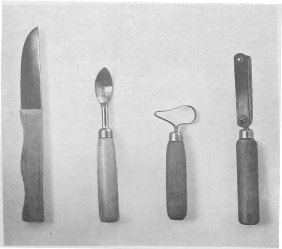
FIG. 2—Preparation Utensils (Left to right) Cannery knife, peach pitting spoon, pear coring loop, and pear paring knife.
