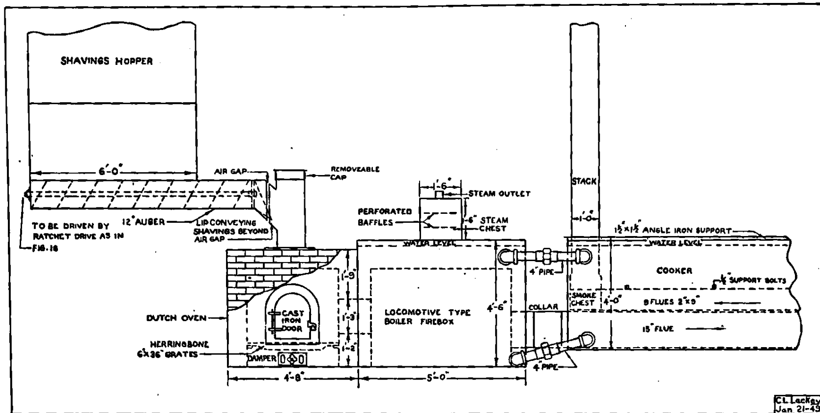
FIG. 20—Boiler Firebox Equipped with Dutch Oven and Shavings Hopper for No. 2 Cannery Cooker.
