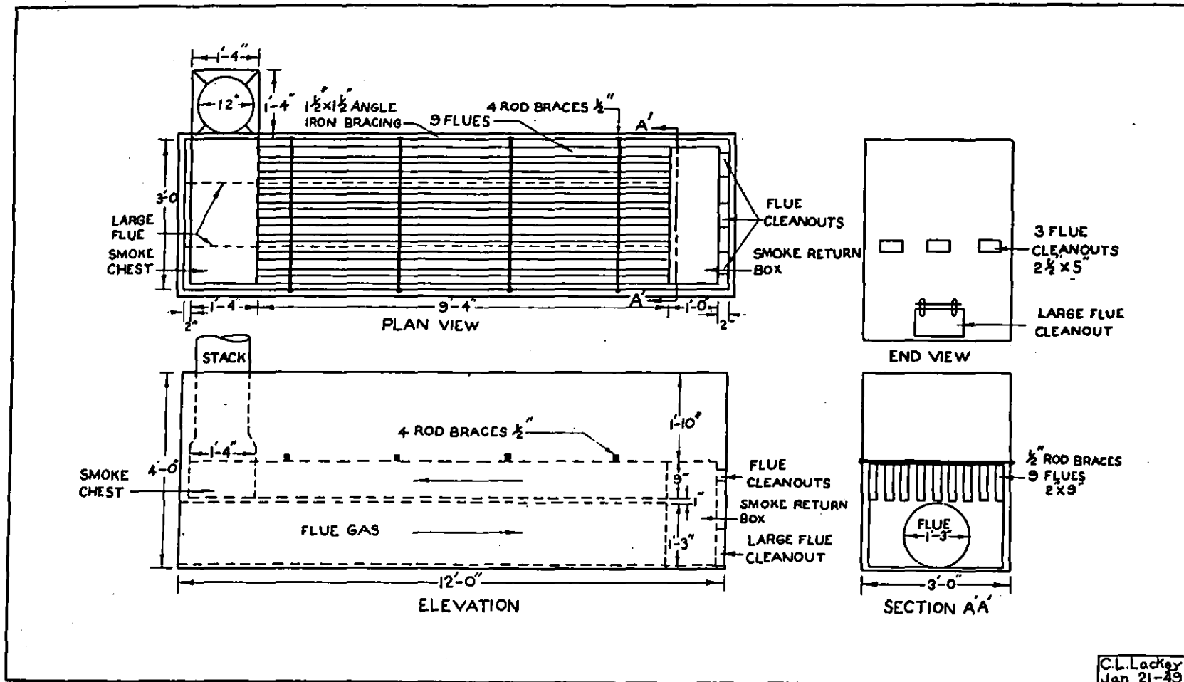
FIG. 18—Cooker for No. 2 Cannery
