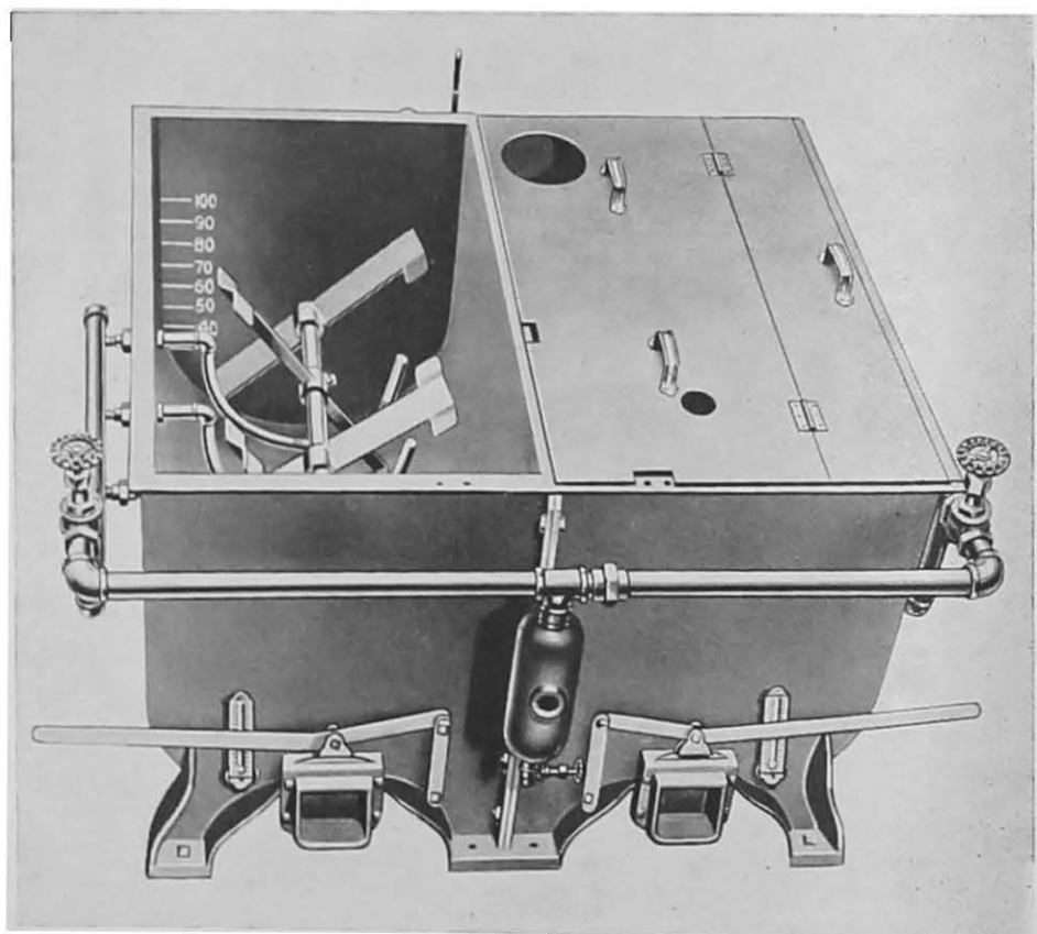
FIG. 37—Duplex Batch Cream Style Corn Mixer
