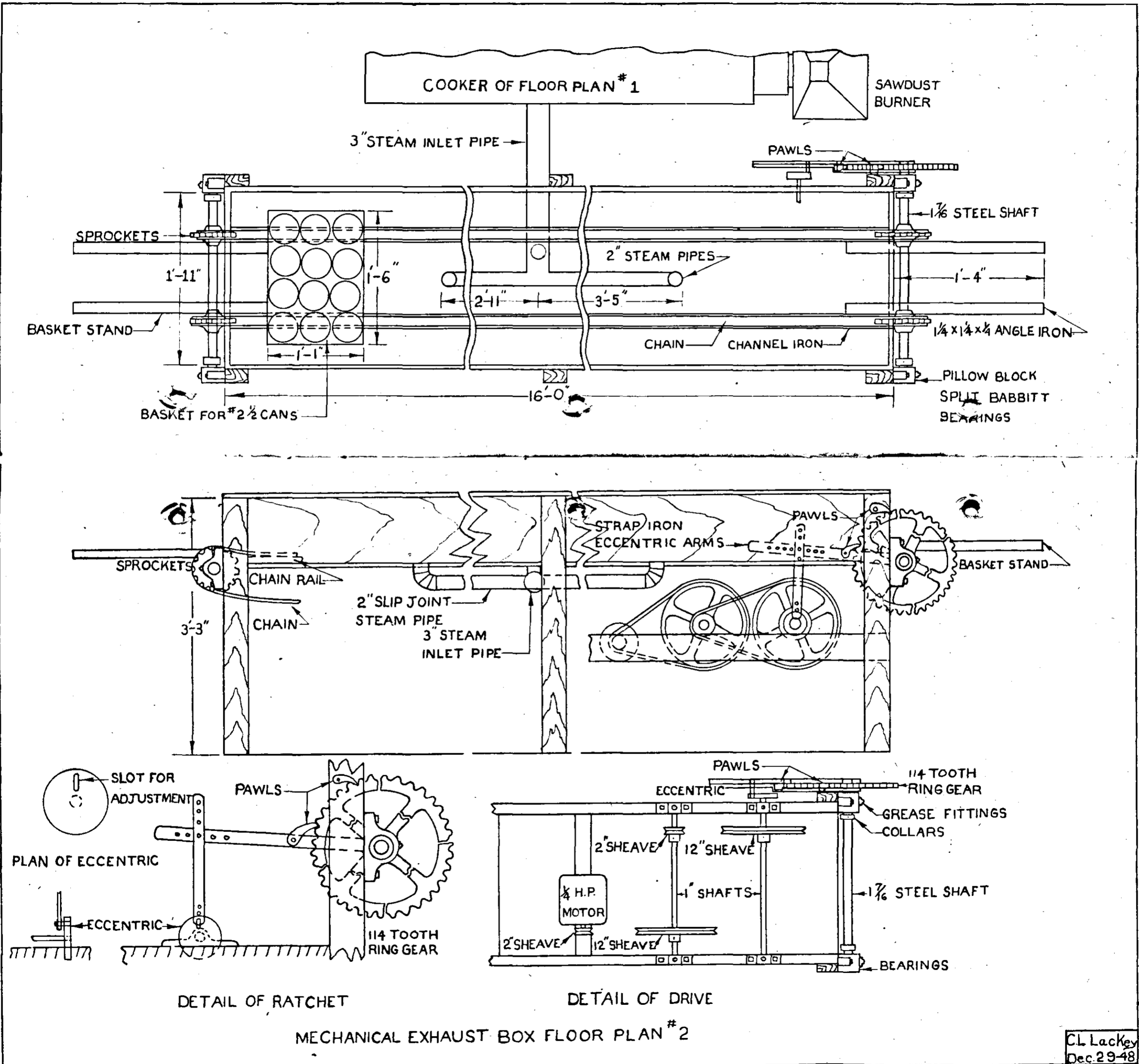
FIG. 17—Mechanical Exhaust Box for No. 2 Cannery
