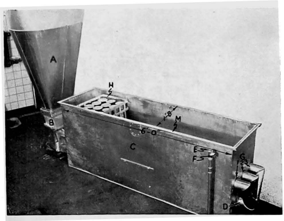
FIG. 12—No. 1 Cannery Cooker
