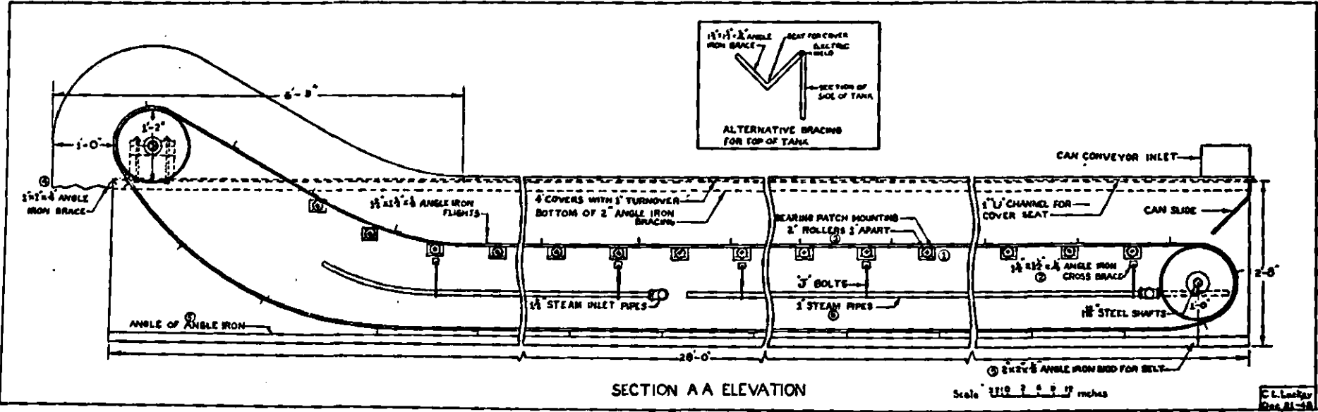
FIG. 23(A)—Elevation of Cooker for No. 3 Cannery
