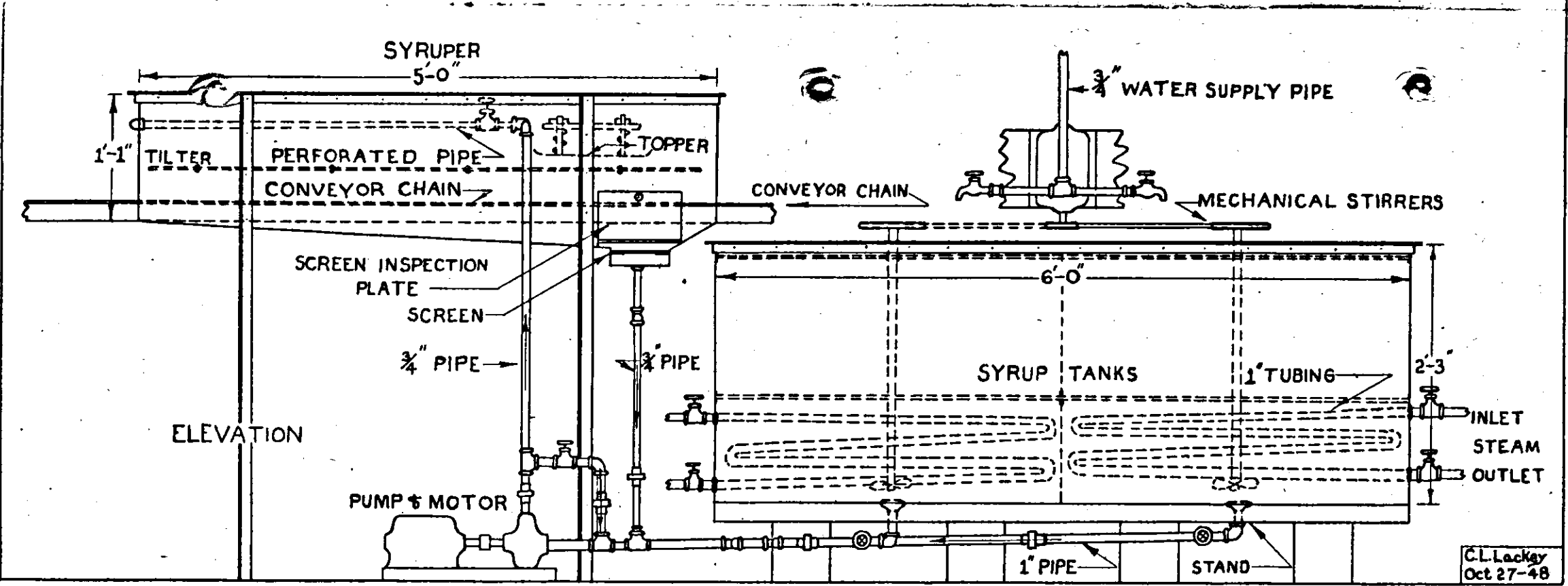
FIG. 16—Plan View and Elevation of Syruper for No. 2 and No. 3 Cannery
