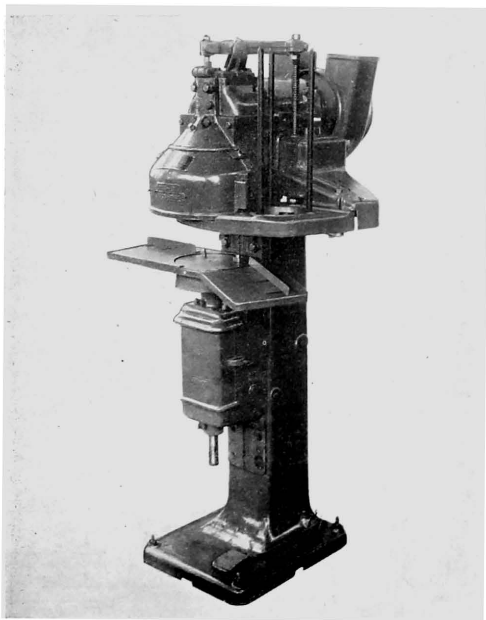
FIG. 5—Copper with Mechanically-operated Lid Feed and Rolls for Size No. 2 Cannery.
