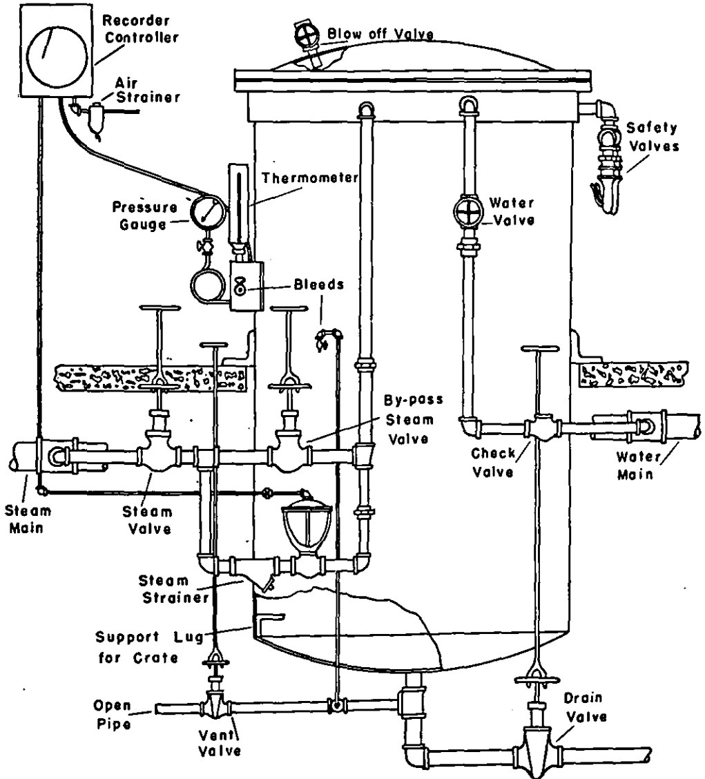
FIG. 30—Vertical Retort Equipped with Top Steam Inlet
