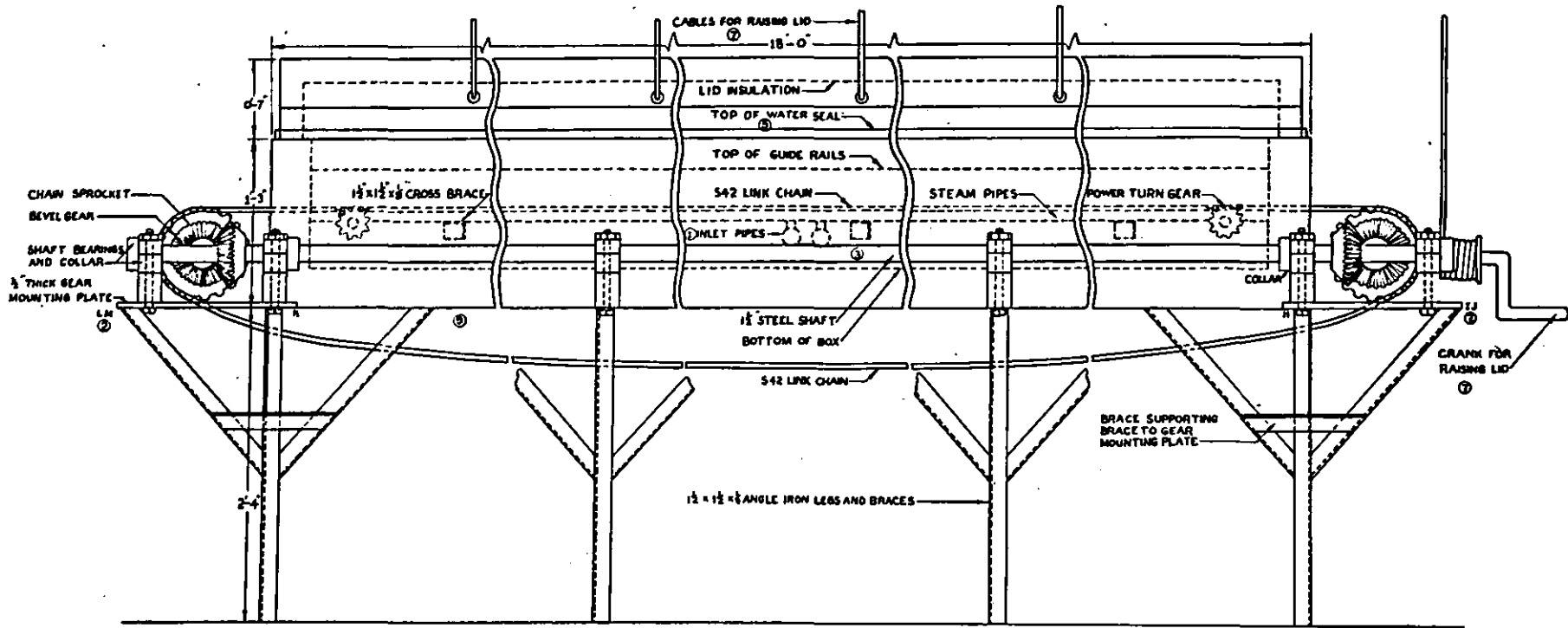
SIDE ELEVATION No 2
