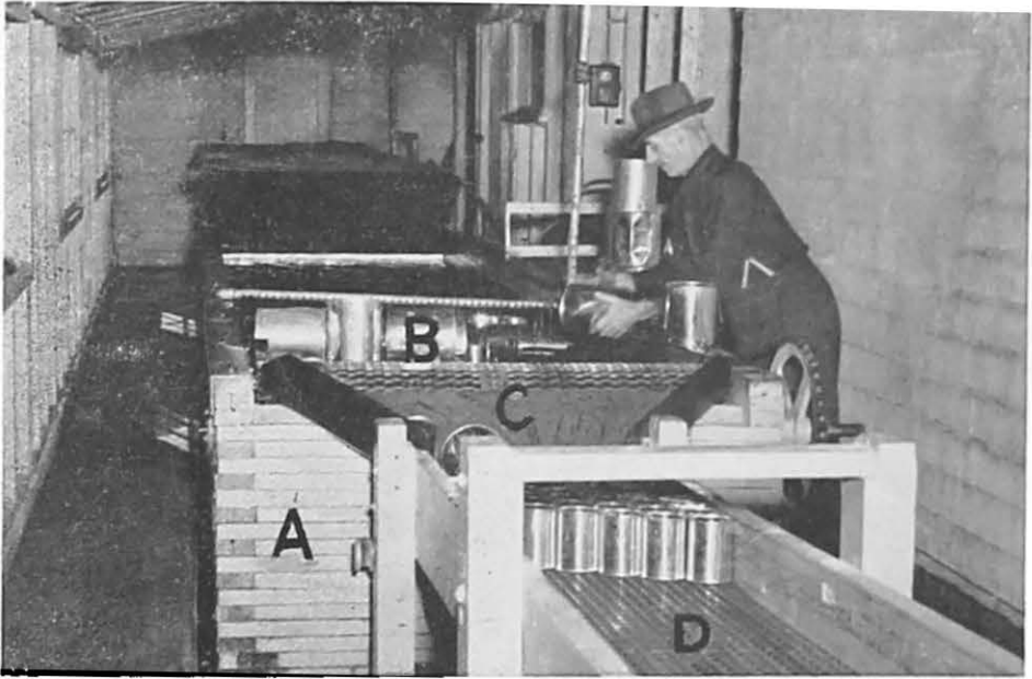
FIG. 23(B)—End View of Cooker and Cooler in No. 3 Cannery
