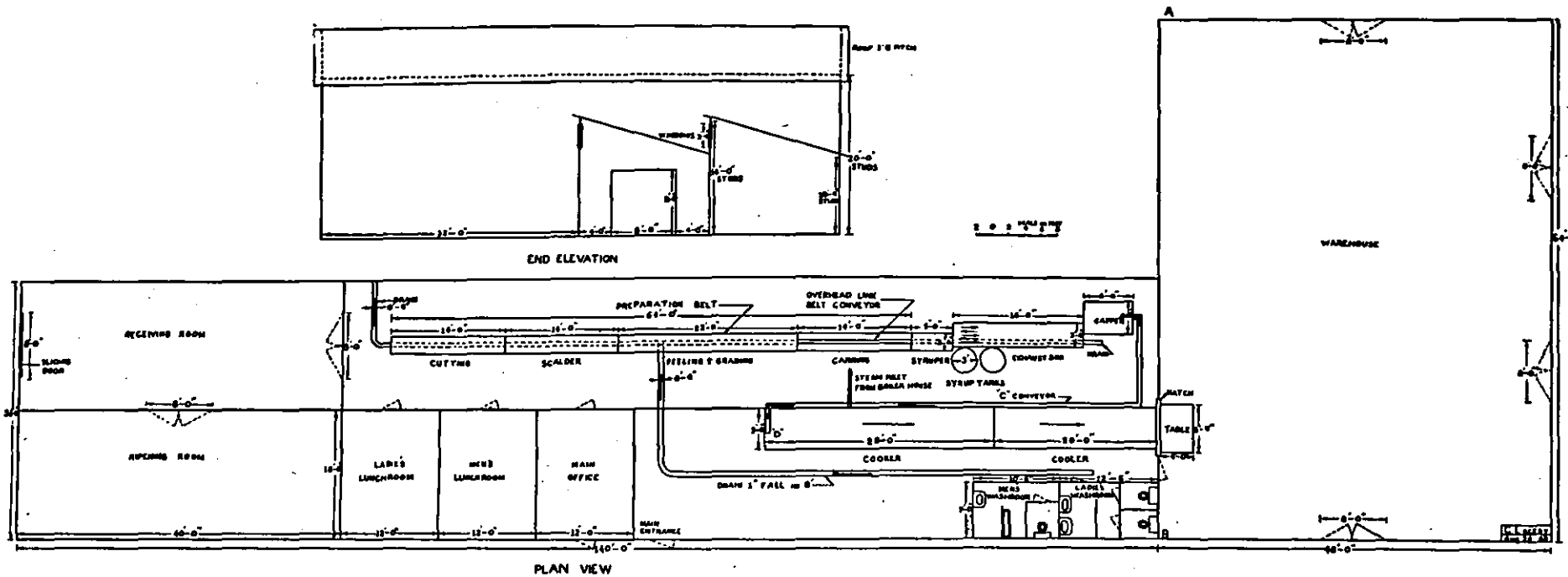
FIG. 21—Floor Plan and Elevation of No. 3 Cannery
