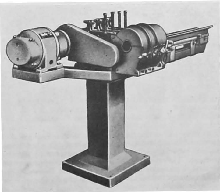
FIG. 36—Corn Cutter
