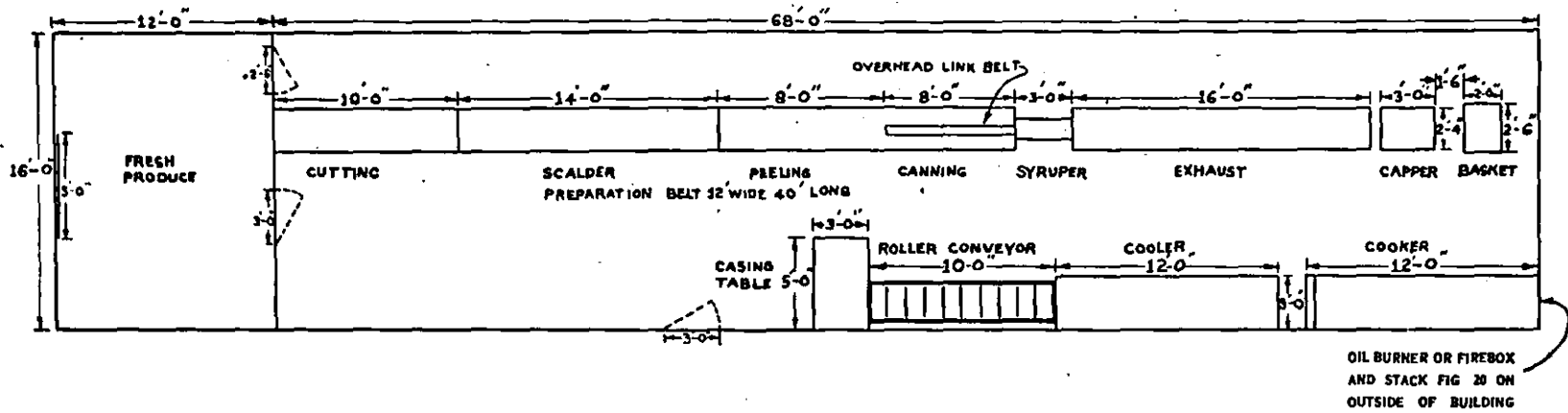
Fig. 15—Floor Plan of No. 2 Cannery
