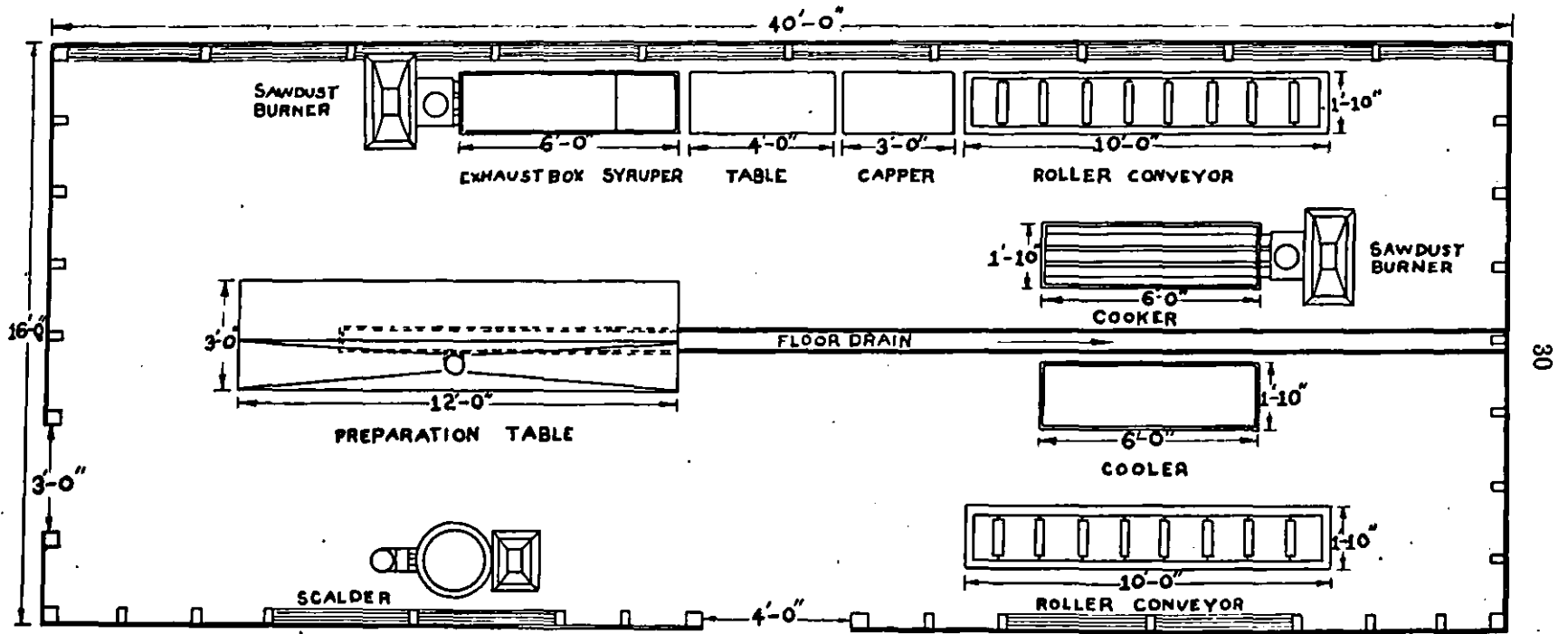
FIG. 9—Floor Plan of No. 1 Cannery
