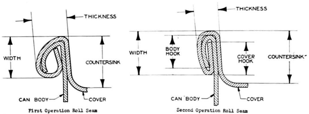
FIG. 7—Description of Double Seam
