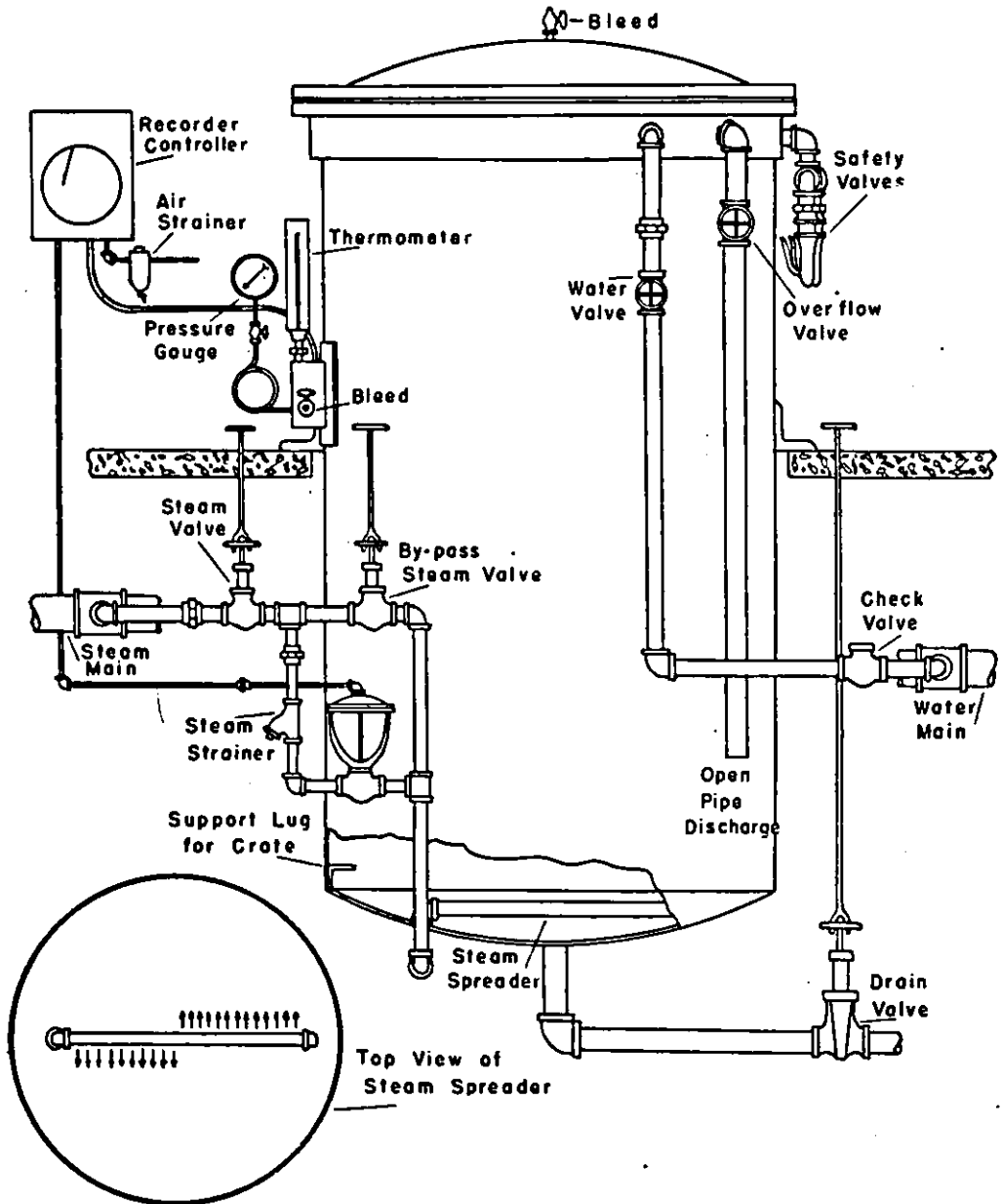
FIG. 29—Vertical Retort Equipped with Bottom Steam Inlet
