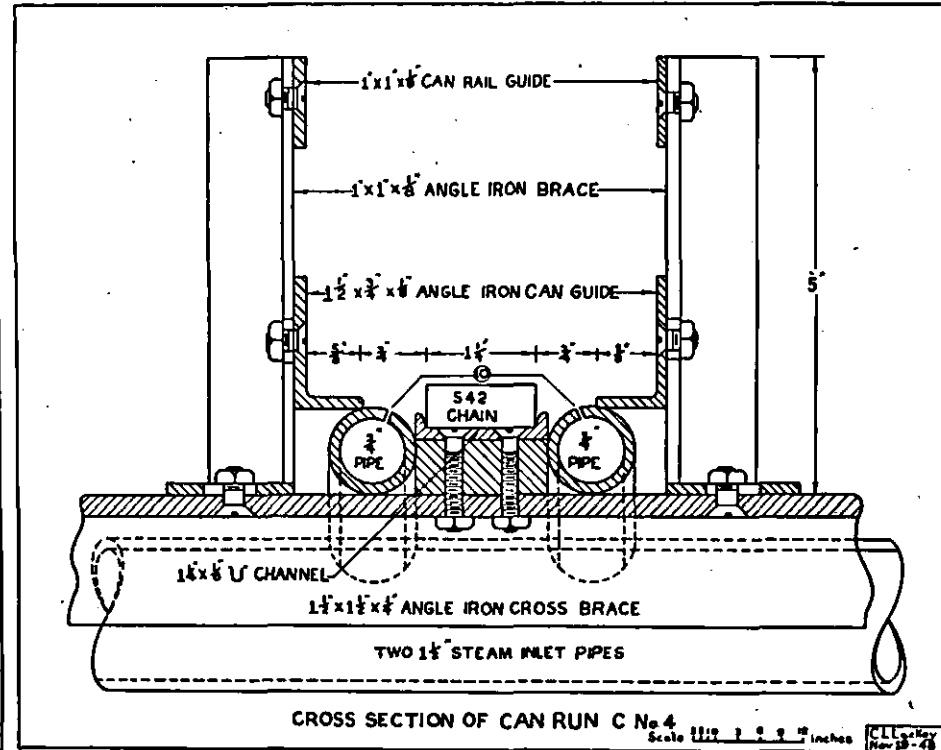
Fig. 22(C)—Detail of a Single Run
