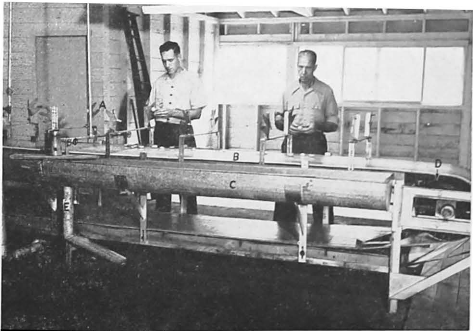
FIG. 24—Starting End of Preparation Belt in No. 3 Cannery .
