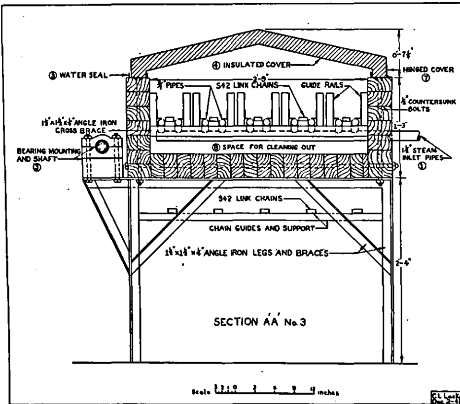
Fig. 22(B)—Section
