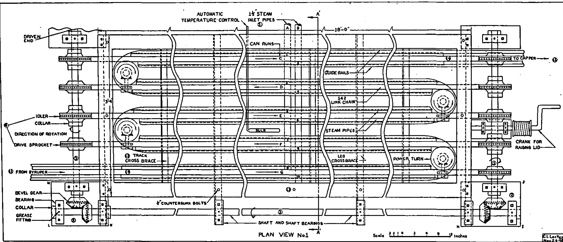
FIG. 22—Exhaust Box for No. 3 Cannery—Plan View
