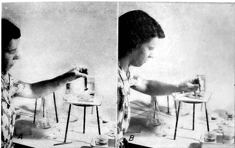
FIGURE 14.—The impregnated specimen is removed from the monomer liquid with tweezers (A); it is then placed in position on the previously hardened base in the mold (B).
