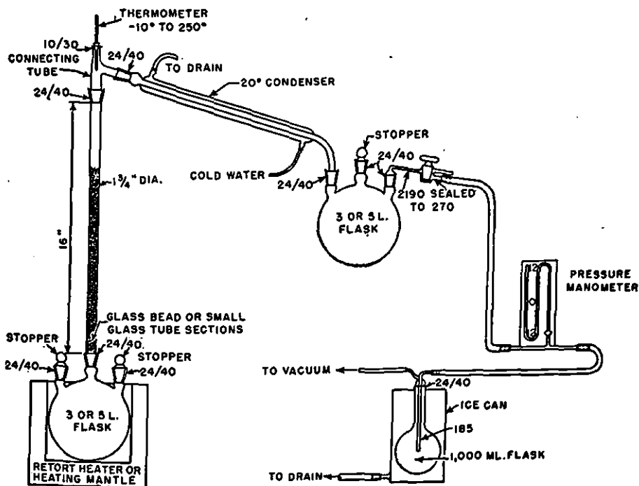
FIGURE 10.—Arrangement of glass apparatus for vacuum distillation of inhibited methacrylate-monomer liquid. This apparatus should be operated under a fume hood. (Courtesy of E. I. du Pont de Nemours & Co. (Inc.), Plastics Dept.)
