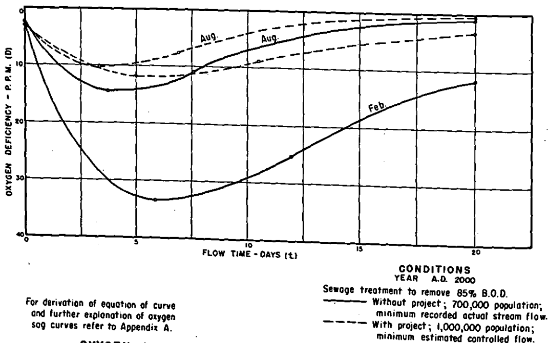
OXYGEN SAG CURVES FOR MINIMUM FLOW IN YEAR A.D. 2000 FIGURE 2
