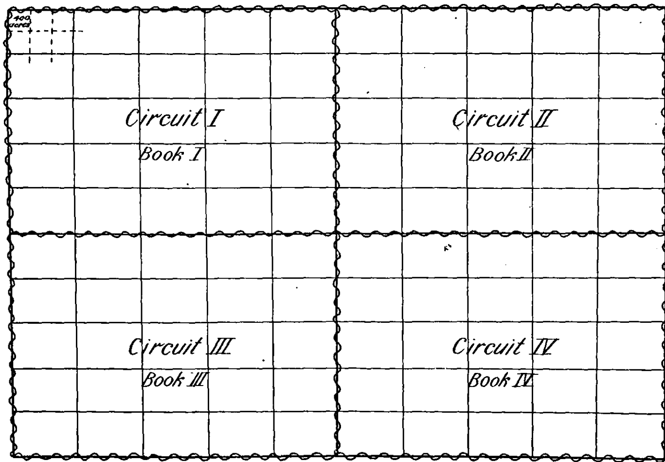
Diagram of Block showing main rectangles, levelling circuits & books Tertiary levelling to run north & south
