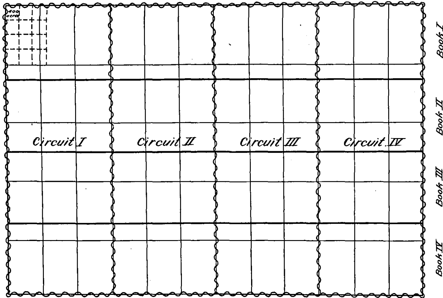
Diagram of Block showing main rectangles, levelling circuits and books, tertiary levelling to run East and West
