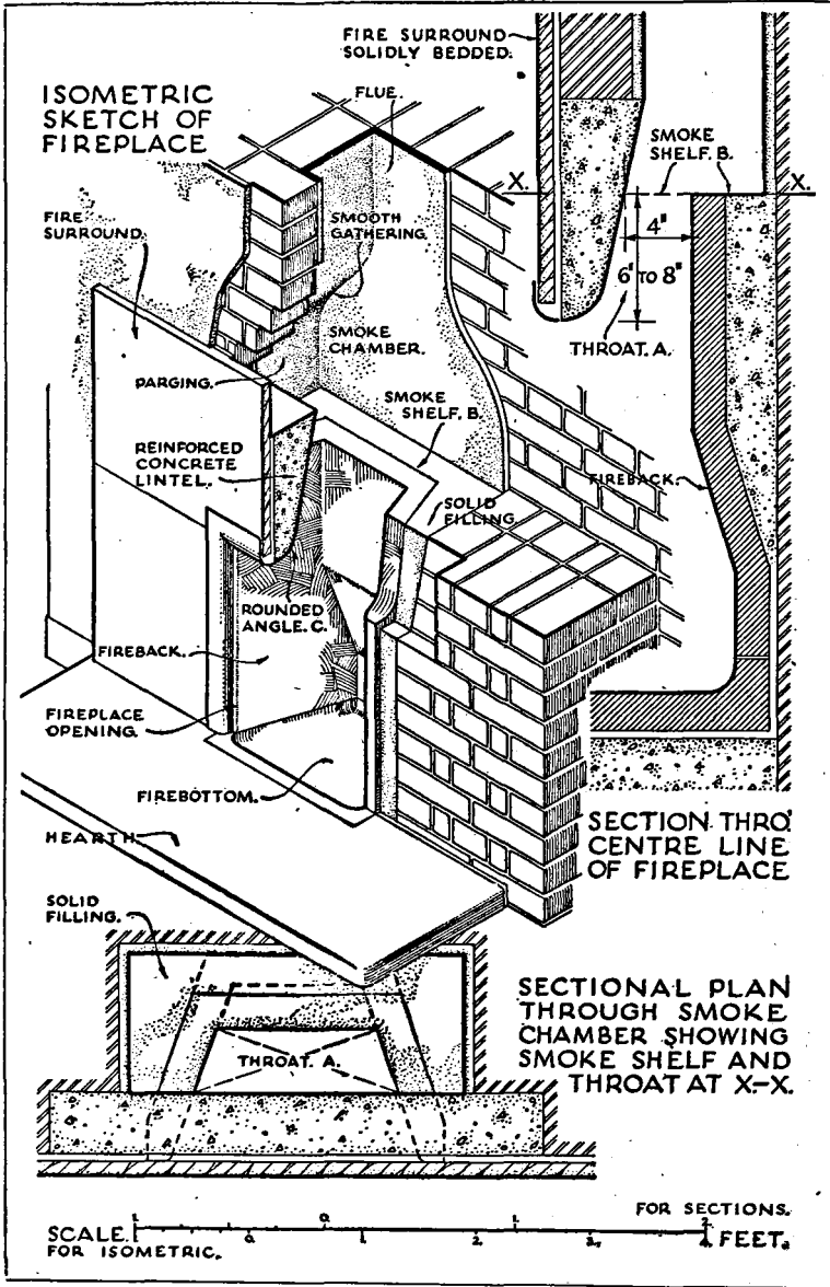
FIG. 2. RECOMMENDATIONS FOR THE DESIGN OF OPEN FIREPLACES
