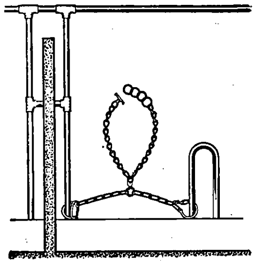
Fig. 8. Chain Tie
