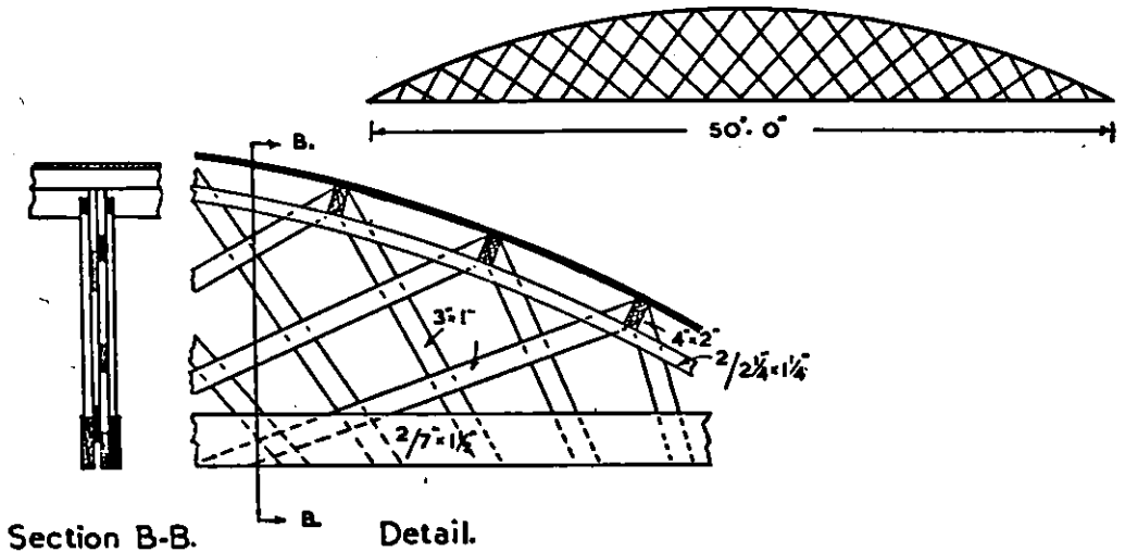
Fig. 43. Timber Truss—Belfast Type
