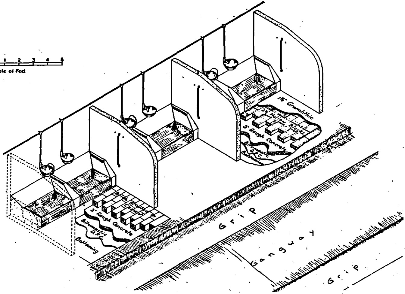
Fig. 6. Alternative Methods of Byre Floor Construction
