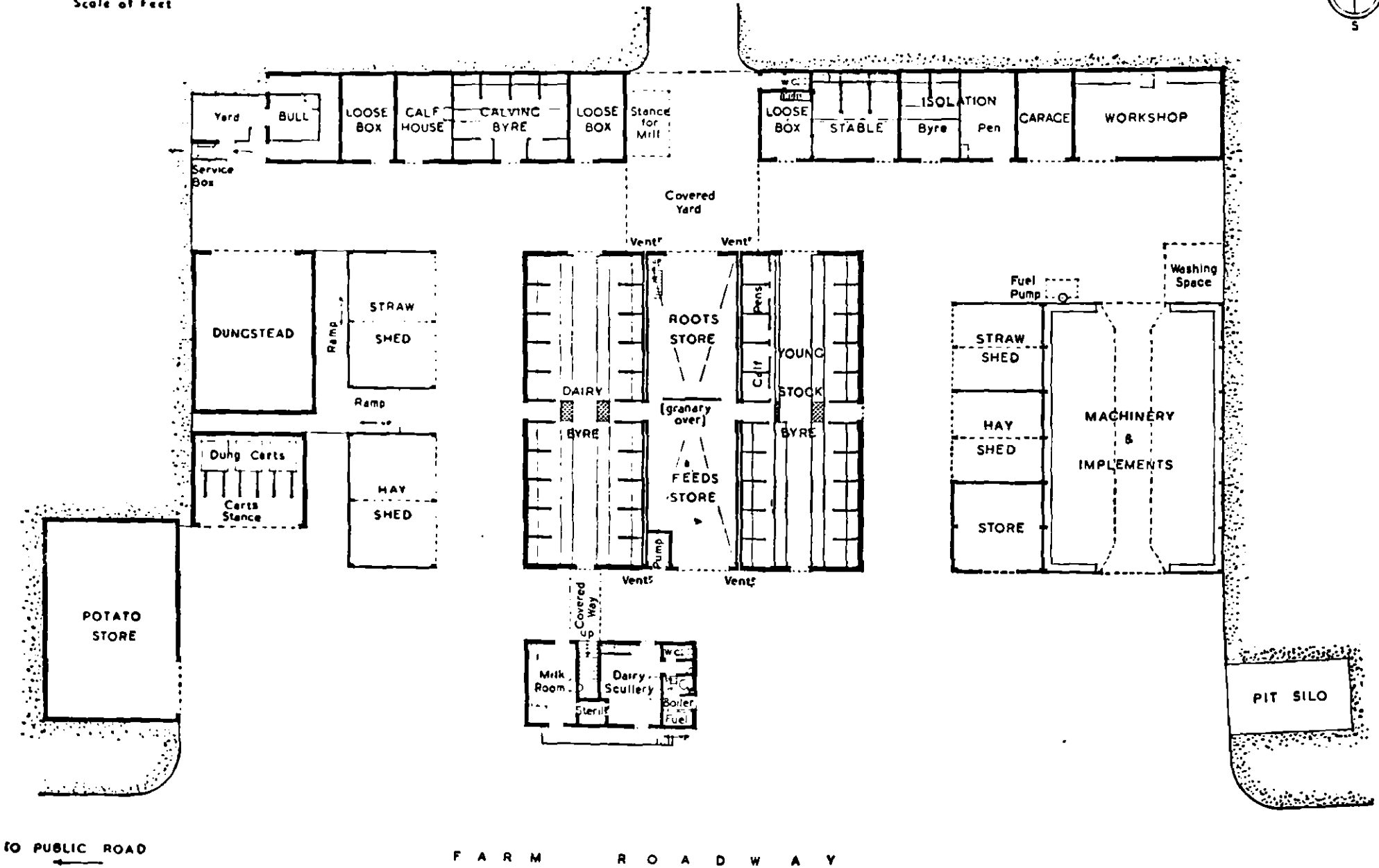
Plate 2. Plan C. Steading for Mixed Arable and Dairy Farm (Byre System) for 200 to 250 Acres (See paragraph 53)
