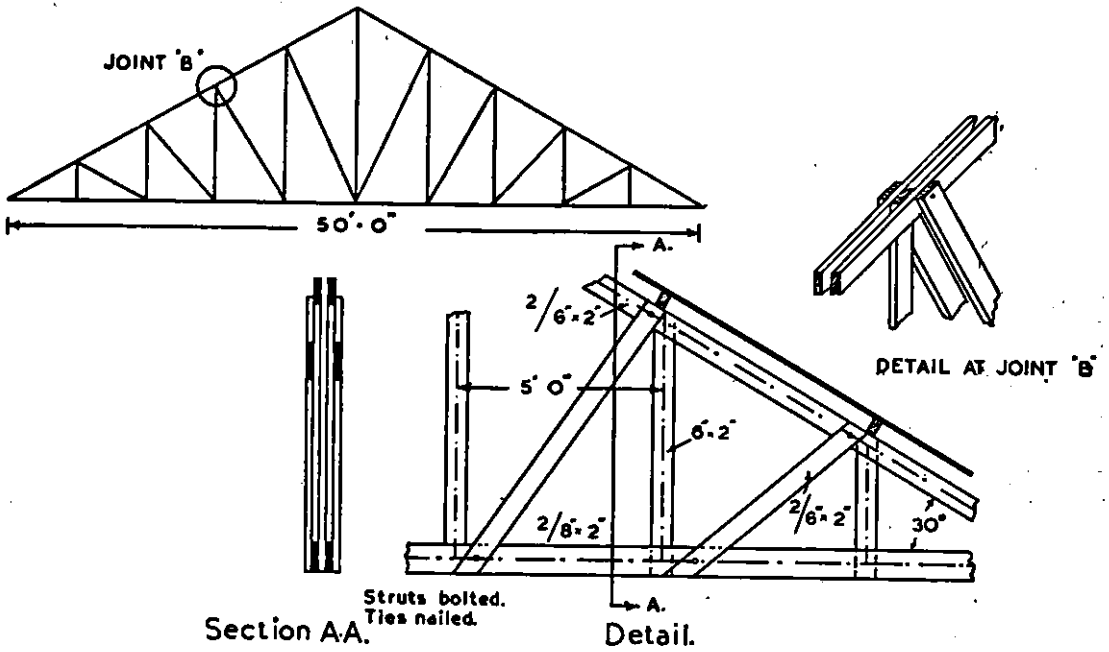
Fig. 42. Steel Truss
