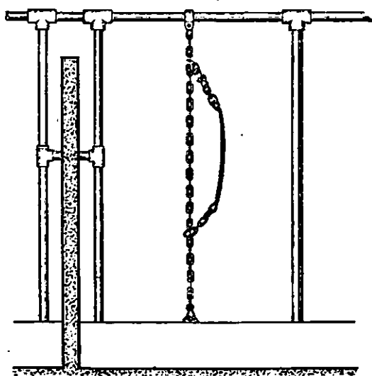
Fig. 9. Chain Tie "Dutch" Type
