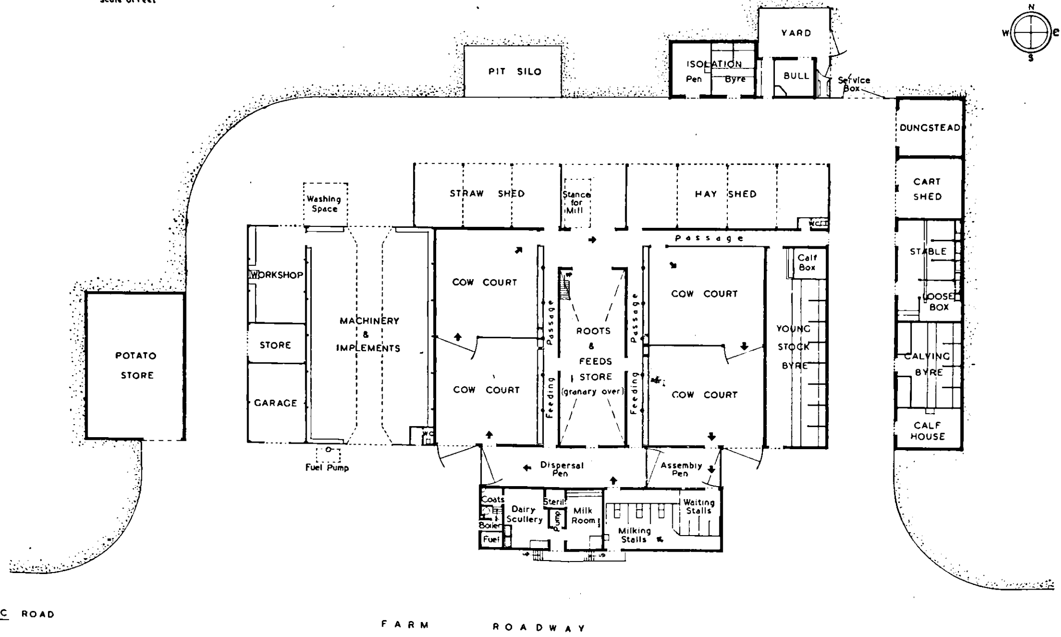
Plate 4. Plan E. Steading for Mixed Arable and Dairy Farm (Cow Court System) for 200 to 250 Acres (See paragraph 55)
