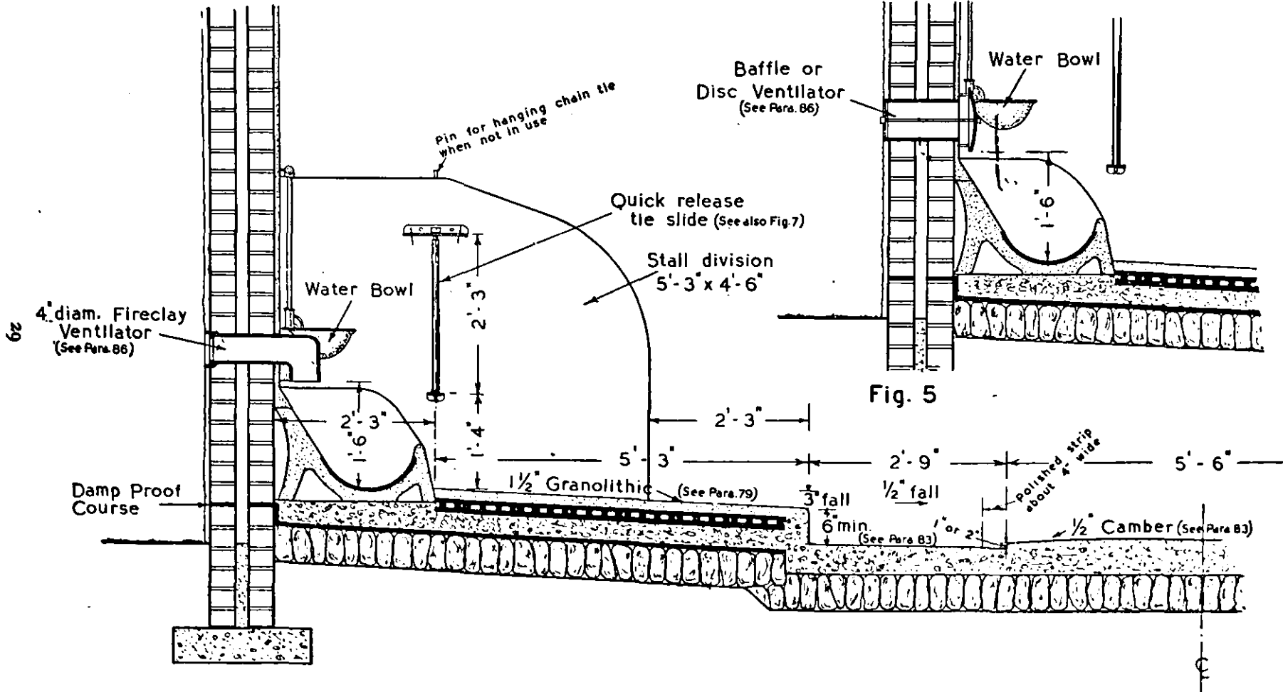
Fig. 4. Byre Details
