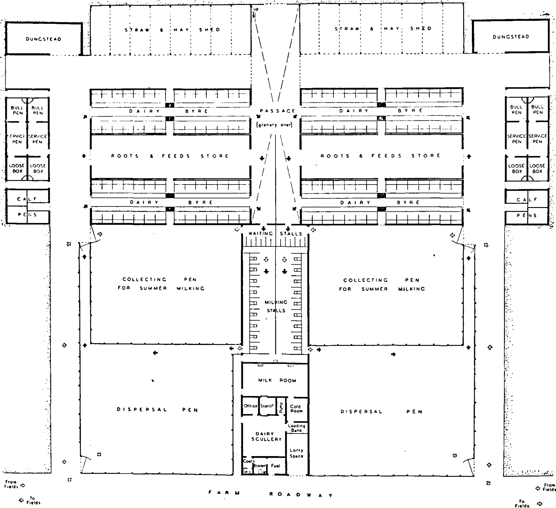
Plate 8. Plan J. Dairy Steading for 224 Cows (See paragraph 59)
