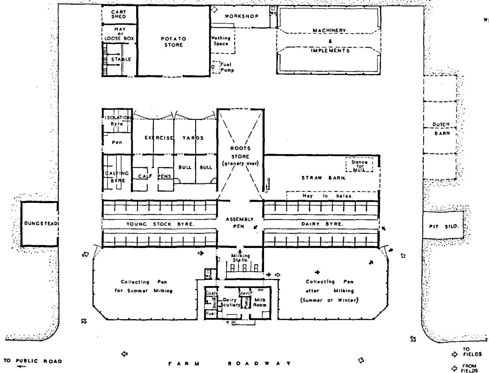
Plate 3. Plan D. Steading for Mixed Arable and Dairy Farm (Byre System) for 200 to 250 Acres (See paragraph 54)
