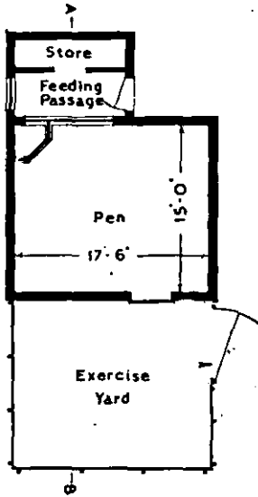
PLAN
