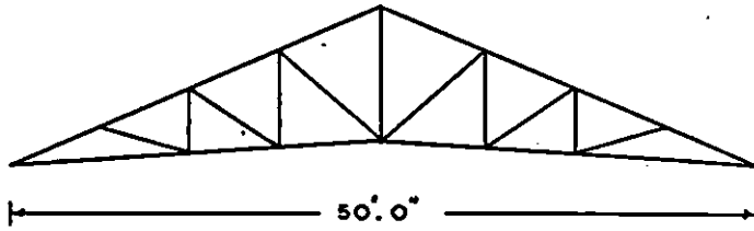
Fig. 43. Timber Truss—Belfast Type
