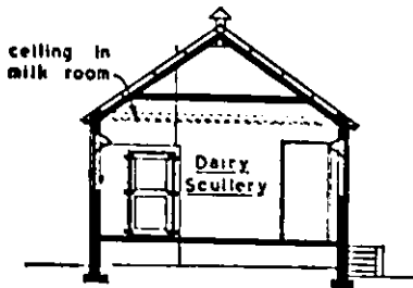
CROSS SECTION THRO' SCULLERY
