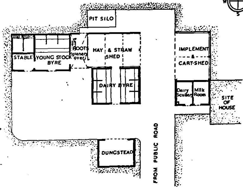
Plate 13. Plan O. Steading for Farm of 20 to 30 Acres Plan P. Steading for Farm of 20 to 30 Acres (See paragraphs 64 and 65)
