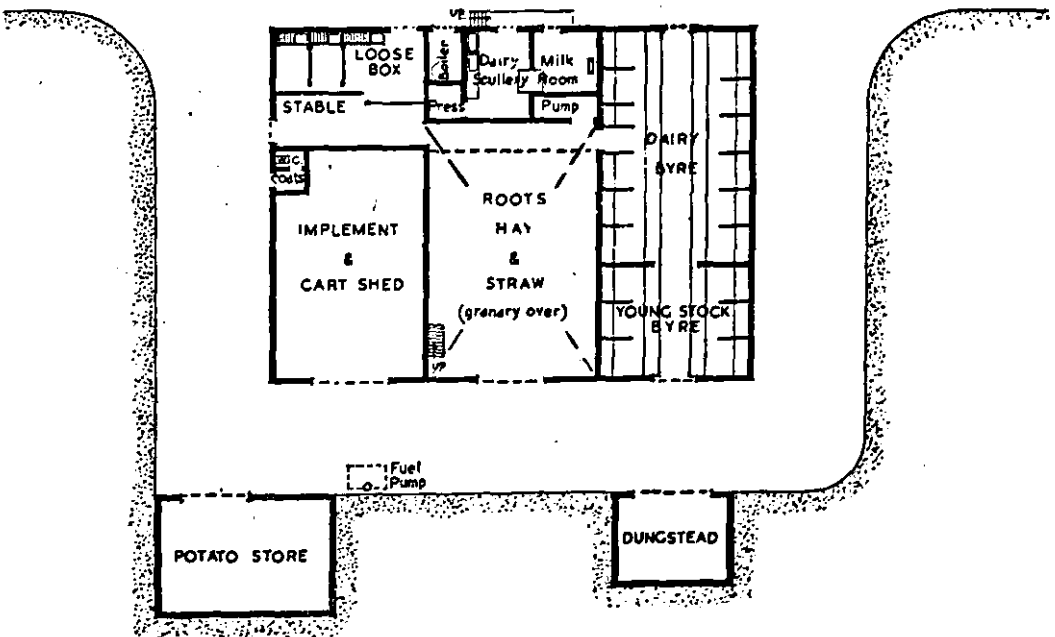
Plate 11. Plan M. Steading for Mixed Arable and Dairy Farm (Byre System) for 75 Acres (See paragraph 62)
