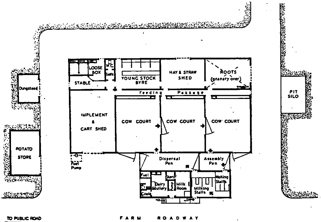
Plate 12. Plan N. Steading for Mixed Arable and Dairy Farm (Cow Court System) for 75 Acres (See paragraph 63)
