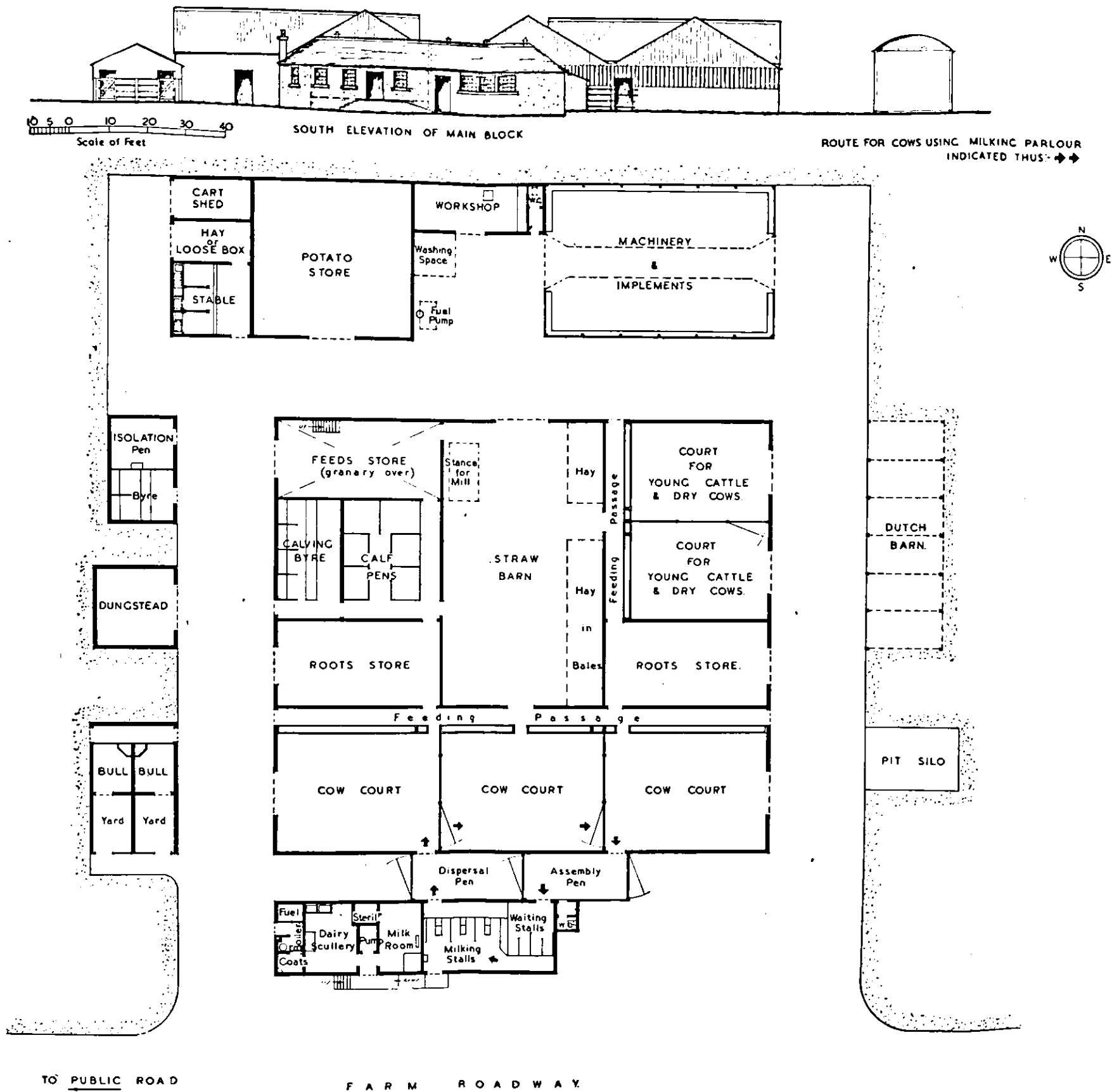
Plate 7. Plan H. Steading for Mixed Arable and Dairy Farm (Cow Court System) for 200 to 250 Acres
