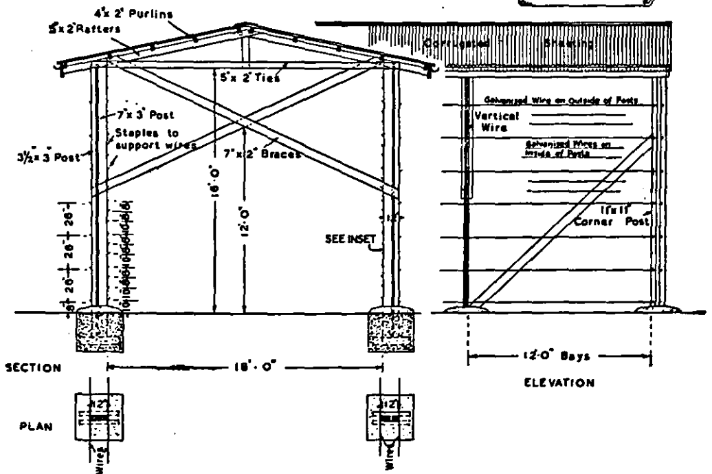
Fig 38. Dual Purpose Shed
