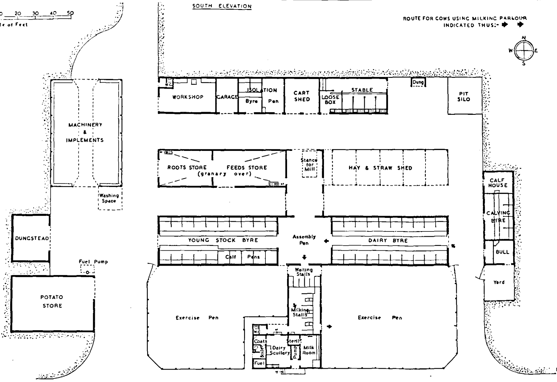
ALTERNATIVE SCHEME FOR BUCKET SYSTEM OF MECHANICAL MILKING
