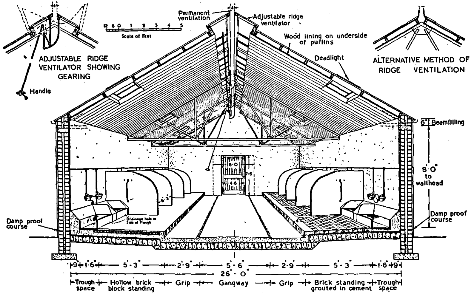
Fig. 1. Double Dairy-Cow Byre (Interior Perspective)
