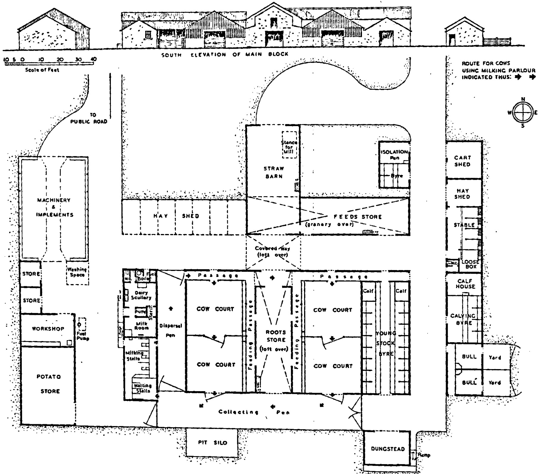
Plate 6. Plan G. Steading for Mixed Arable and Dairy Farm (Cow Court System) for 200 to 250 Acres (See paragraph 57)
