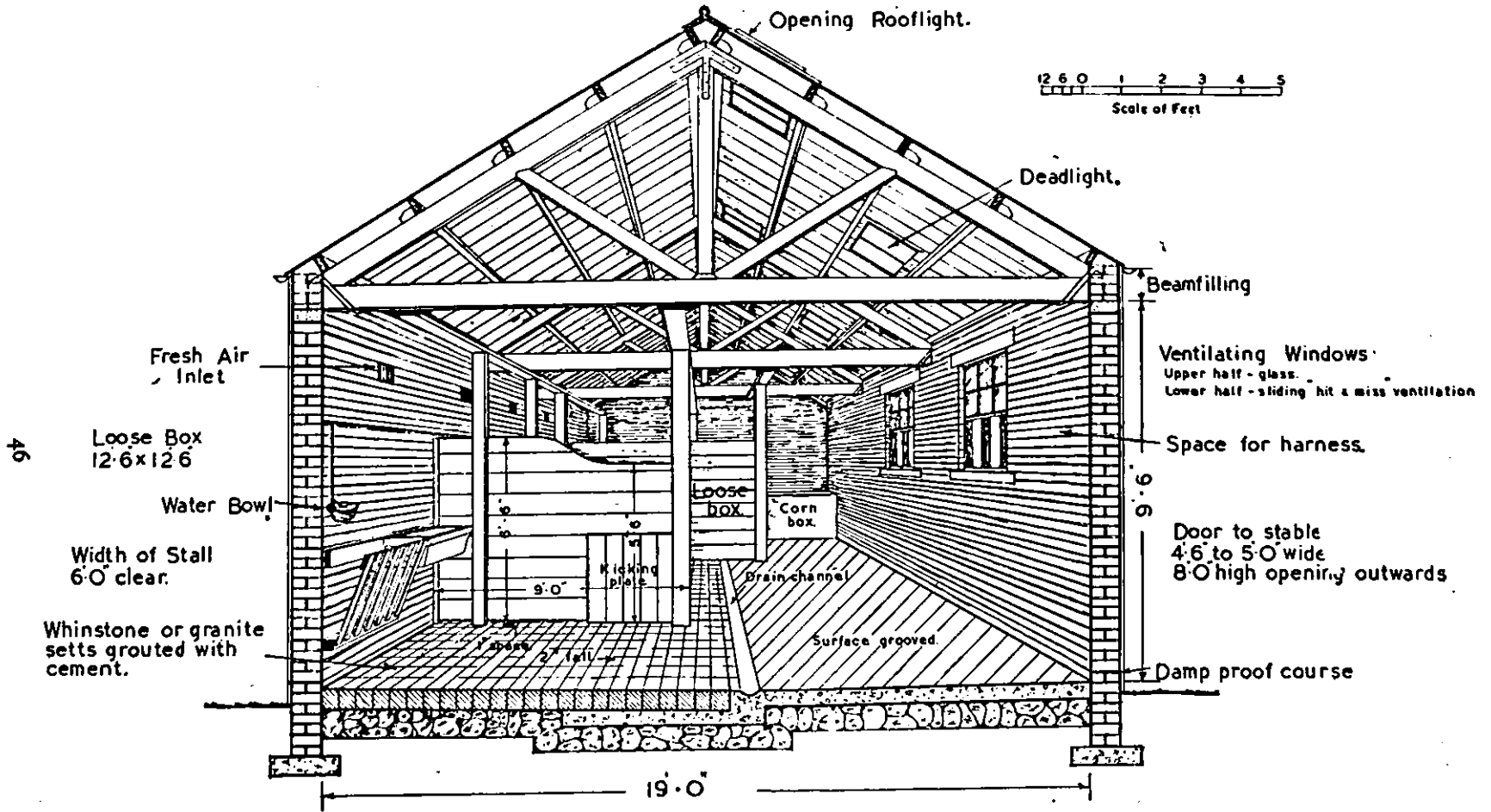
Fig. 25. Stable (Interior Perspective)
