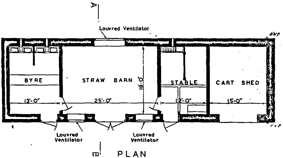
Plate 14. Plan Q. Highland Croft Steading for 5 to 10 Acres (See paragraph 66)
