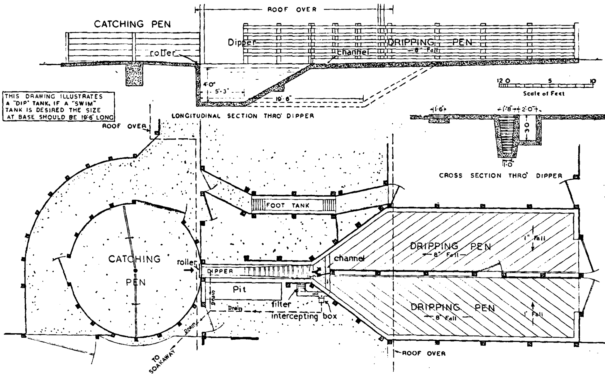
Fig. 40. Design for Sheep-Dipper
