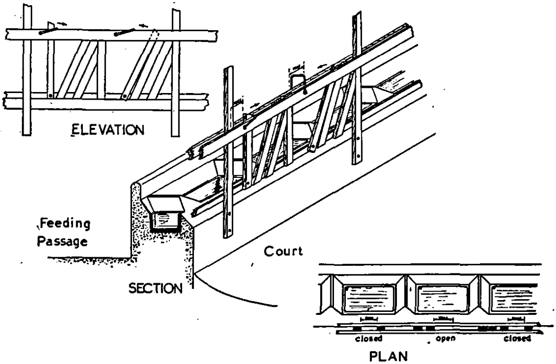
Fig. 13. Timber Yoke for Cow Courts
