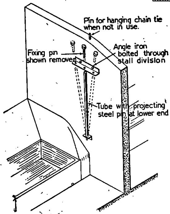
Fig. 7. Quick-Release Tie Slide
