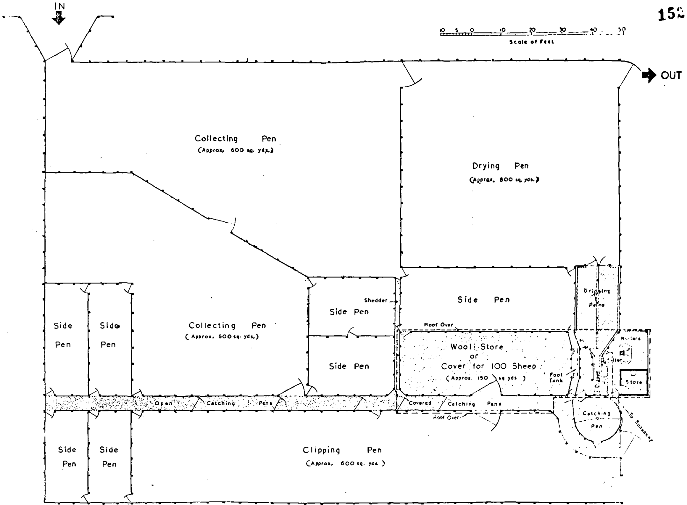
Fig. 39. Plan of Sheep-Dipper and Collecting Pens or Fanks
