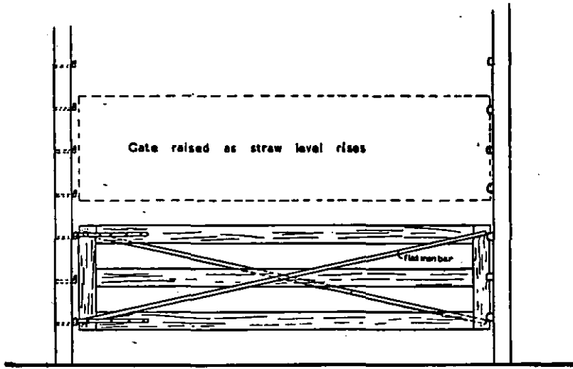
Fig. 12. Lifting Gate for Cow Courts .
