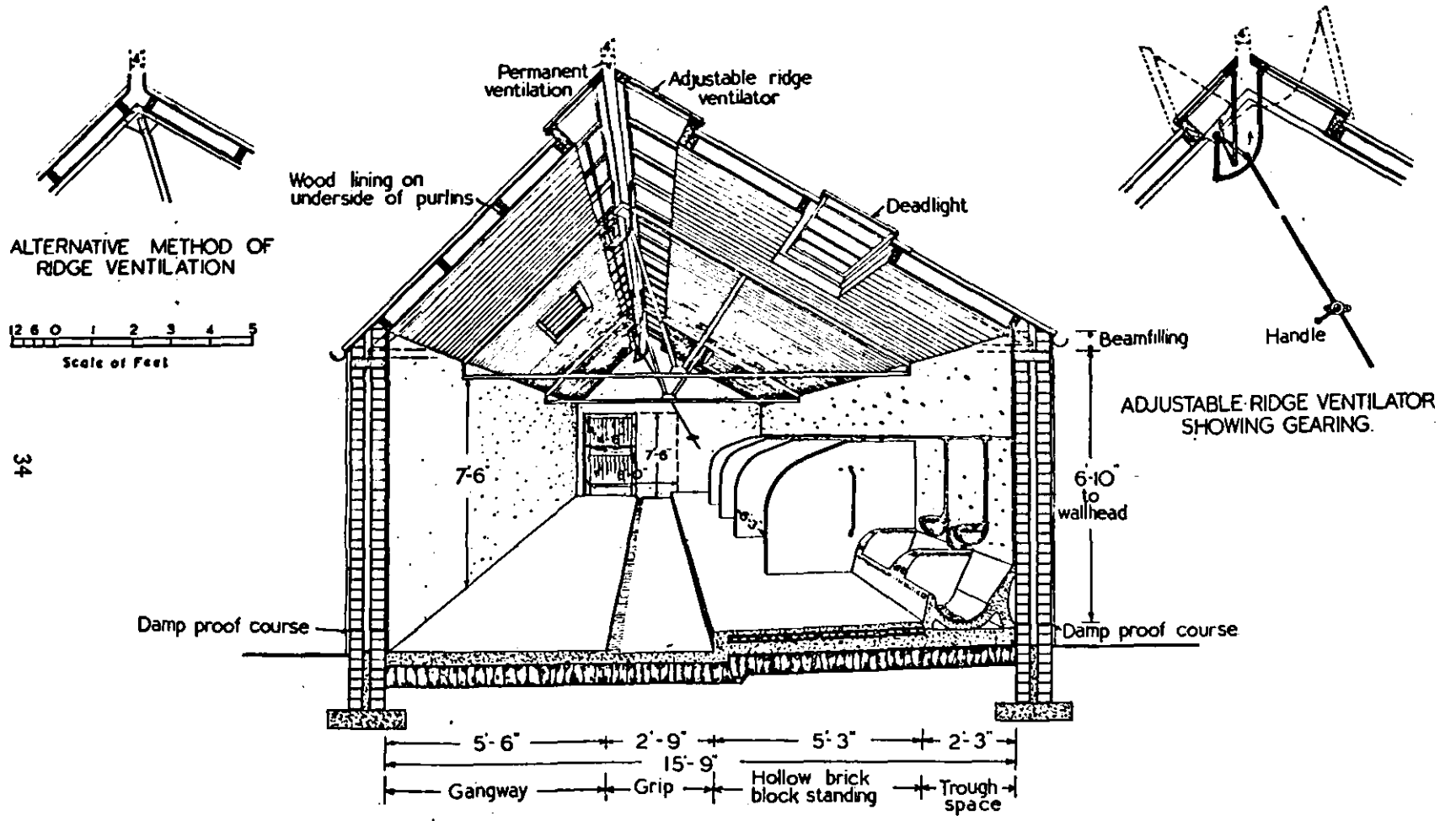
Fig. 11. Single Dairy-Cow Byre (Interior Perspective)
