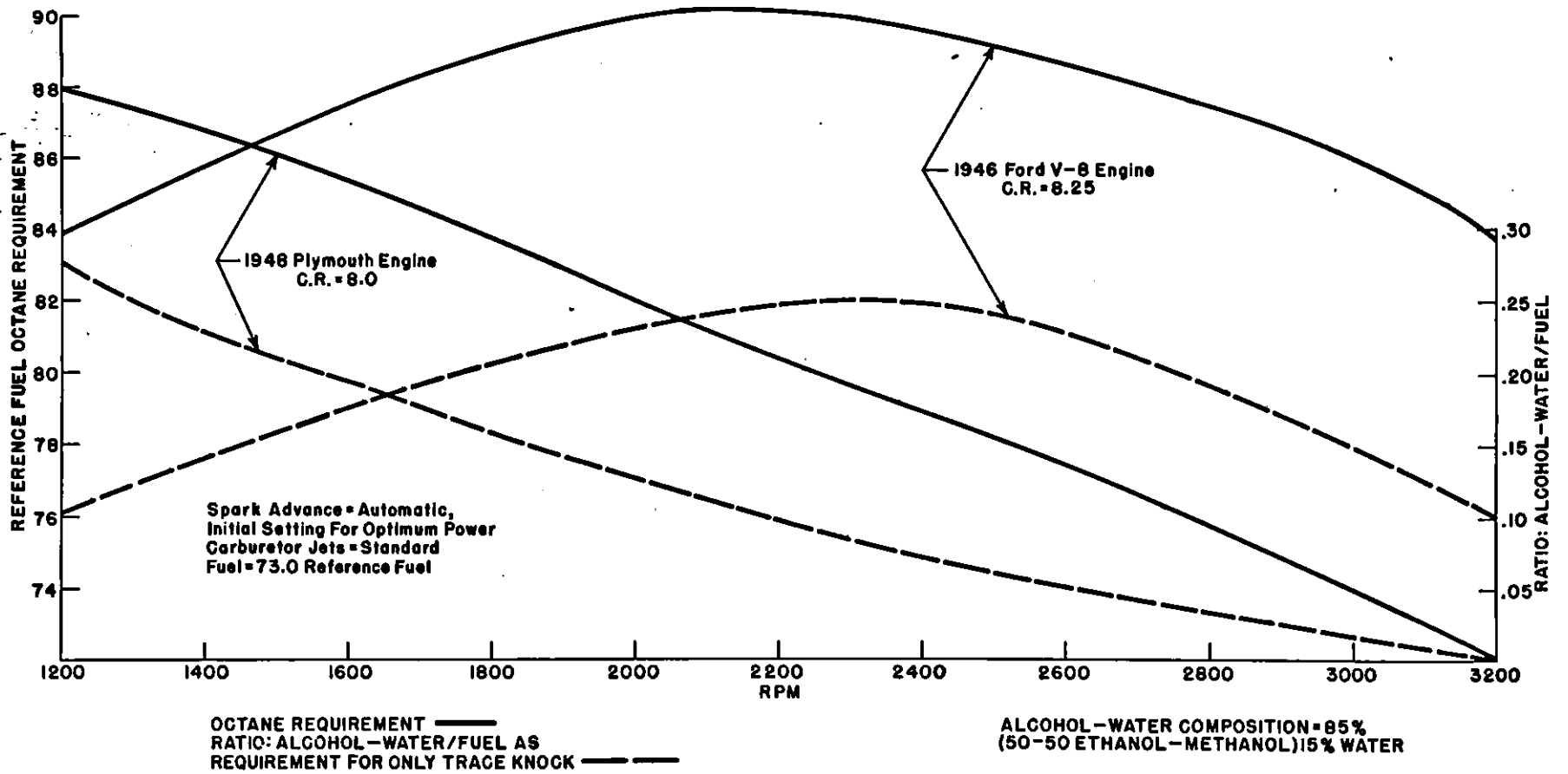
Figure 4.--Injection rate and octane requirement as related to engine speed at full throttle for two L-head, high compression engines.
