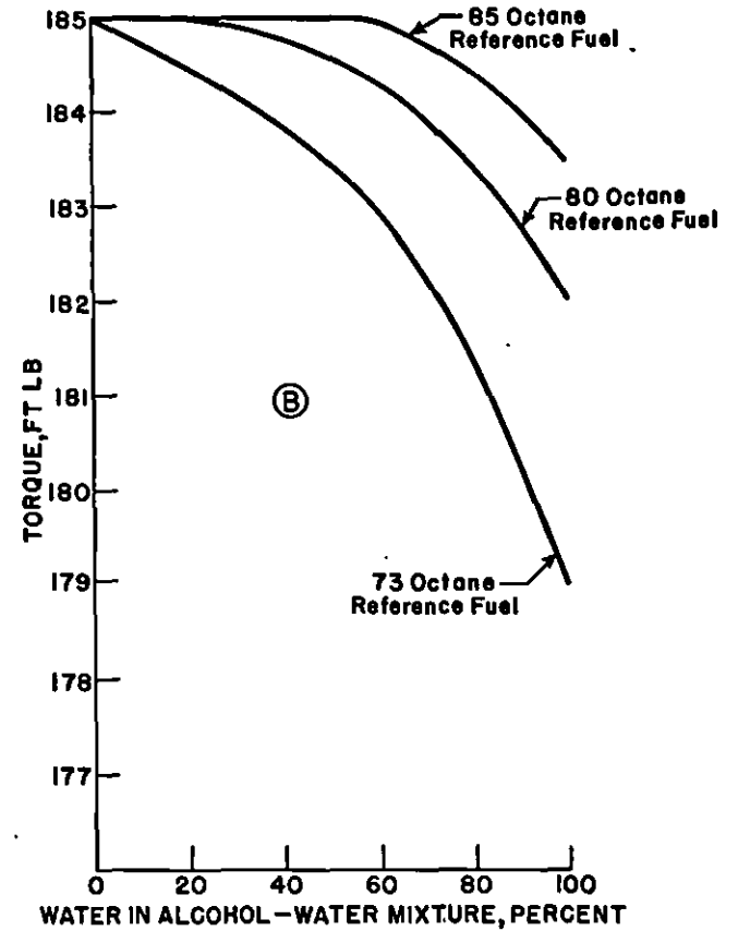
Figure 3.--Effect of the percentage of water in the ethanol-water mixture on the amount of injection required for only trace knock and on engine torque.
