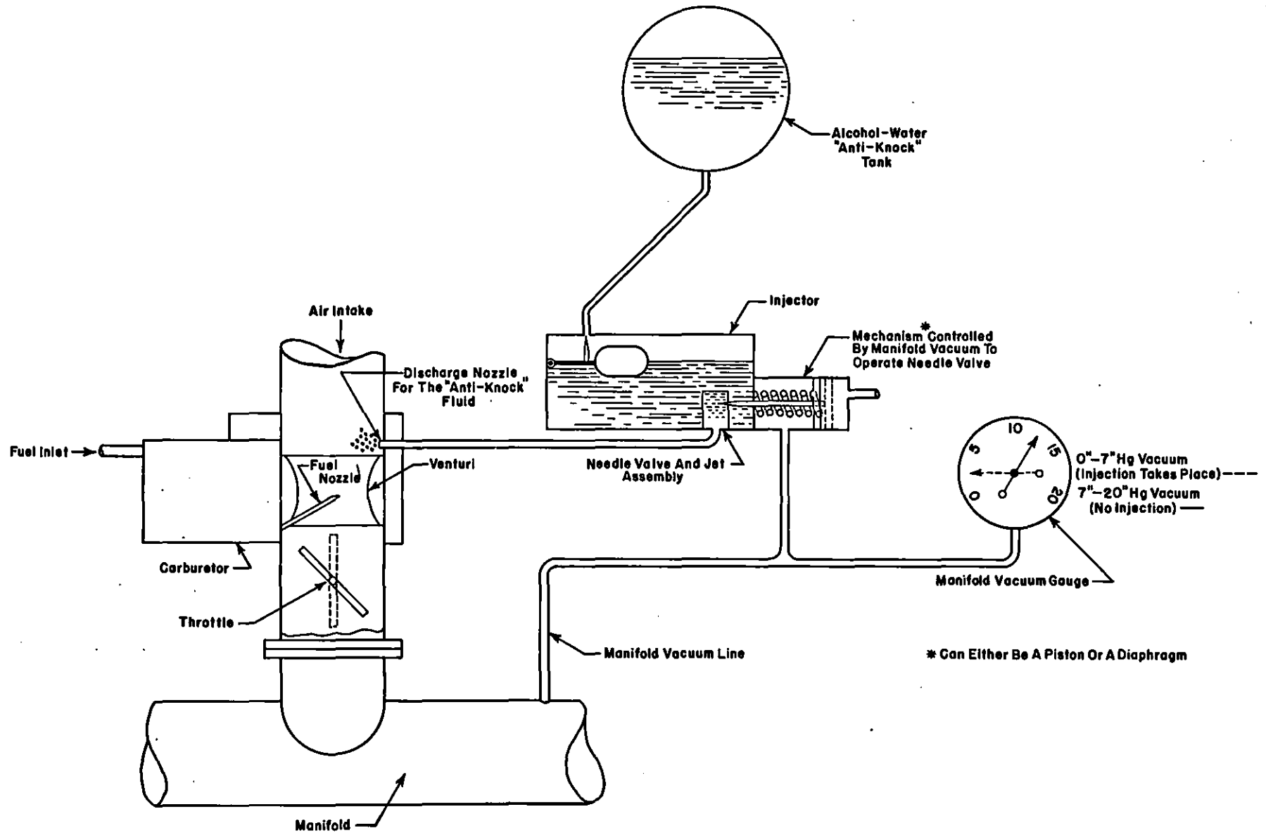
Figure 2.--Diagram of injector principle.
