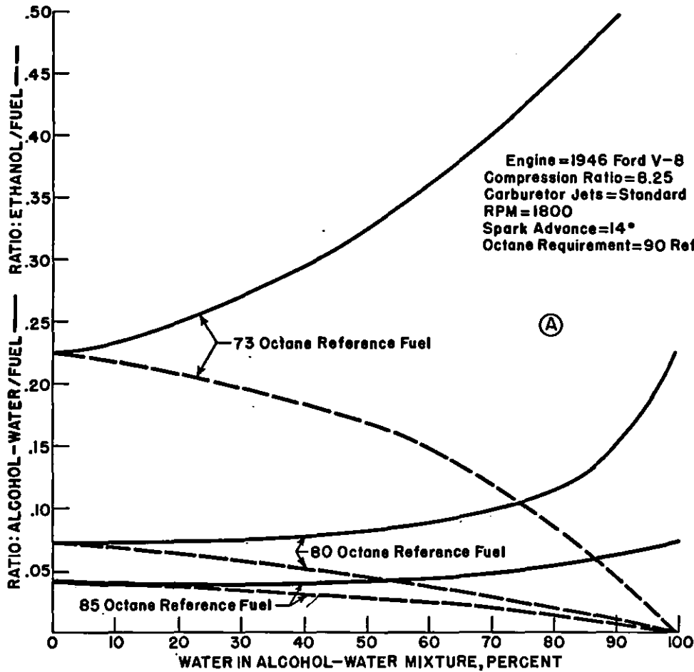
Figure 3.--Effect of the percentage of water in the ethanol-water mixture on the amount of injection required for only trace knock and on engine torque.
