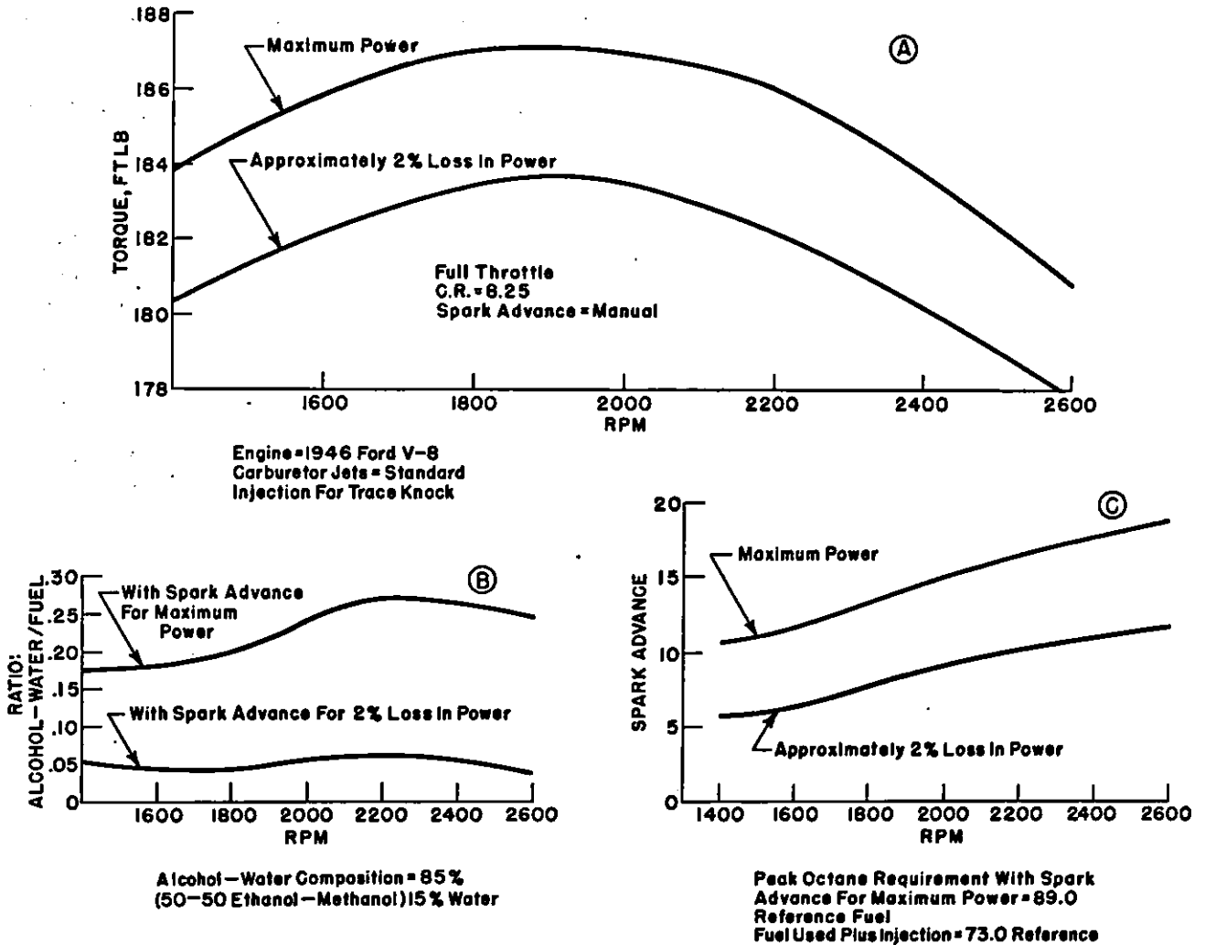
Figure 10.--Effect of spark advance on power and injection rate required.
