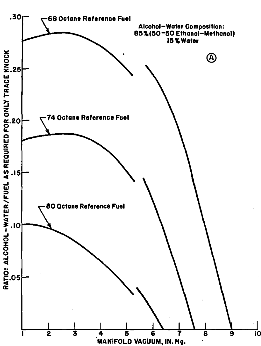
Figure 5.--How manifold vacuum for injection "cut-out" and injection rate required for only trace knock vary with the octane number of the fuel used.
