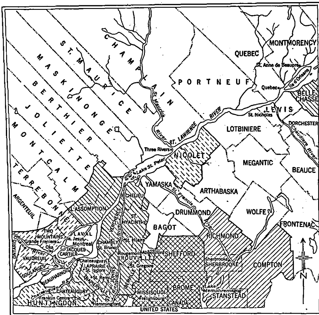
INDEX MAP OF CENTRAL QUEBEC SHOWING LOCATION OF SURVEYED AREAS
