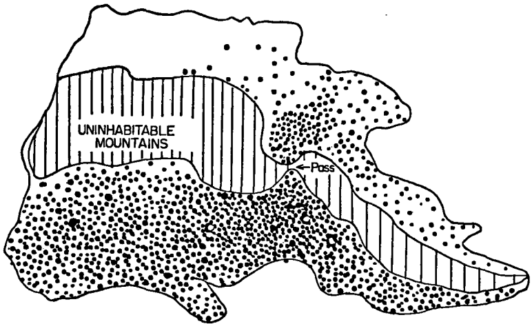
FIGURE 24. Diagram showing the situation after a gene has crossed a barrier between two isolated populations. The degree of stippling roughly proportional to gene density on the two sides of the barrier.
