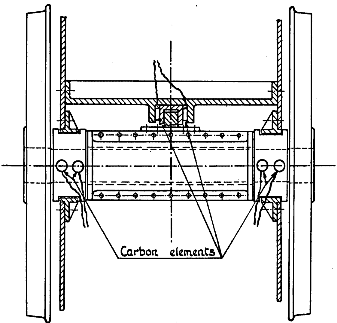
Plan view of pair of coupled wheels.
