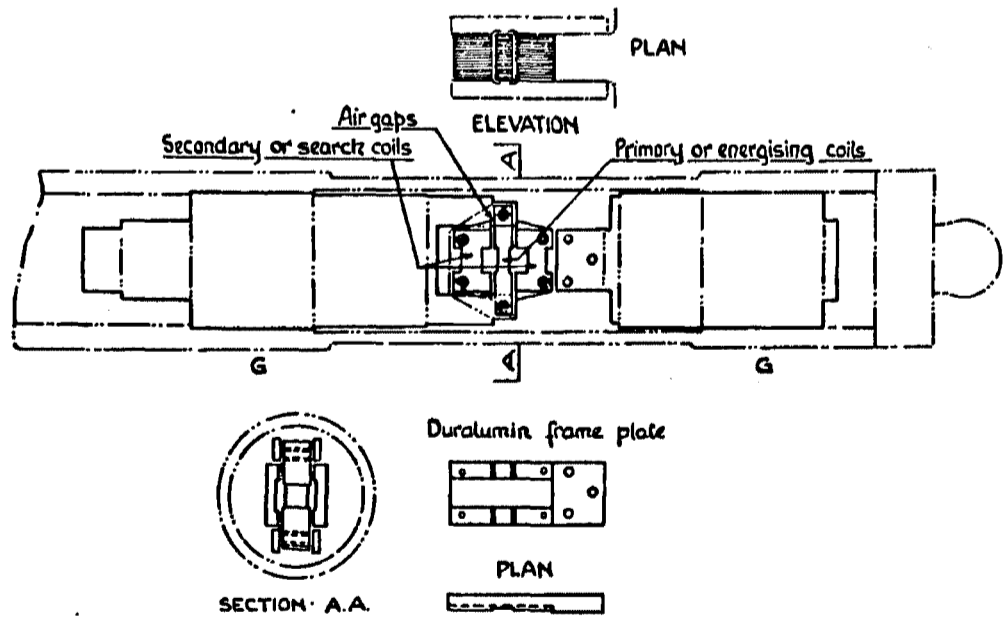
ELECTROMAGNETIC DETECTOR FOR WEIGHBARS.
