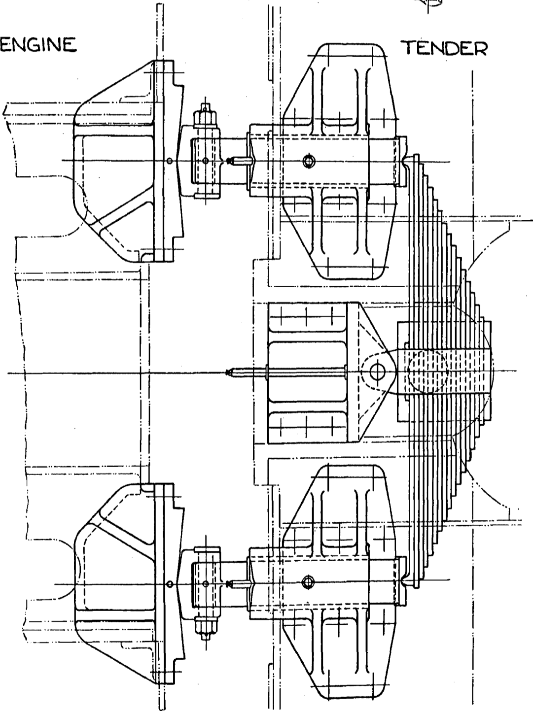
ARRANGEMENT OF GERMAN TYPE INTERMEDIATE BUFFING GEAR.
