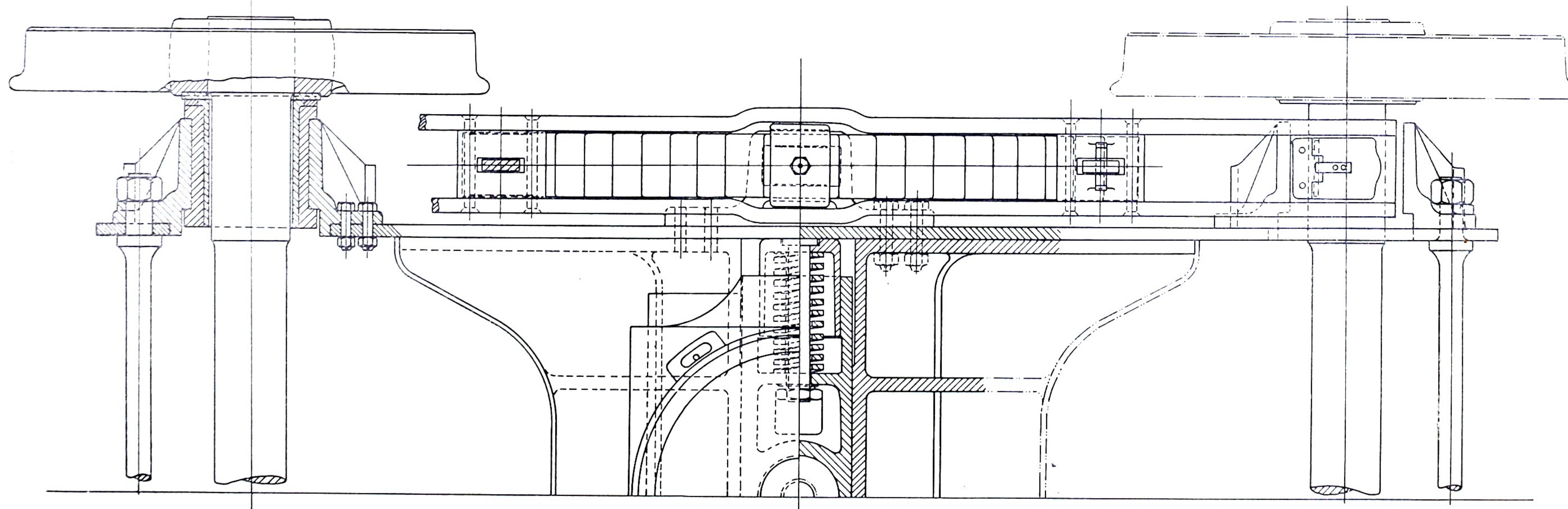
X CLASS PACIFIC BOGIE AS ORIGINALLY DESIGNED.
