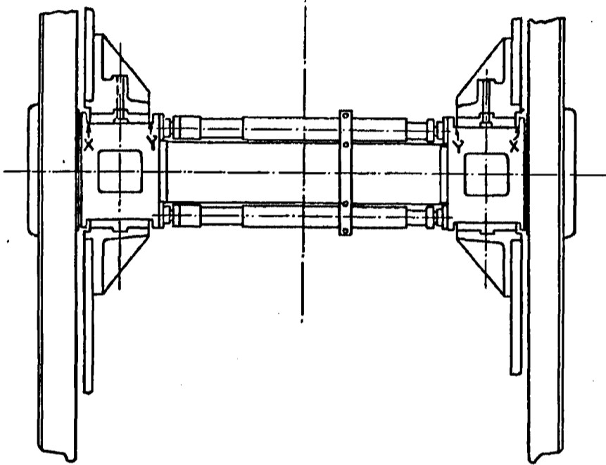
ASSEMBLY OF WEIGHBARS BETWEEN AXLEBOXES.
