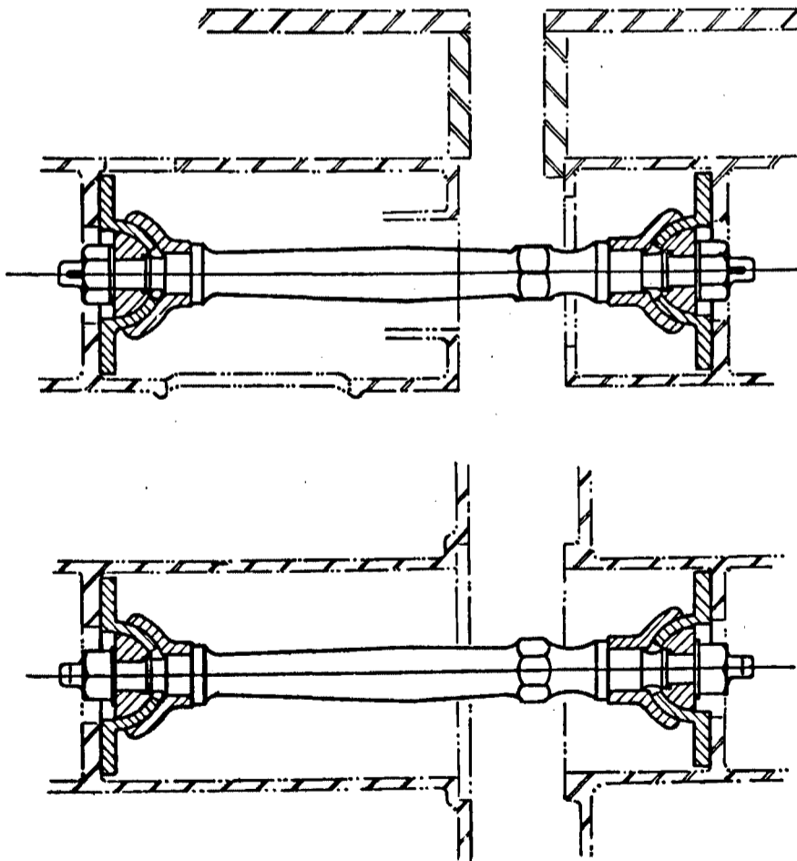
GOODALL TYPE DRAWGEAR.
