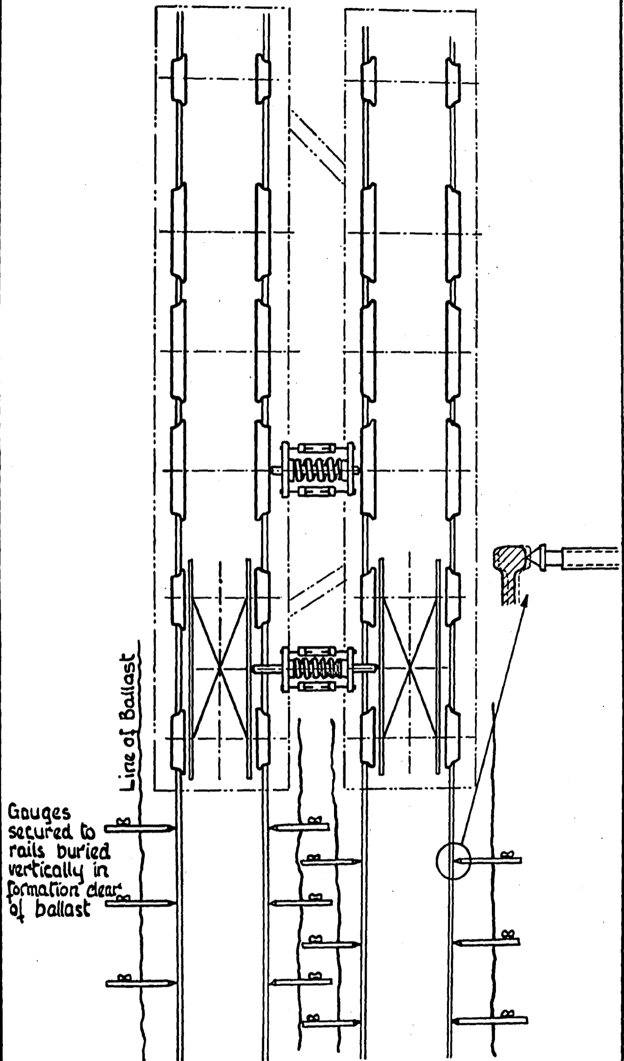
DIAGRAM SHEWING ENGINES COUPLED TOGETHER FOR TRACK TESTS
