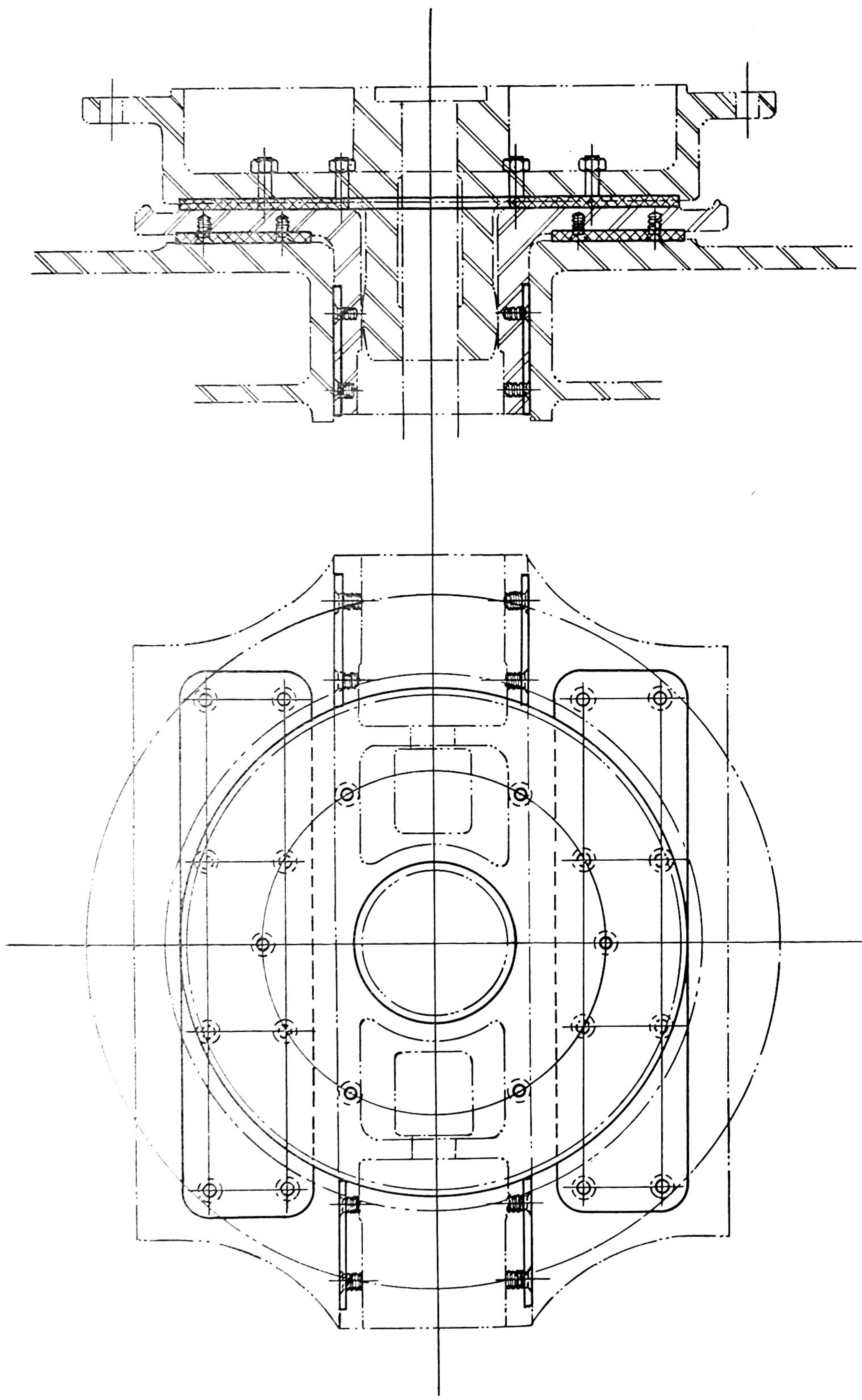
POSITION OF FRICTION LINERS ON BOGIE.
