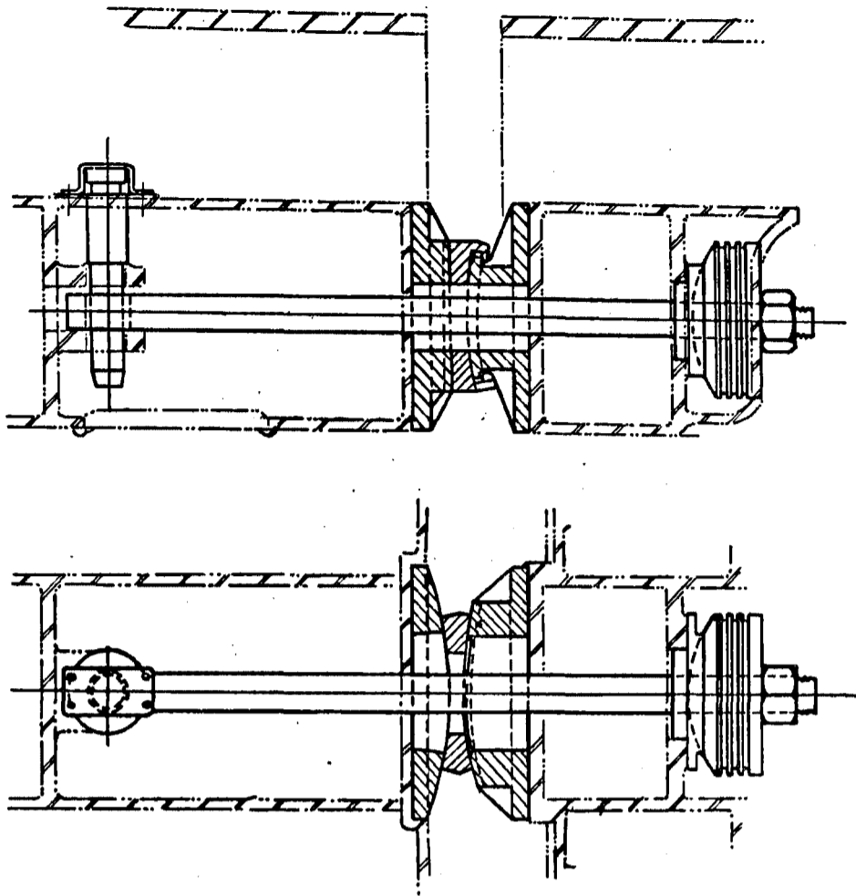
AMERICAN TYPE DRAWGEAR.
