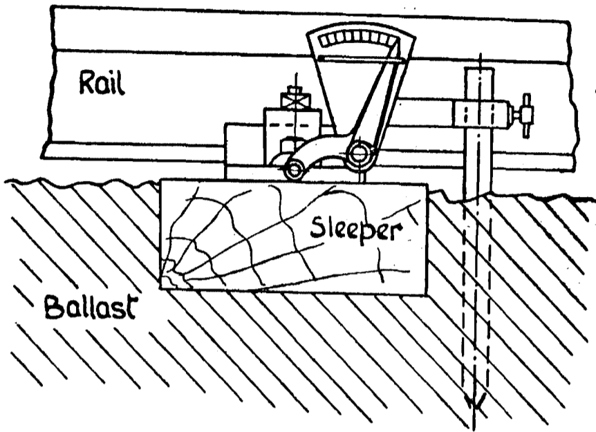
Position of pointers before passage of train.
