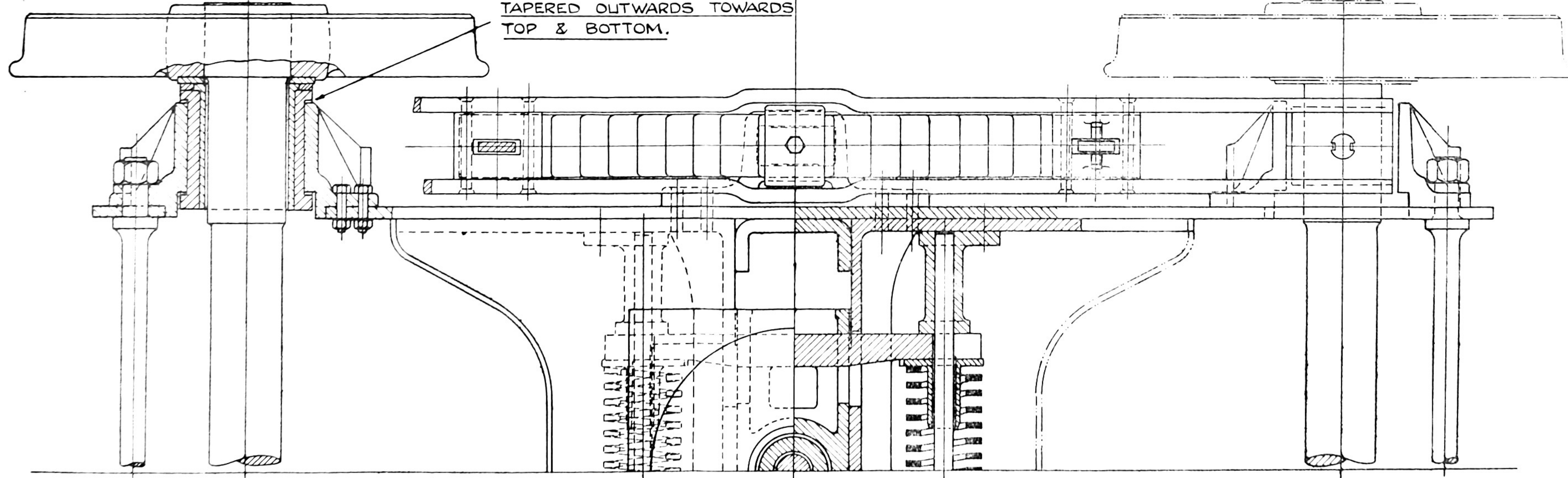
X CLASS PACIFIC BOGIE SUGGESTED ARRANGEMENT.
