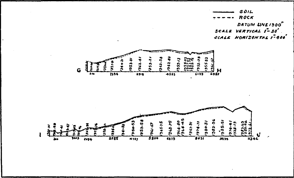
Sections through Village Area. (Continuation of lines G-H and I-J, see Plate II.)
