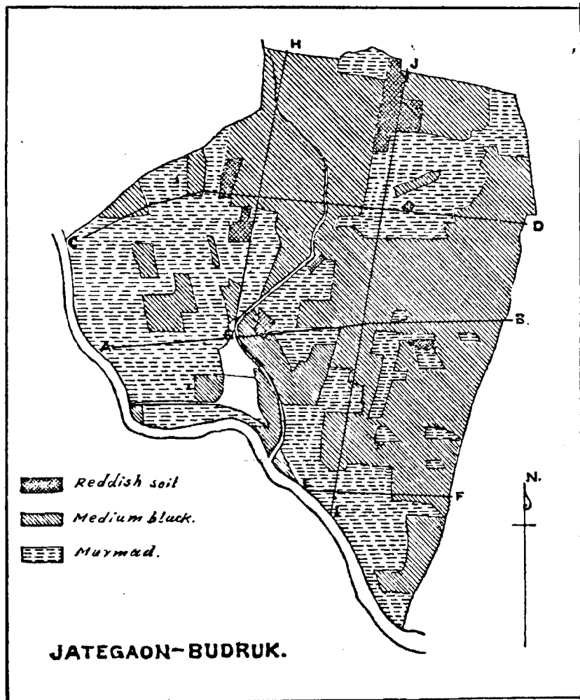
Soil Map of the Village of Jategaon Budruk. (Sections on lines AB, CD, EF, GH, and IJ, are shown on Plates III. and IV.)
