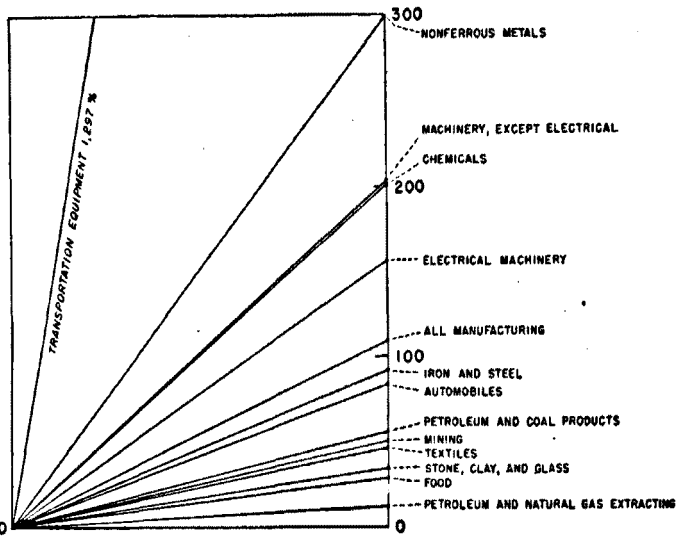
CHART 15.—Percentage increase in electricity requirements of manufacturing and extracting industries. (Source: U. S. Department of Commerce.)
