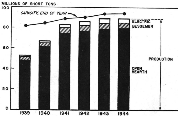
CHART 21.—Steel capacity and production (ingots and steel for castings). (Source: American Iron and Steel Institute.)
