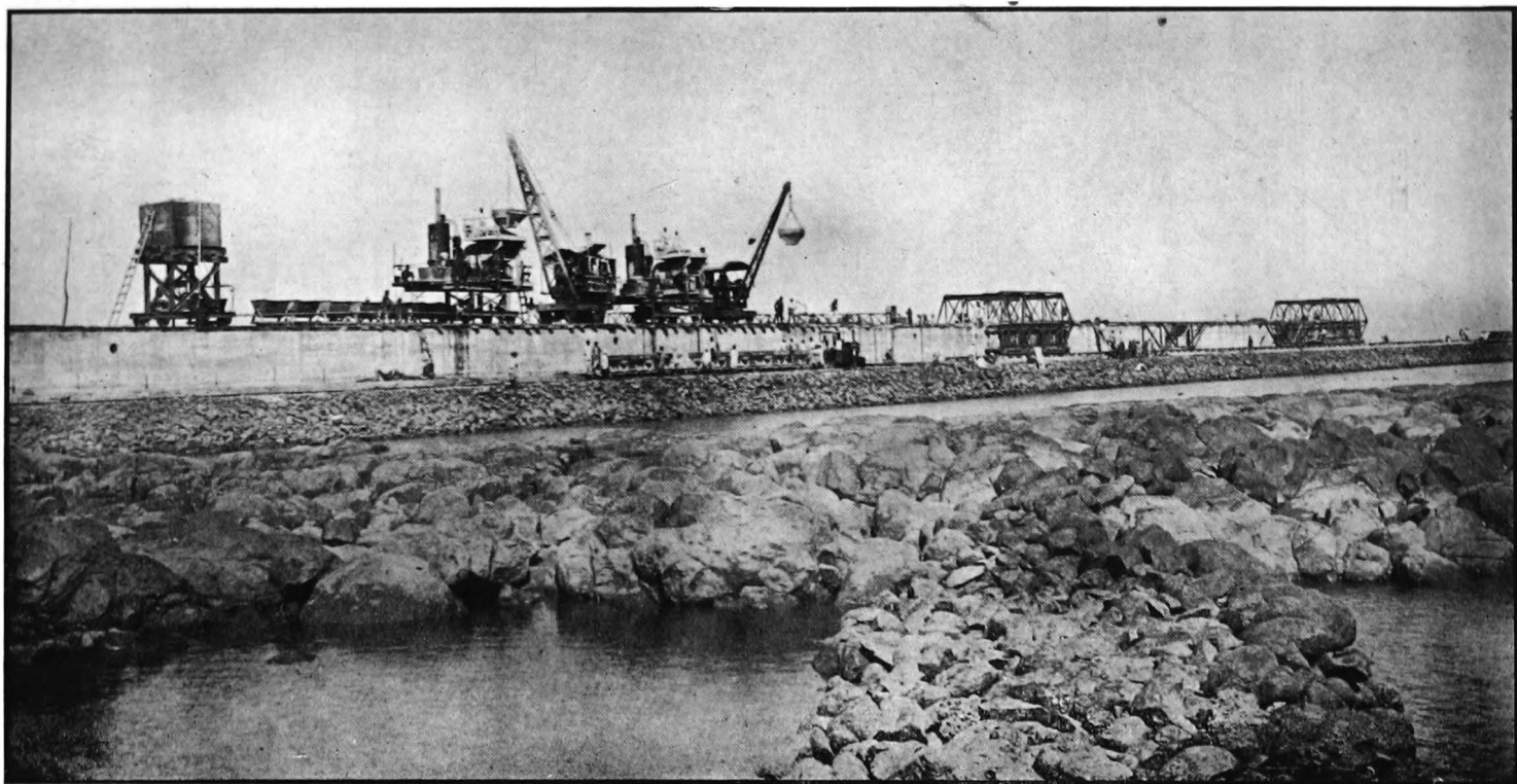
M. C. Wall Chainage 3,200. Concreting Plant including Steel forms. Date 18th October 1923.
