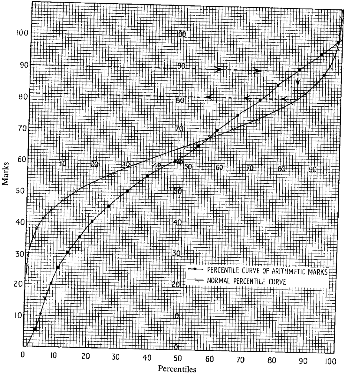
Percentile Curve of 1,379 Arithmetic Marks and Normal Percentile Curve
