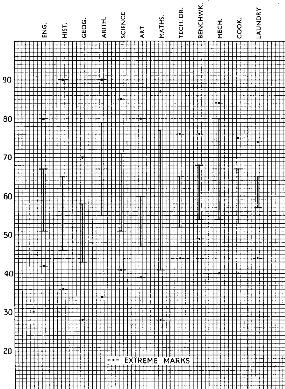
Illustration of Differences in Mean and Scatter of School Marks
