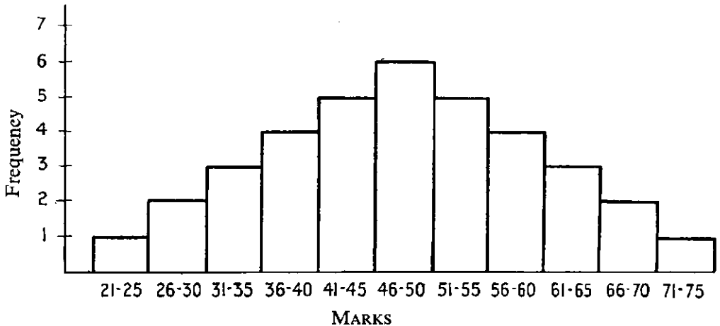
Diagrammatic Representation of Frequency Distribution A
