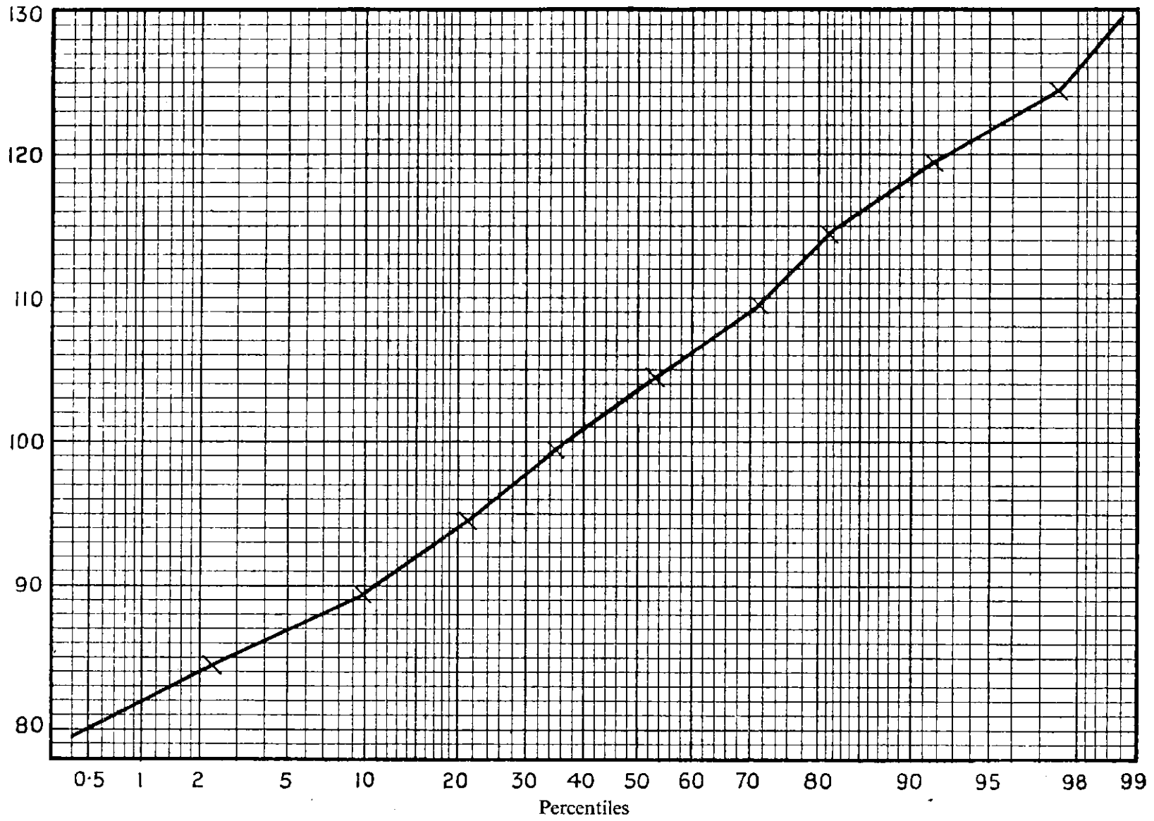
FIG. X Graph of Percentile Distribution of IQs on Per mille Paper
