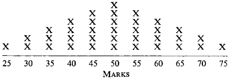
FIG. I Distribution of Marks in Test A
