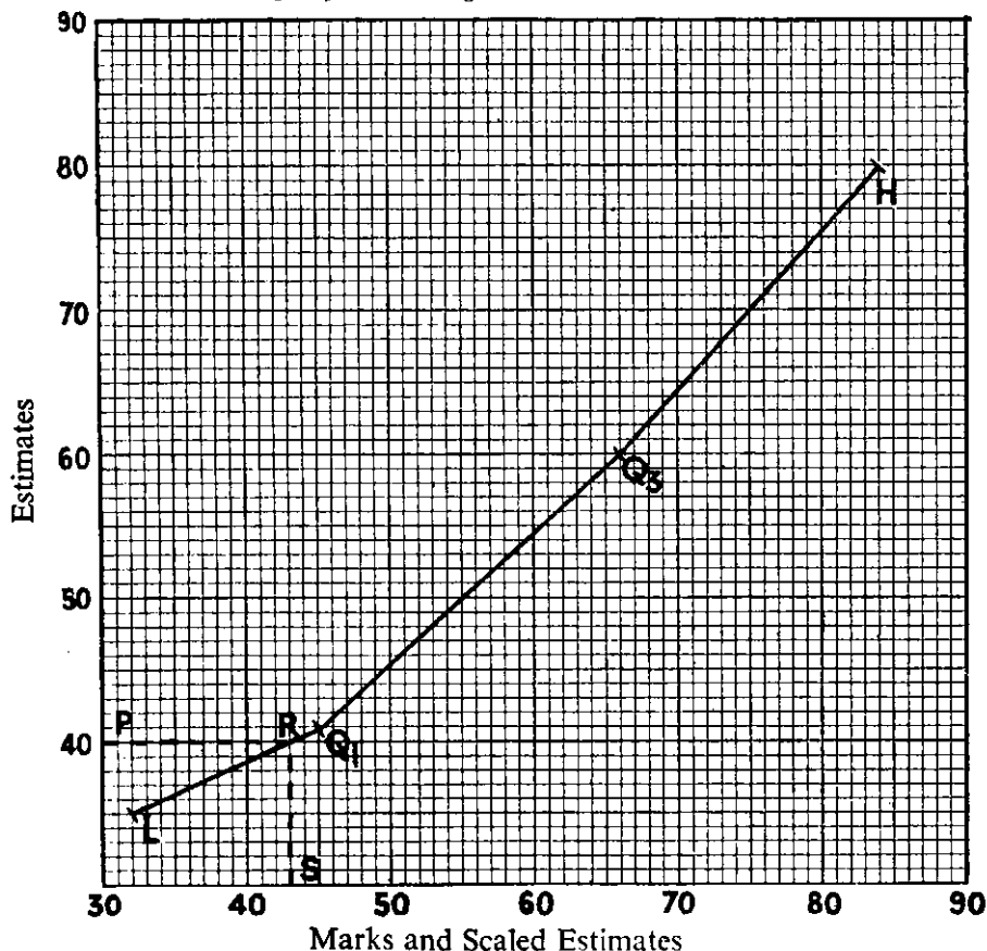
Graph for Scaling Teachers' Estimates
