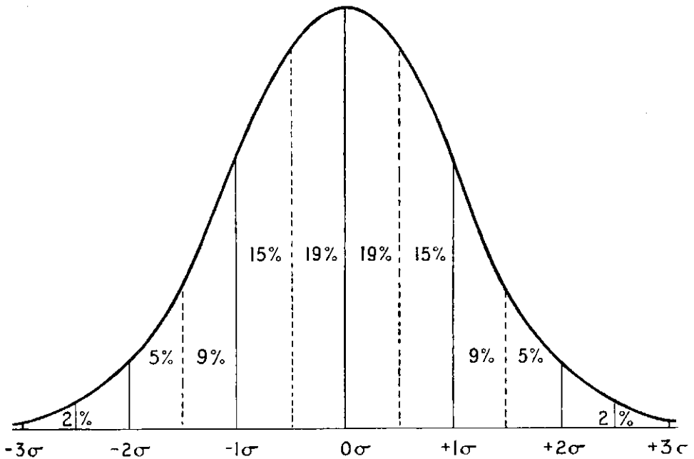
FIG. VII Area under Normal Curve
