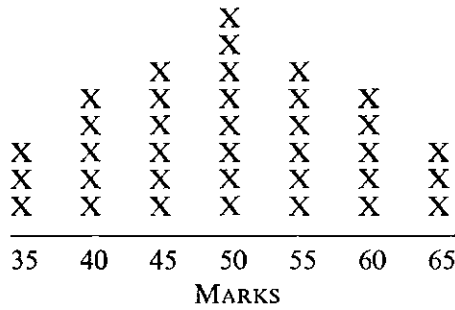
FIG. III Distribution of Marks in Test C
