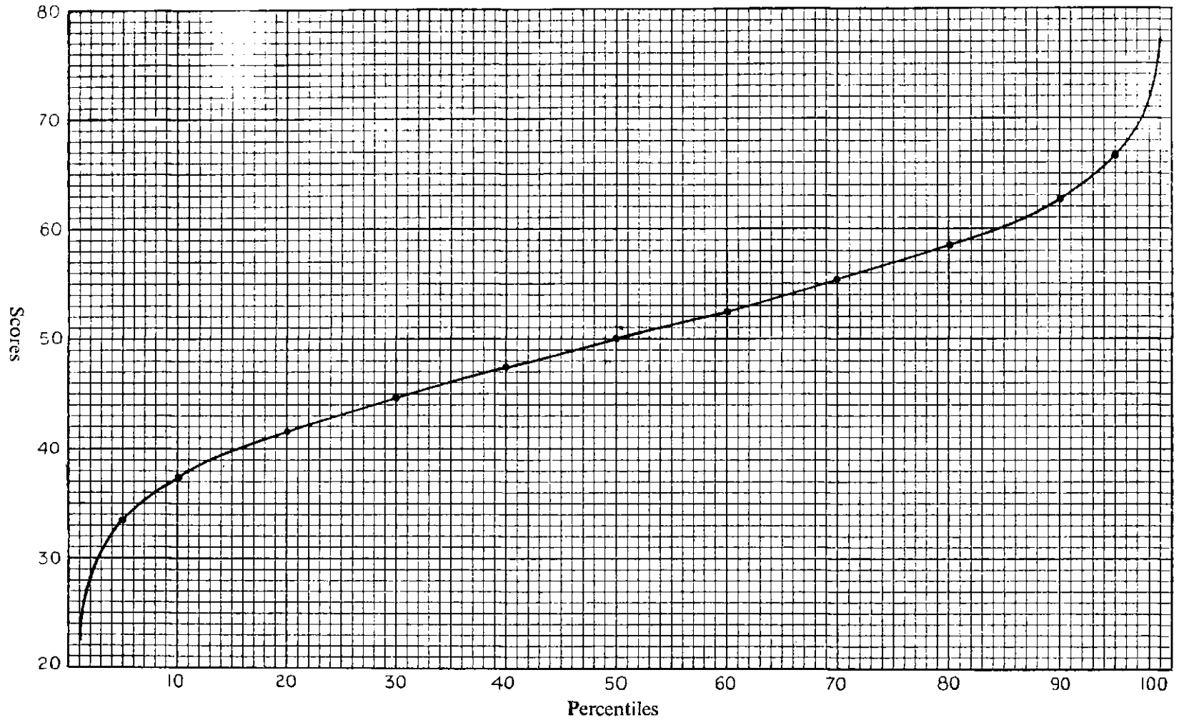
FIG. VIII Percentile Curve or Ogive
