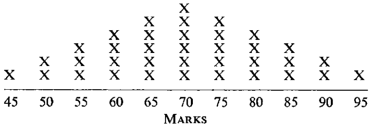
FIG. II Distribution of Marks in Test B
