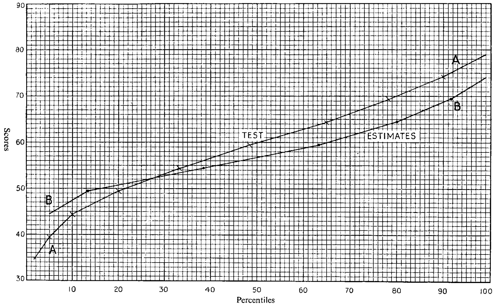
Graph for Scaling Teachers' Estimates in English in School E
