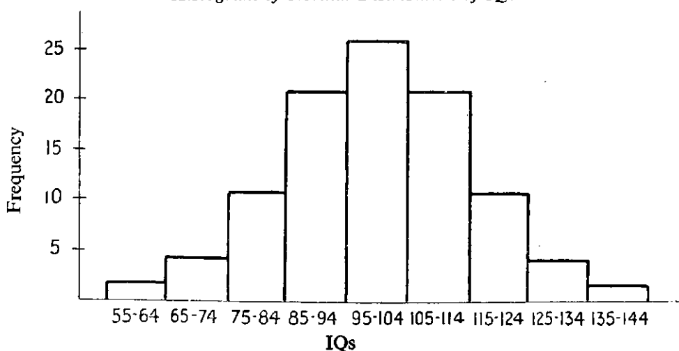
FIG. VI Histogram of Normal Distribution of IQs
