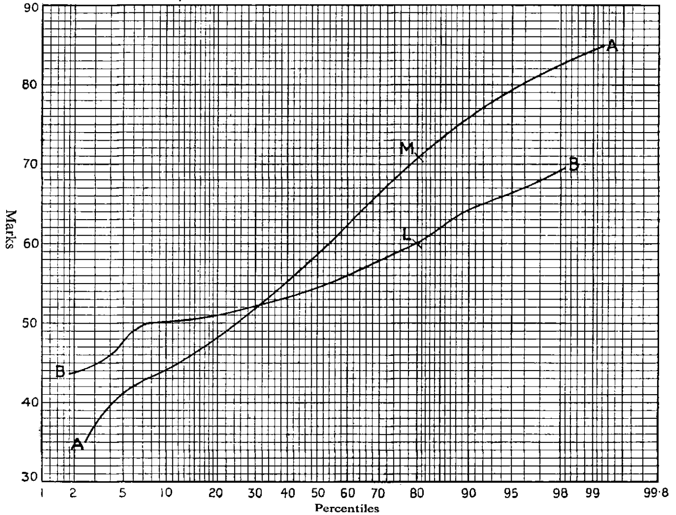
FIG. XX Graphs for Scaling Leaving Certificate Teachers' Estimates
