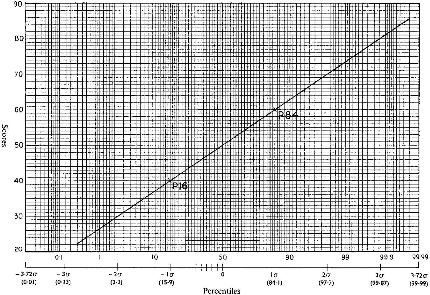
FIG. IX Percentile Curve on Per mille Paper
