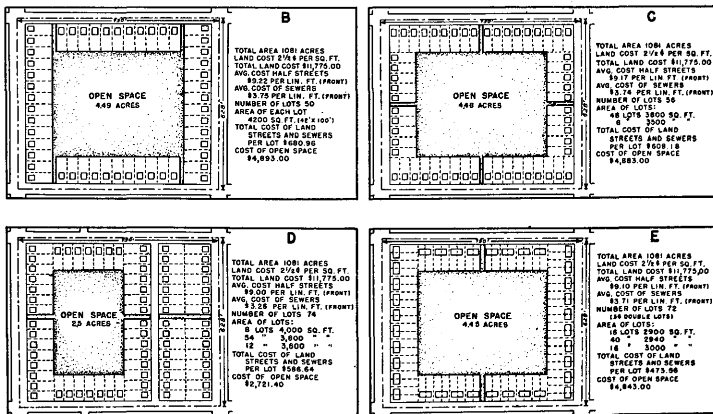
FIGURE 11.—Four ways of replatting a given city area.
