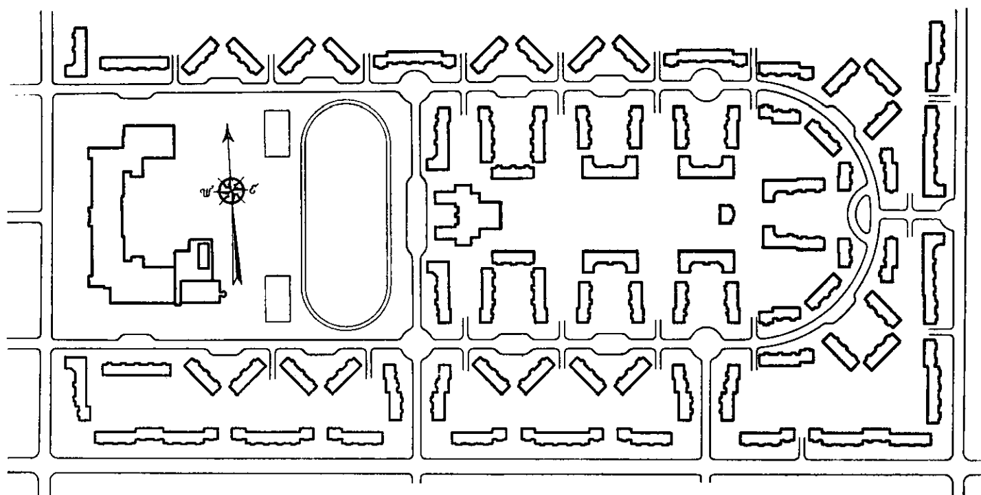
FIGURE 23.—Plan of Kenfield, Buffalo, N. Y.
