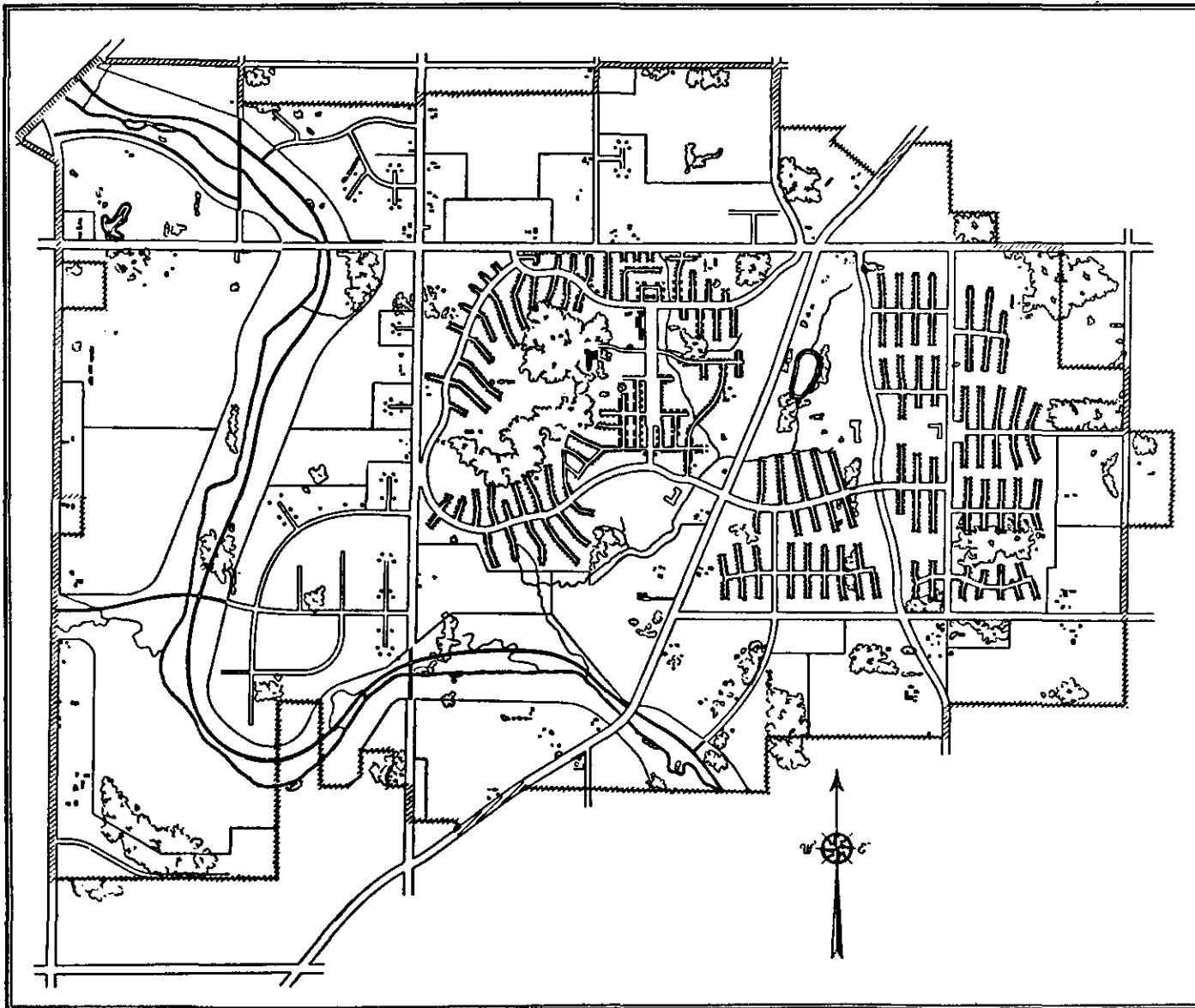
FIGURE 12.—Plan of the proposed ultimate development of Greendale, Wis., Farm Security Administration project.
