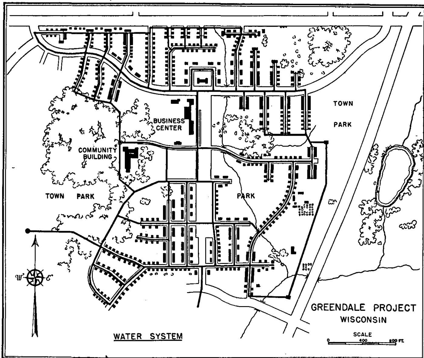
FIGURE 22.—Water system of the first town unit, Greendale, Wis.
