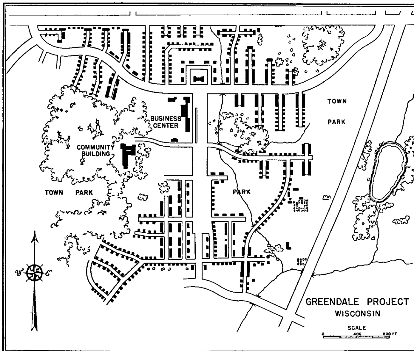
FIGURE 20.—Plan of the first town unit of Greendale, Wis., Farm Security Administration project.
