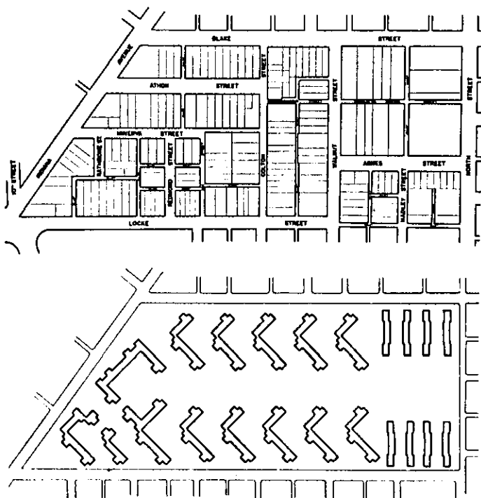
FIGURE 25.—Comparison of Original Street and Alley Layout and Site Plan of Lockefield Garden Apartments, at Indianapolis, Ind.
