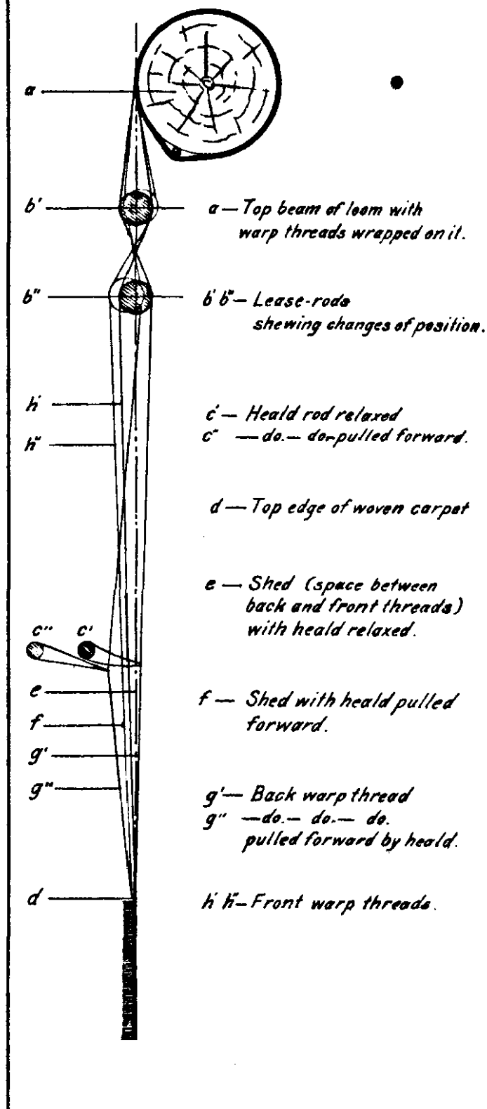
Sectional Elevation of Carpet Loom Illustrating movement of Lease-rods.
