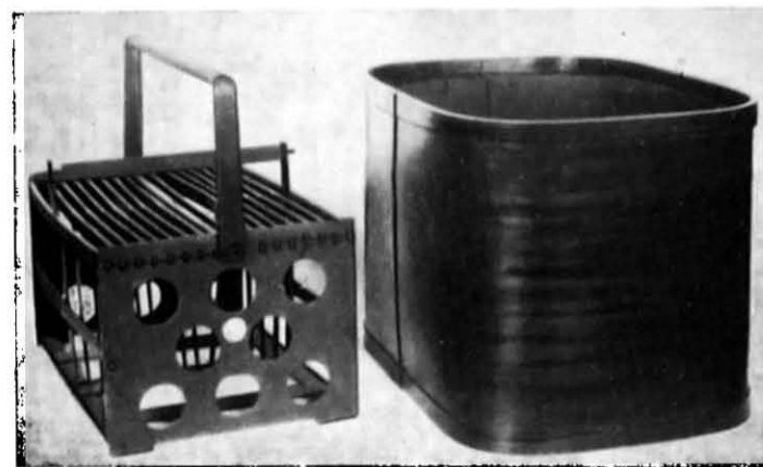
Fig. 49. Celluloid set for treating eggs with hydrochloric acid. Acid solution is made in the vessel. On the left side is the frame in which egg cards are placed and the frame with egg cards is dipped into the solution.
