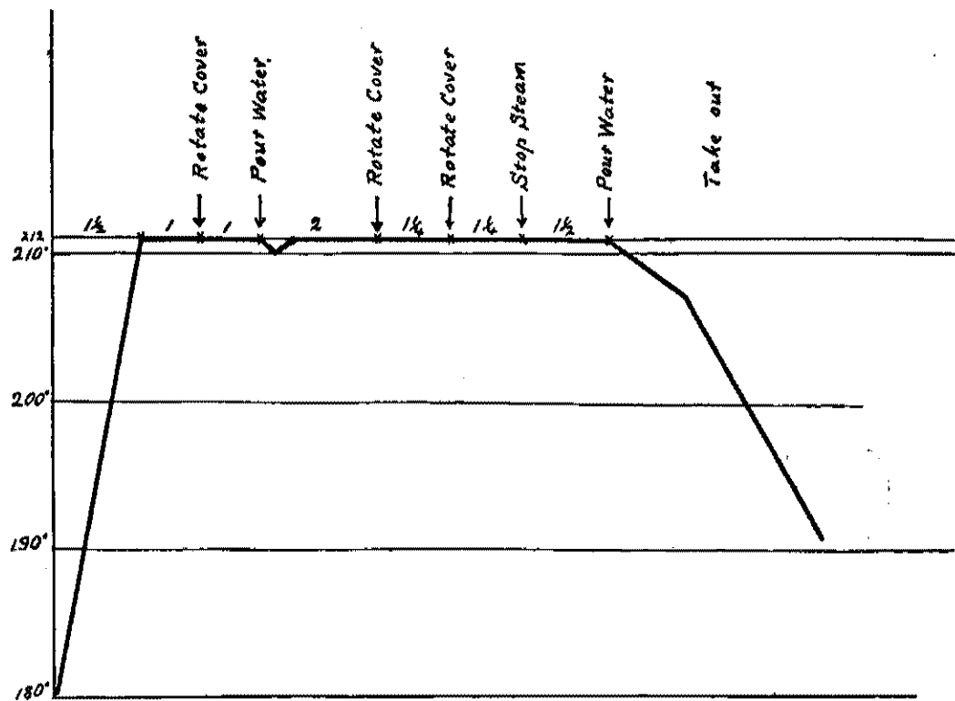
Fig. 52. Chart for cooking for sunken method of reeling. The figures 1, 1 1/2, etc., indicate periods in minutes.
