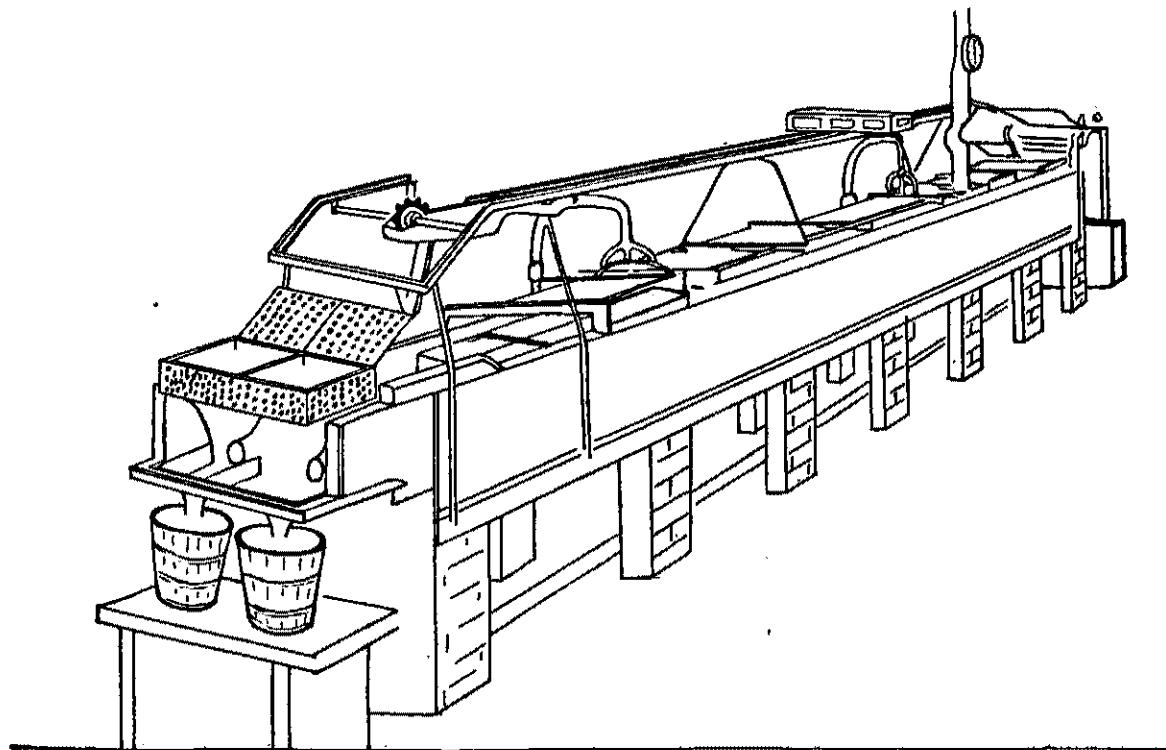
Fig. 53. Continuous cooking plant (Rather diagrammatic).
