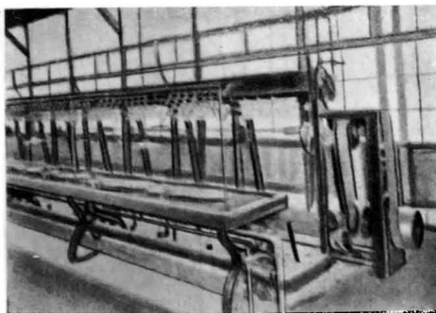
Fig. 18. Details of common filature machinery. Basins are fixed on a table. The small reels rotate above and behind the reeler under a sort of concave roofing containing heated gas pipe.
