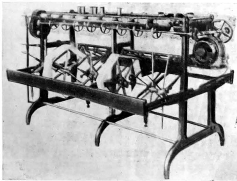
Fig. 42. Winding machine (Aswood).
