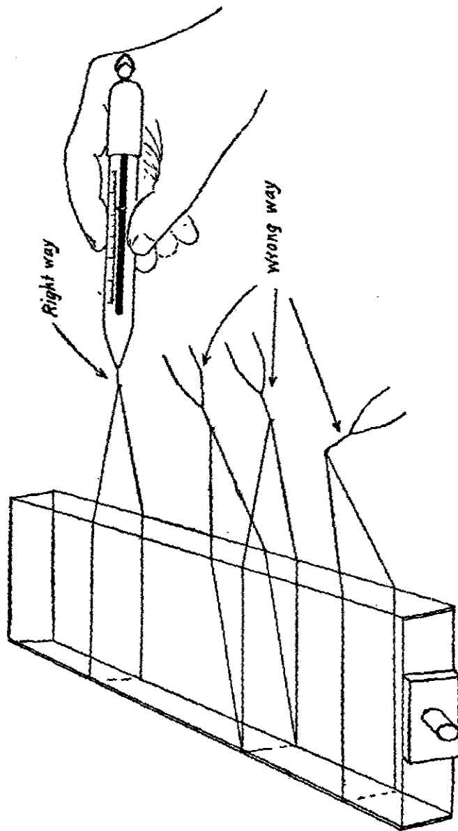
Fig. 43. Hand Serimeter—Correct method of pulling the thread on the inspection board is indicated.
