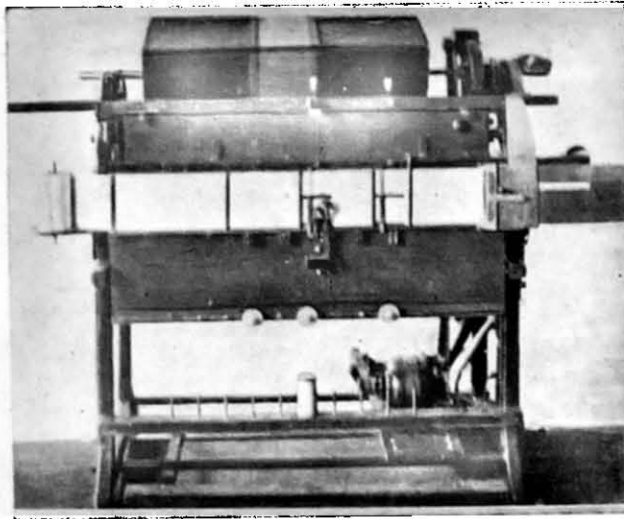
Fig. 46. Wyckoff's Evenness Tester.
