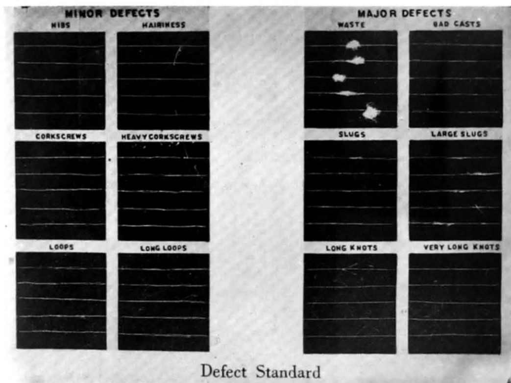
Fig. 32. Defects standard.
