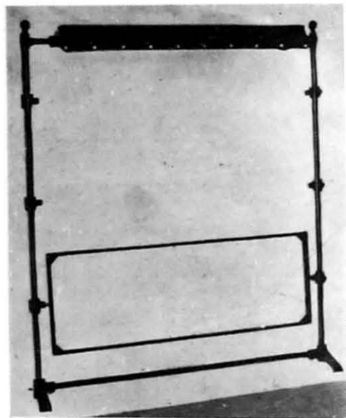
Fig. 35. Rack on which inspection boards are required to be placed. The evenness standard and two inspection boards are accommodated at the same time.
