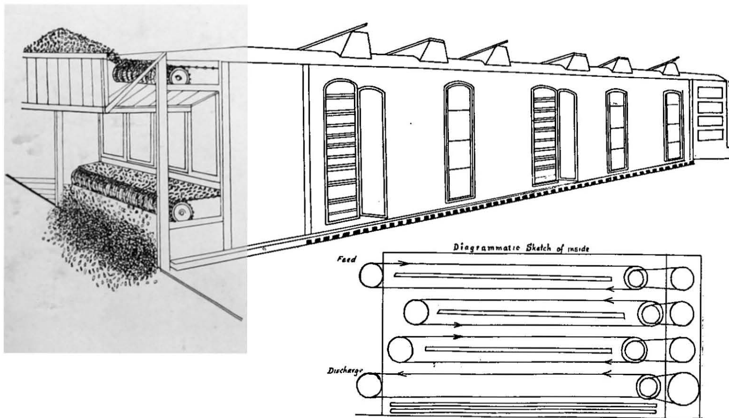
Fig. 24. Imamura plant for continuous drying of cocoons. (Diagrammatic sketch.)
