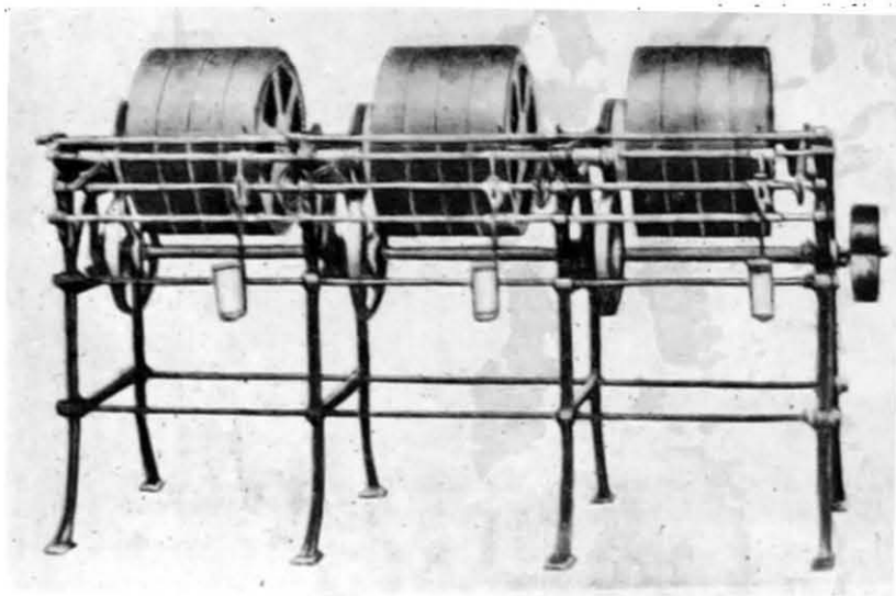
Fig 44. Inspection drums.
