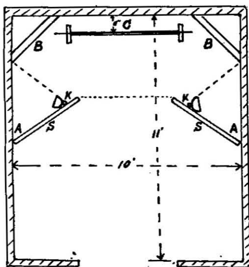
Fig. 34. Seriplane board inspection room. External surfaces of reflecting screens S, walls B, C and floor inside dotted lines are painted flat gray. The rest of the floor and walls, ceiling and internal surfaces of screens are flat white.
