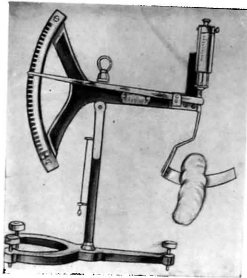
Fig. 26. Hank weighing balance.
