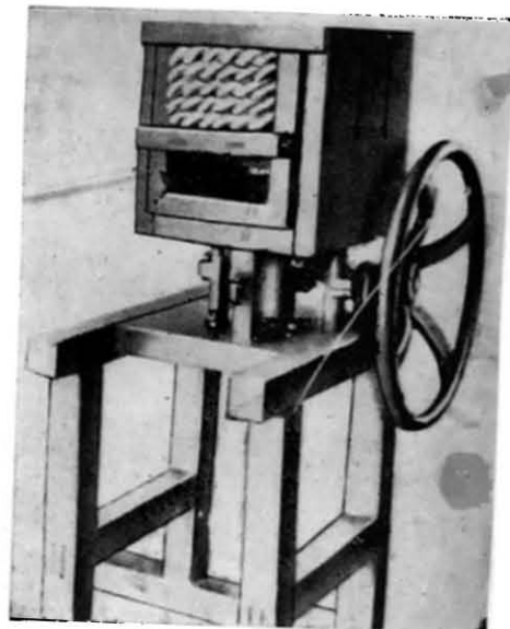
Fig. 28. Book-making machine.
