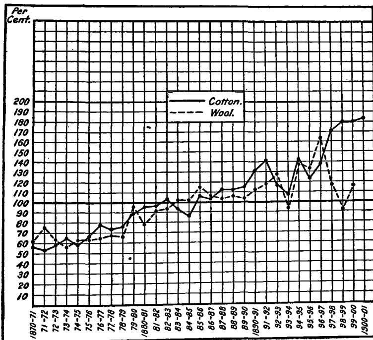
CHART 7.—Takings of cotton and woolen mills, 1870-1901.
