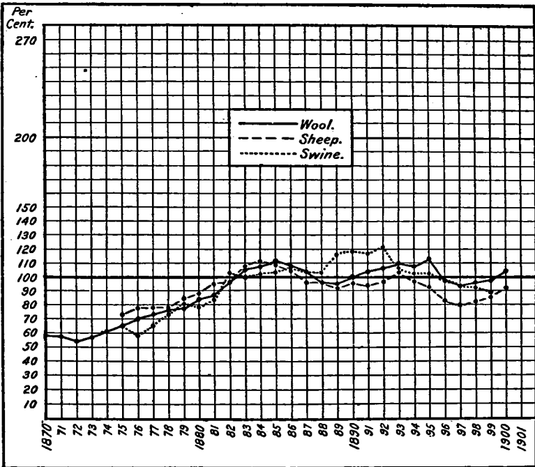
CHART 4.—Relative numbers of sheep and swine and annual wool clip, 1870–1900, averages for 1879–1888 being 100.
