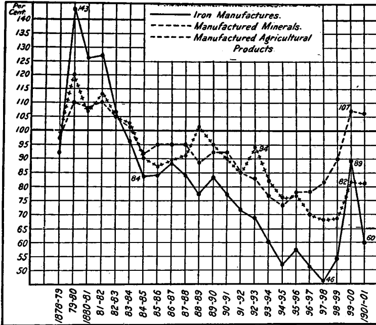
CHART 5.—Wholesale prices, 1878-1901, average prices for 1879-1889 being 100.
