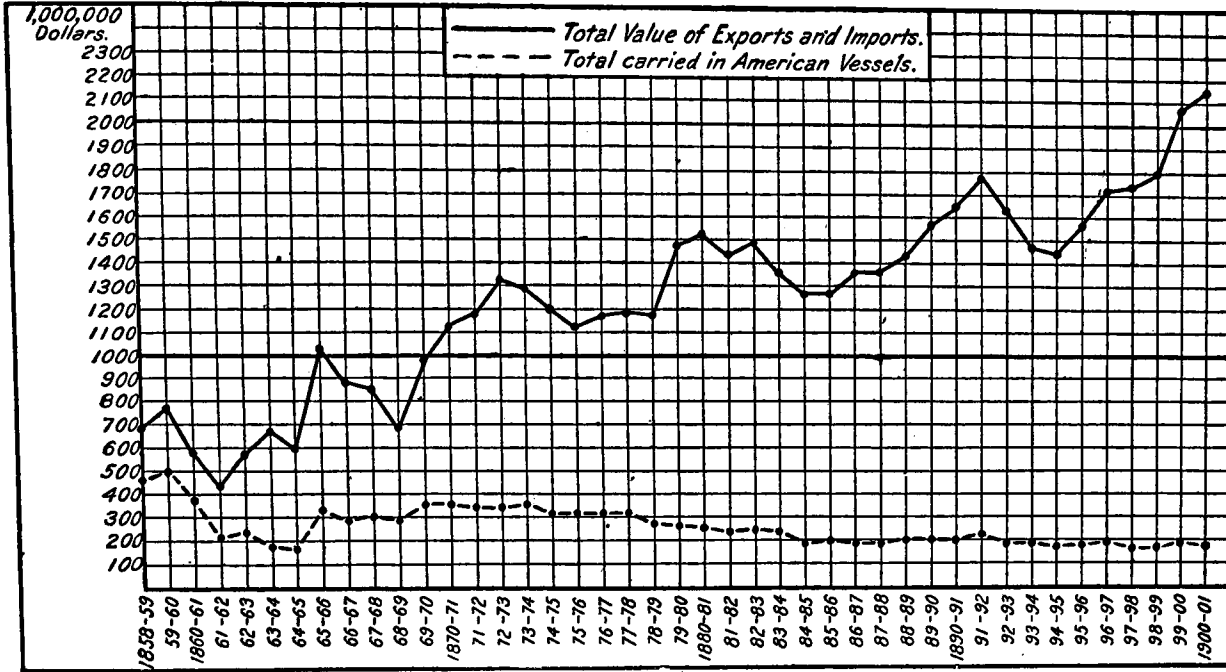
CHART 11.—Foreign carrying trade, 1858-1901.
