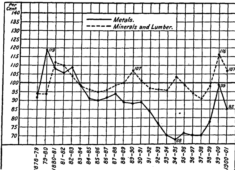
CHART 4.—Wholesale prices, 1878-1901, average prices for 1879-1889 being 100.
