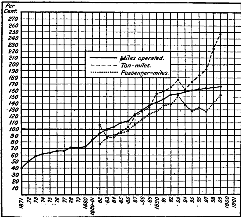
CHART 10.—Relative increase and decrease of miles of railroad operated, and passenger and ton-mileage, average for 1879-1888 being 100.
