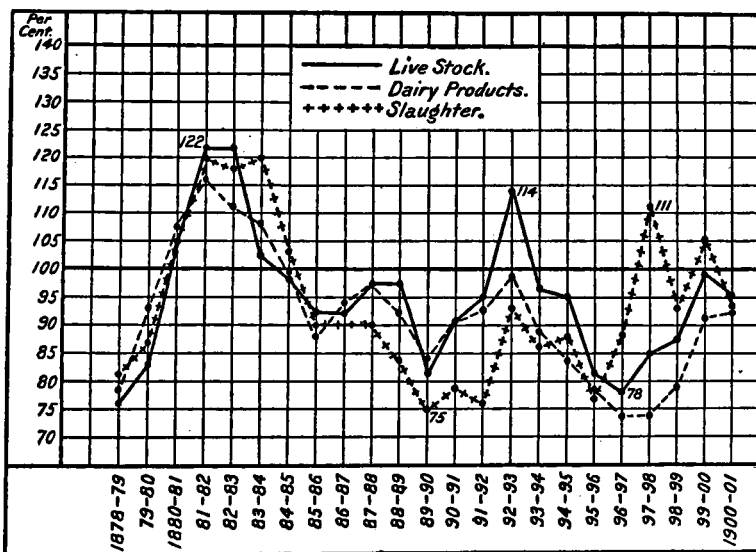
CHART 2.—Wholesale prices, 1878-1901, average prices for 1879-1889 being 100.
