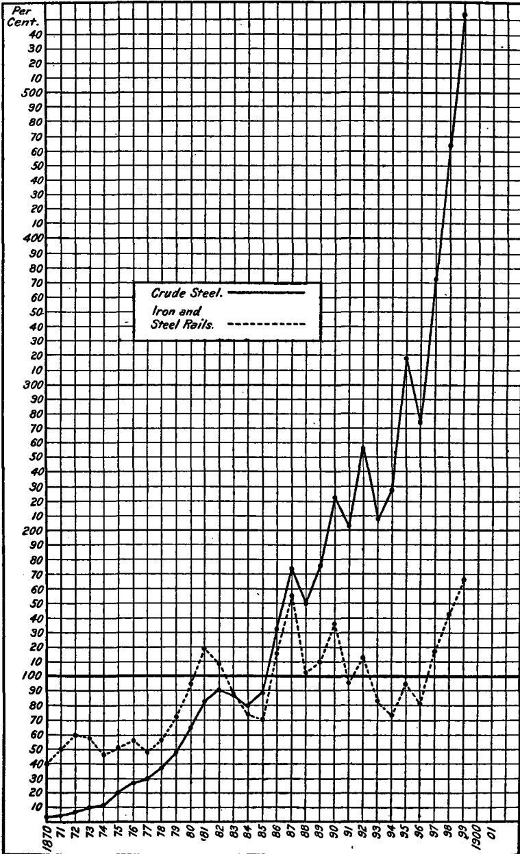
CHART 6.—Relative production of iron products, 1870-1899, average production for 1879-1888 being 100.
