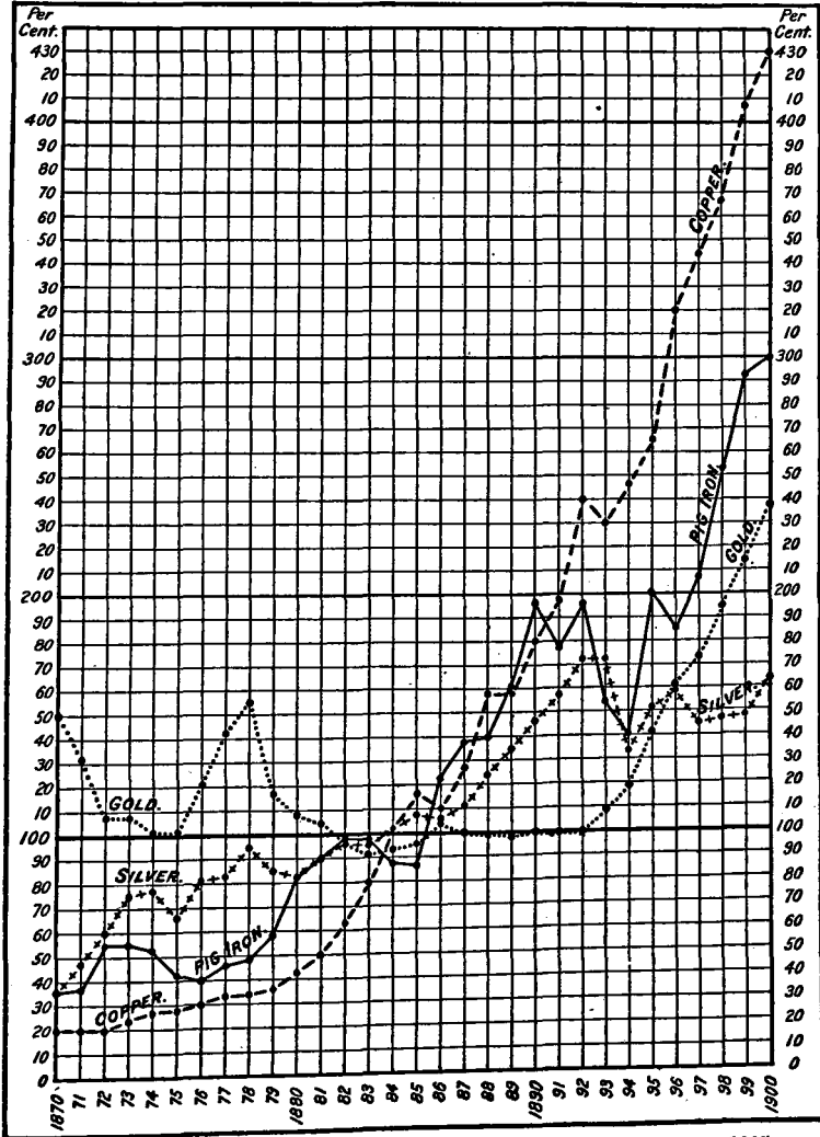
CHART I.—Relative changes in volume of production of gold, silver, pig iron, and copper, 1870-1900, average production for 1879-1888 being 100.
