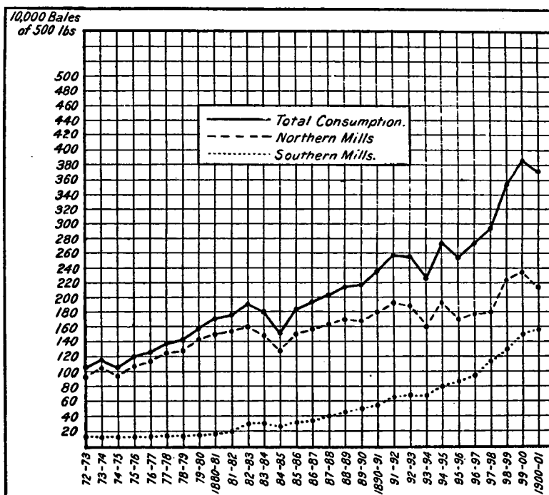
CHART 8.—Cotton consumption of mills in the United States.
