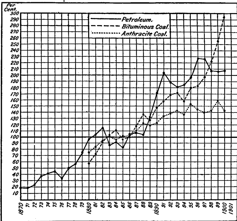
CHART 2.—Relative changes in volume of production of petroleum, anthracite coal, and bituminous coal, 1870–1900, average production for 1879–1888 being 100.
