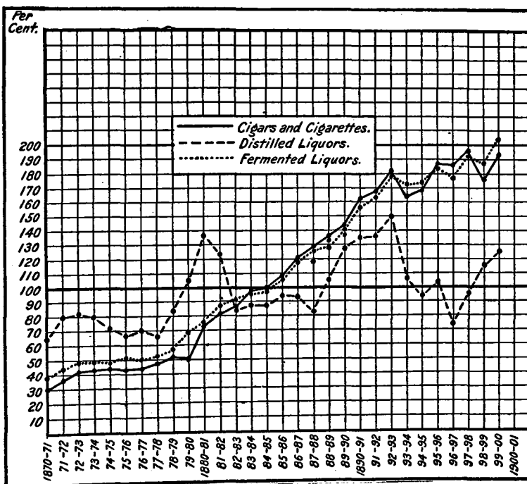
CHART 9.—Relative changes in production of distilled liquors, fermented liquors, and cigars, average production for 1879-1888 being 100.
