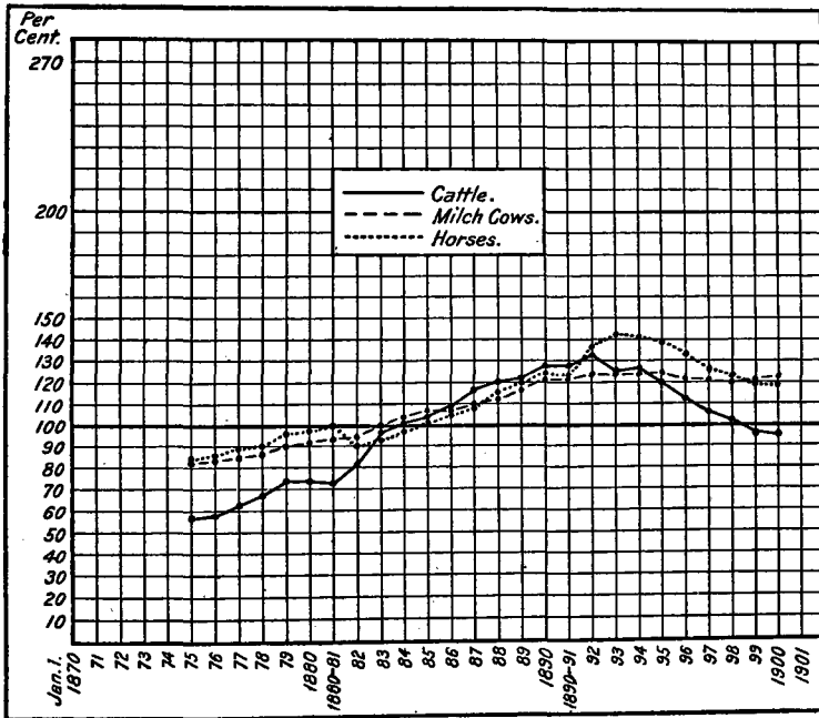
CHART 5.—Relative numbers of horses, milch cows, and cattle, 1874-1900, average numbers for 1880-1889 being 100.
