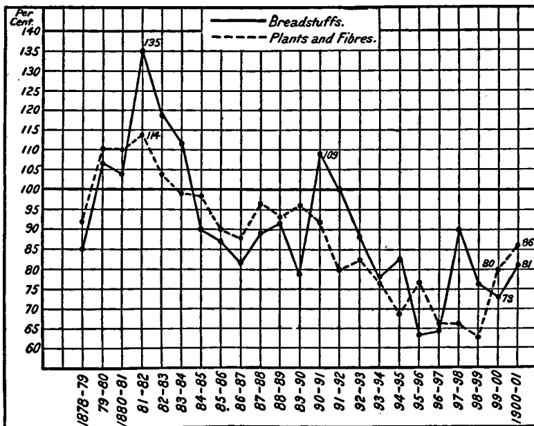
CHART 3.—Wholesale prices, 1878-1901, average prices for 1879-1889 being 100.
