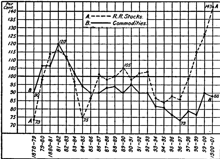
CHART 1.— Wholesale prices, 1878-1901, average prices for 1879-1889 being 100.
