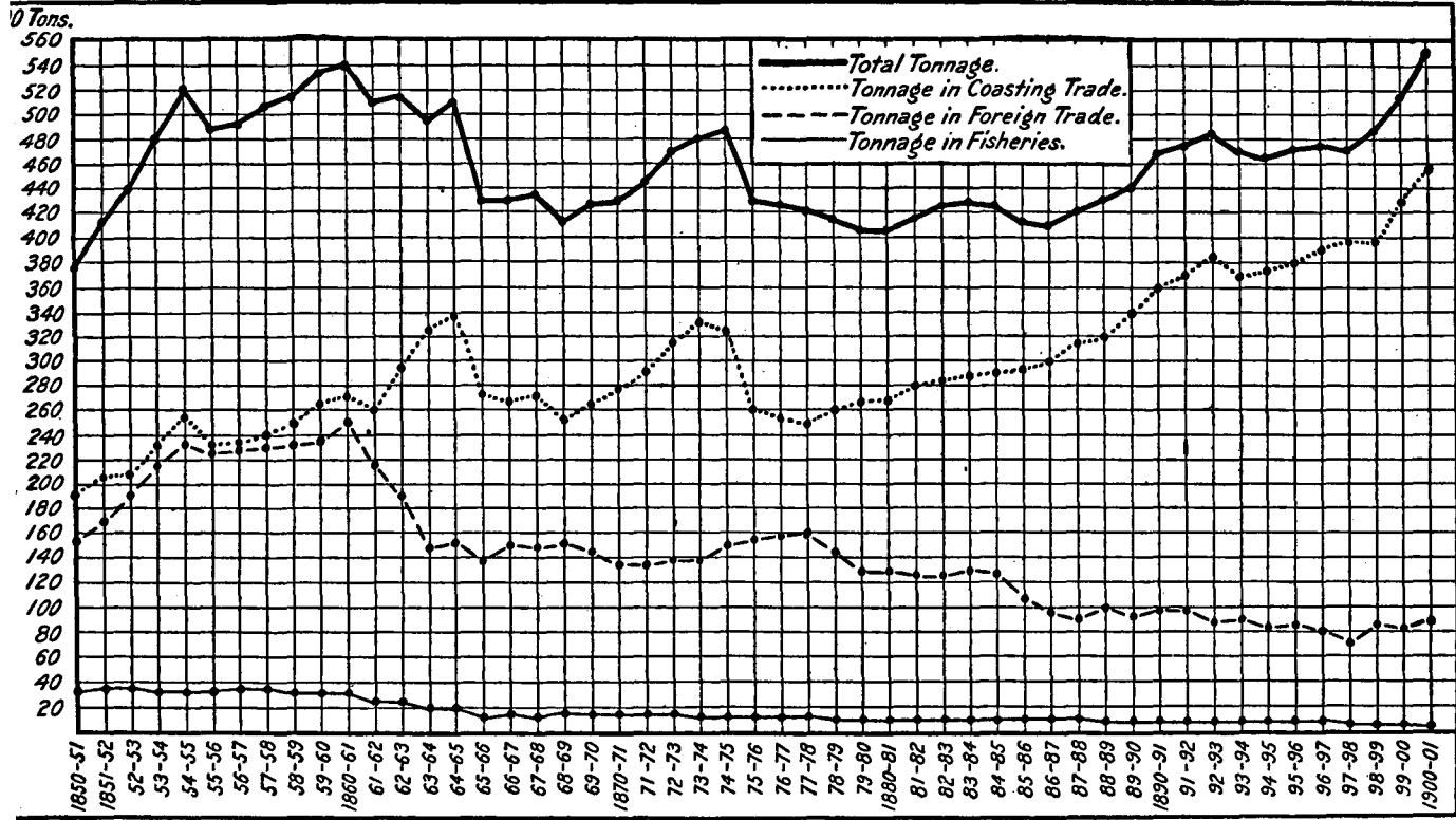
CHART 12.—Distribution of tonnage, United States merchant marine, 1851-1901.
