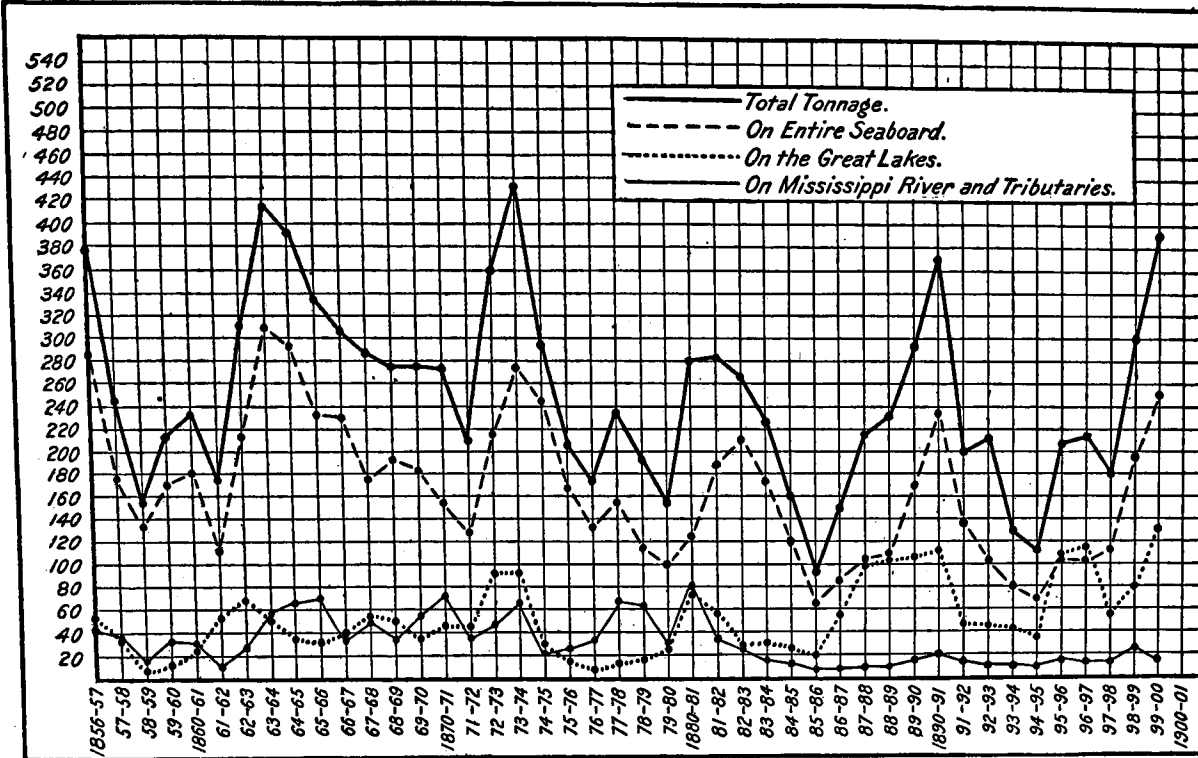
CHART 13.—Tonnage of vessels built in the United States, 1857-1901.
