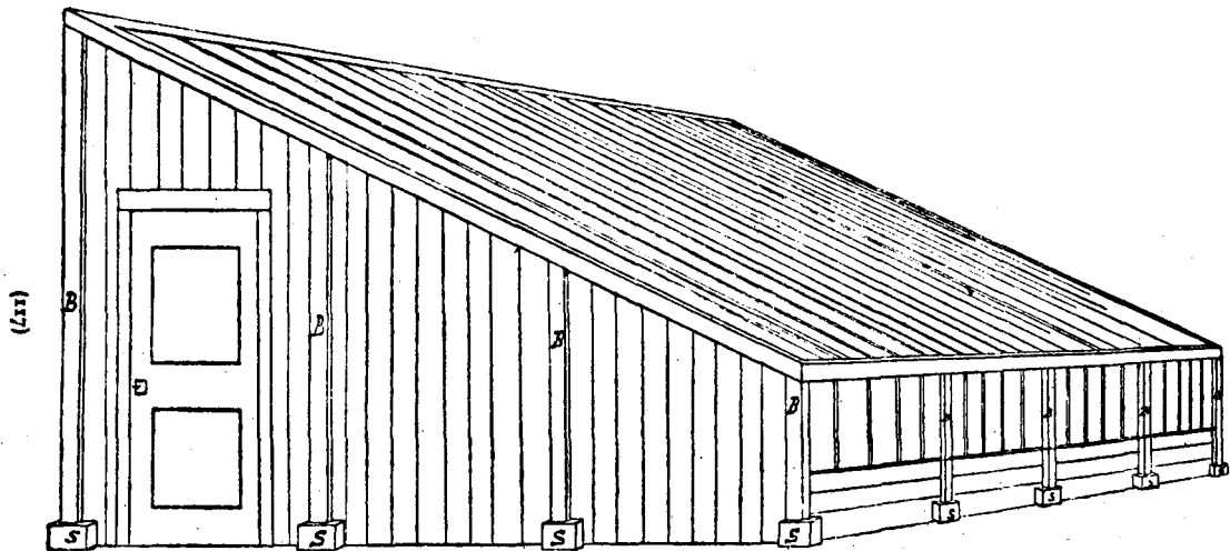
FIG. 7.—Cool Greenhouse of the plainest description in Guernsey. s , Concrete stones mounted on purpose to receive the standards b, b ; the spaces between them being fitted with matching-boards, which enter a groove in the stone s .
