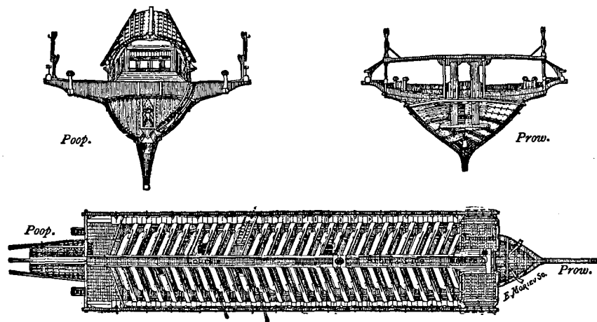
PLAN AND SECTIONS OF A GALLEY.
