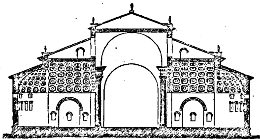
Transverse Section of Basilica of Maxentius.
