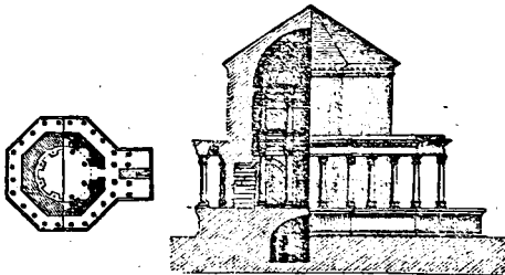
Plan and Elevation of Octagon Temple in Diocletian's Palace at Spalatro.
