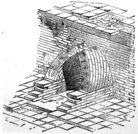
35.—VAULTED DRAIN. (KHORSABAD.) (Perrot and Chipiez.)
