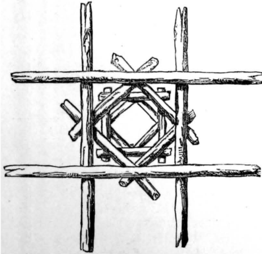
33.—ARMENIAN LOUVRE (Botta.)
