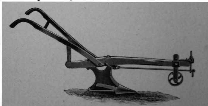
FIG. 9. SUBSOIL PLOW.
