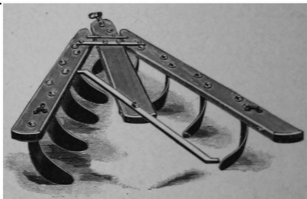
FIG. 23. SHARES HARROW.
