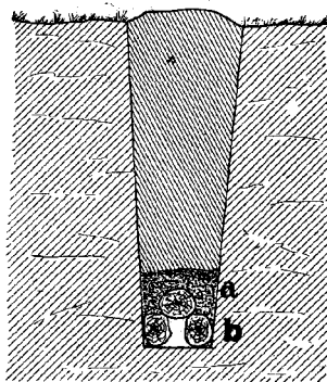
FIG. 43. Section of Pole Drain: a , gravel covering; b , poles.
