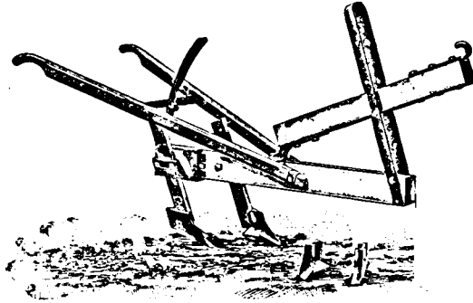
FIG. 53. DITCHING PLOW.
