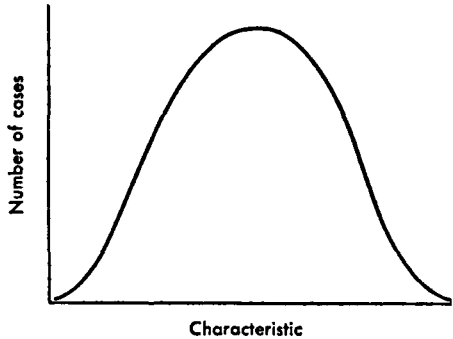
FIGURE 2. Curve of normal distribution.
