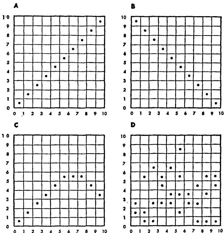
FIGURE 3. Scattergram representations of various types of correlation: (A) perfect positive correlation; (B) perfect negative correlation; (C) perfect curvilinear correlation; (D) perfect low correlation.
