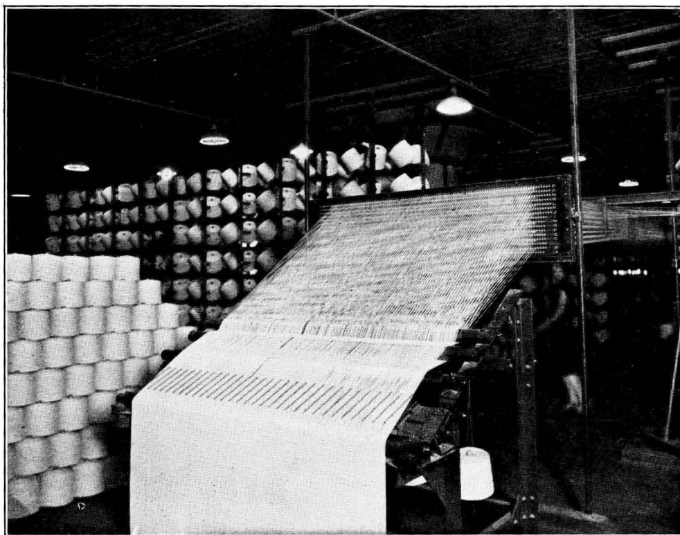
FIGURE 2.—SHEET OF INDIVIDUAL WEFTLESS CORDS GUIDED BY CENTRAL BOARD AND GATHERING COMB DIRECTLY INTO CALENDER.
