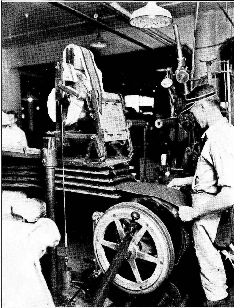
FIGURE 5.—DRUM PROCESS OF TIRE BUILDING: PLACING AND APPLYING SECOND PLY OF TIRE.
