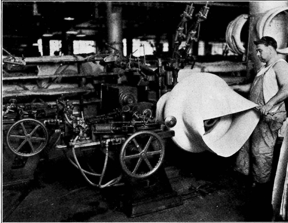
FIGURE 4.—CORE PROCESS OF TIRE BUILDING; DRAWING ENDLESS BAND OF 2 PLYS OVER CORE WITH HELP OF WOODEN OR IRON BAR.
