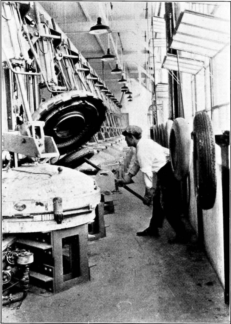
FIGURE 7.—CURING TIRES; EXTRACTING CURED TIRE FROM WATCHCASE VULCANIZER.
