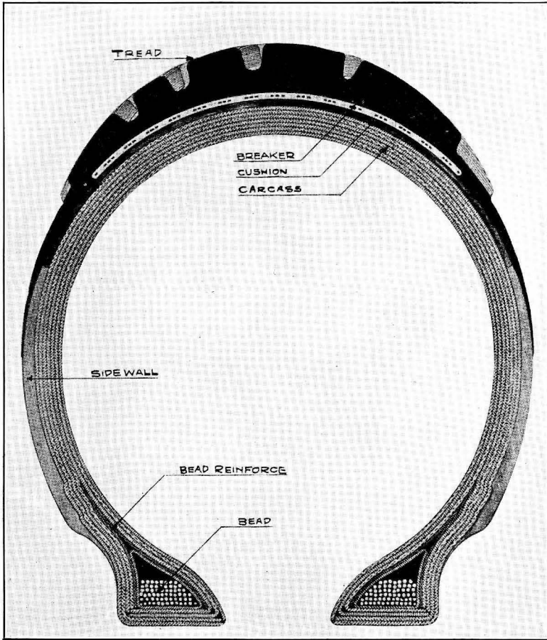
FIGURE 3.—CROSS SECTION OF CORD TIRE.
