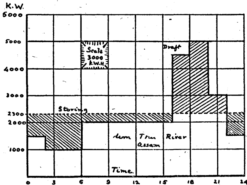
Fig. 19. Regulating storage.
