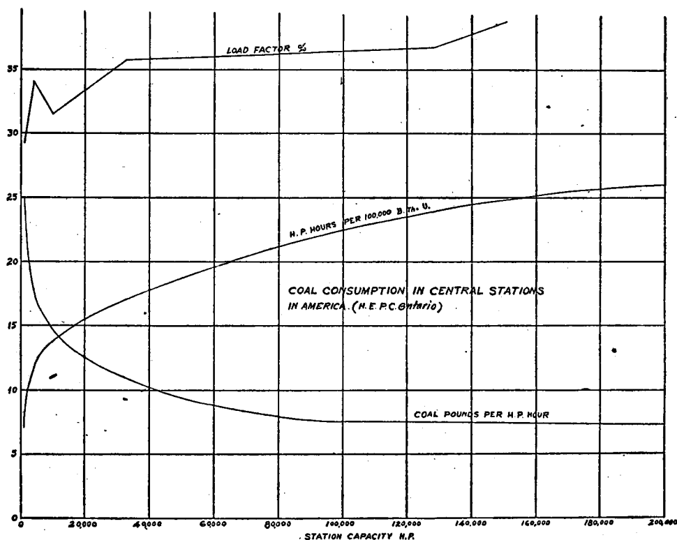
FIG. 21. Coal consumption in Central Stations.
