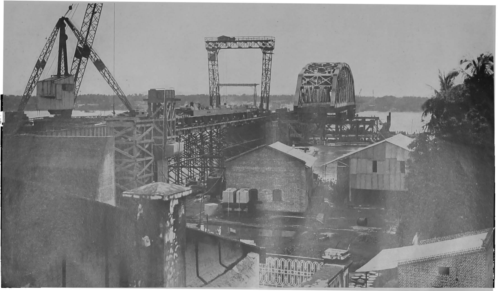
Bally Bridge—Floating first span into position.
