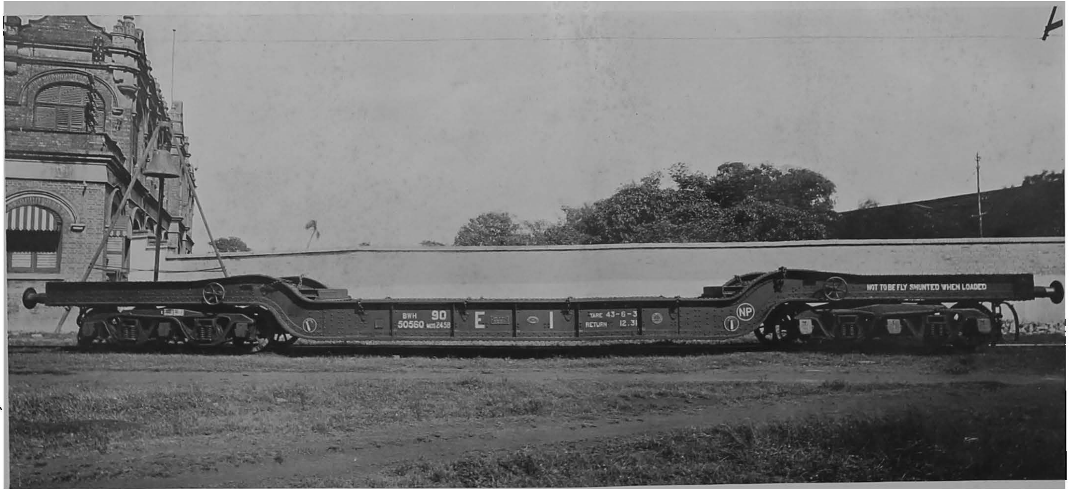
New high capacity well wagon—135 tons gross load.
