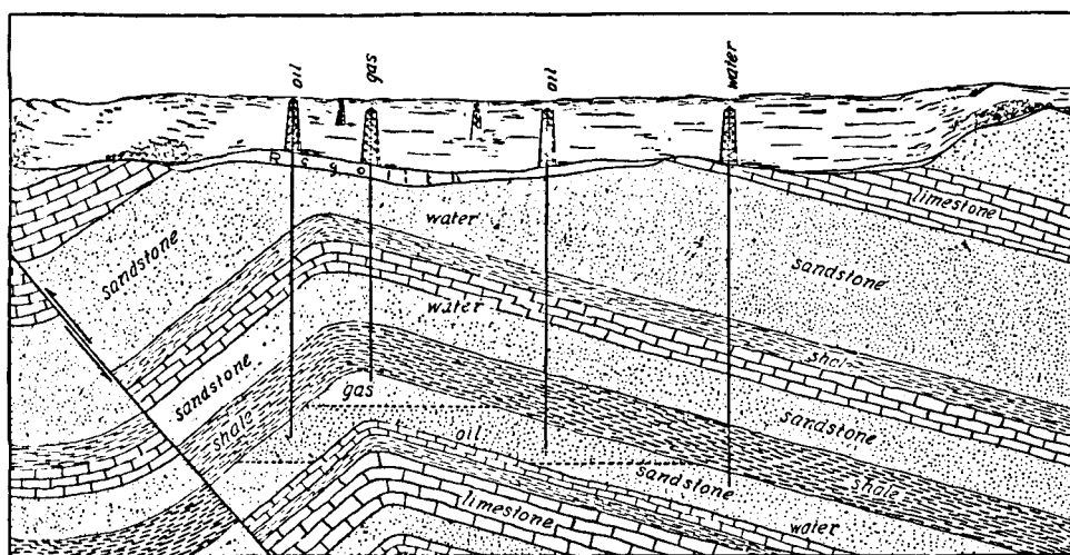
FIG. 338.—A diagram to illustrate one form of structure in which petroleum is entrapped and the relation between the locations of several wells and the nature of their products. The existence of this anticlinal structure is not evident from the surface relief.
