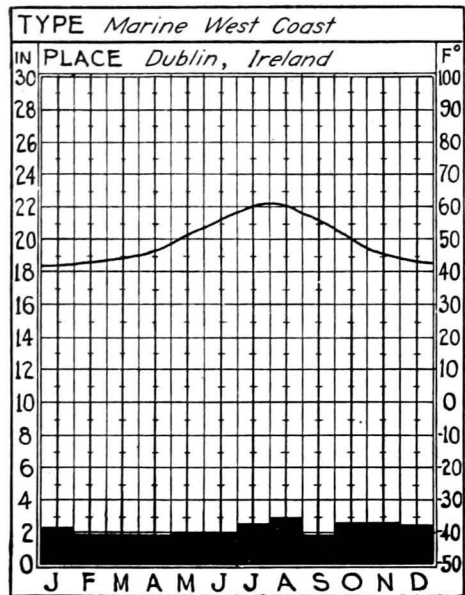
FIG. 95.—Average monthly temperatures and precipitation for a representative station in marine west-coast climate.
