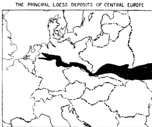
FIG. 213.—The principal loess region of Europe is closely associated with the margin of the older glacial drift. (cf. Fig. 198.) (After Paul Woldstedt, Das Eiszeitalter. )
