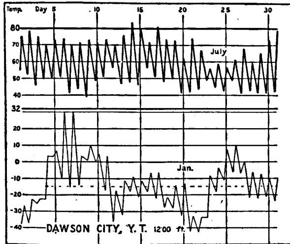
FIG. 106.—Daily maximum and minimum temperatures for extreme months at a representative subarctic station in Canada. (Courtesy of Mark Jefferson and the Geographical Review.)
