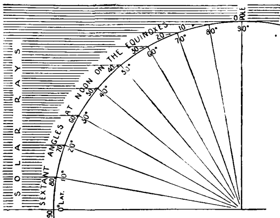
FIG. 2.—The angle at which the midday rays of the sun strike any place on the earth at the time of the equinox is the complement of the latitude of the place.
