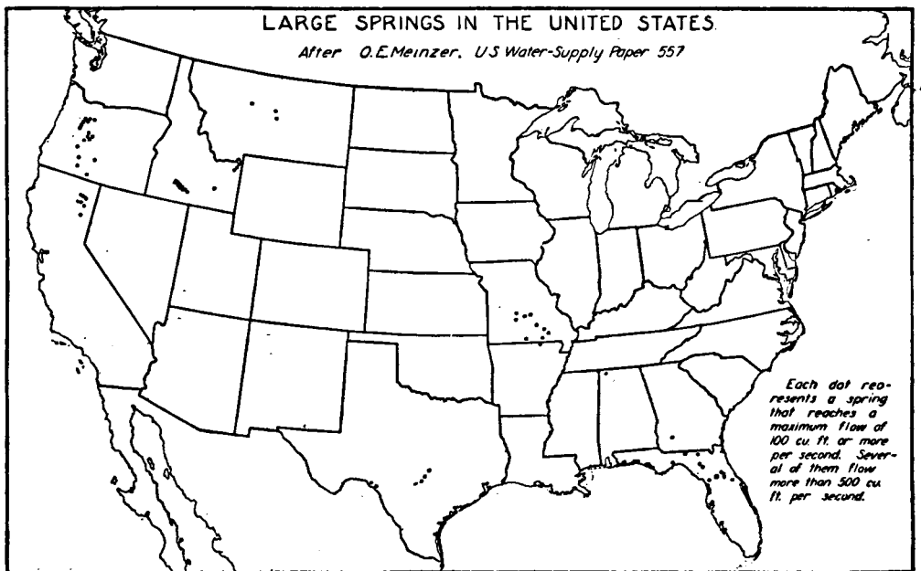
FIG. 277.—Most of the large springs of the United States occur in a few regional groups. Those in Florida, Missouri, and Texas mainly are associated with areas of cavernous limestones, while those of Idaho, Oregon, and California occur more largely in porous-lava formations.
