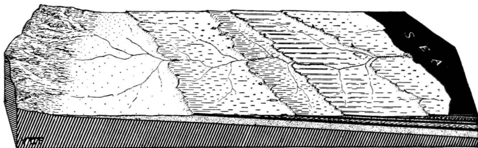
FIG. 141.—A diagram to illustrate the cuestaform ridges, intervening lowlands, and related rock structure of a belted coastal plain. The rock strata shown in solid black are indicated as having superior resistance.
