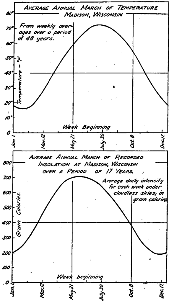
FIG. 20.—Note that temperature lags behind insolation. Insolation curve has been smoothed slightly.
