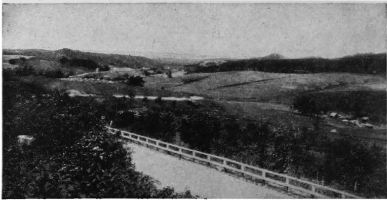
FIG. 146.—Rough dissected plain in southwestern Wisconsin. The local relief in this region averages about 500 ft., but in some localities it exceeds that figure and the surface is truly hilly. ( Wisconsin Geological Survey Photograph. )
