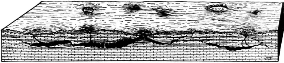
FIG. 153.—A diagram illustrating karst plain features. Sinks of various types are shown in relation to features of limestone solution underground.
