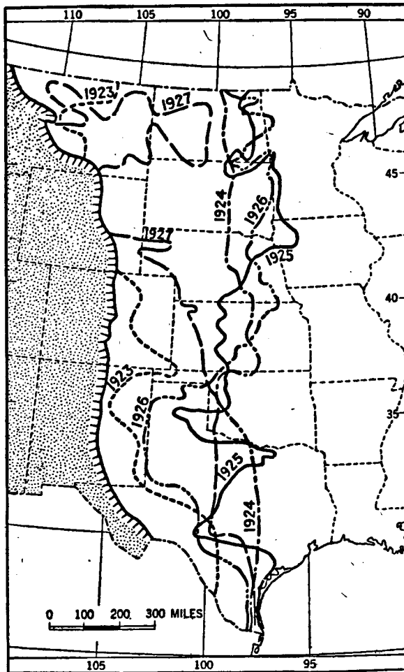
FIG. 85.—Fluctuations in the boundary separating dry and humid climates, over a period of five years, for the region between the Mississippi River and the Rocky Mountains. (After H. M. Kendall.)
