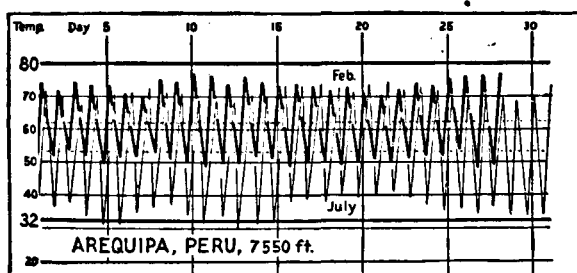
FIG. 110.—Daily maximum and minimum temperatures for a highland station in the tropics. (Courtesy of Mark Jefferson and the Geographical Review.)
