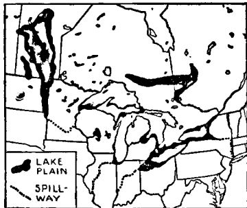
FIG. 202.—The principal glaciolacustrine plains and glacial spillways of North America.
