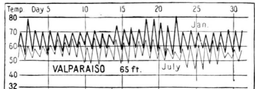
FIG. 87.—Daily maximum and minimum temperatures for the extreme months at a representative dry-summer subtropical station with coastal location in Chile ( Csb ). (Courtesy of Mark Jefferson and the Geographical Review .)
