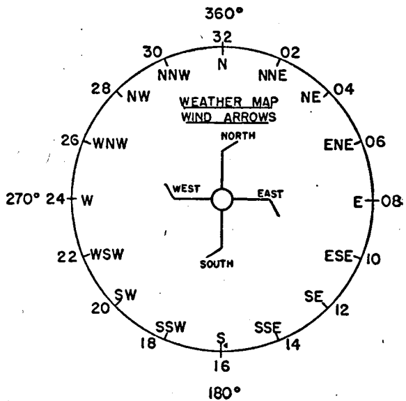
FIG. 33.—Here are shown the usually reported wind directions on a 32-point compass. (From Haynes.)
