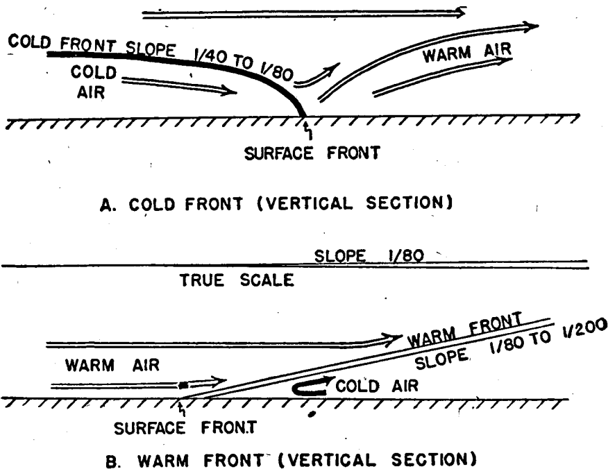
FIG. 52.—Surface fronts and discontinuity surfaces. (After Haynes.)
