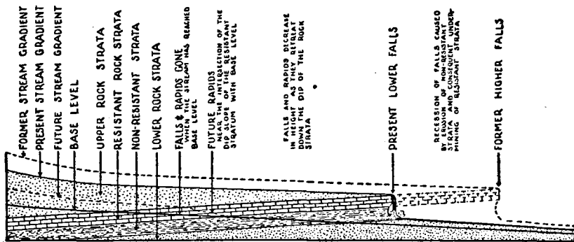
FIG. 130.—A diagram to illustrate one common cause of waterfalls and the reason why such falls retreat upstream, leaving a gorge, and eventually disappear.
