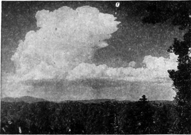
FIG. 47B.—Cumulo-nimbus cloud, or thunderhead. In such a cloud most of the earth's thunderstorms originate. ( U. S. Weather Bureau Photograph. )
