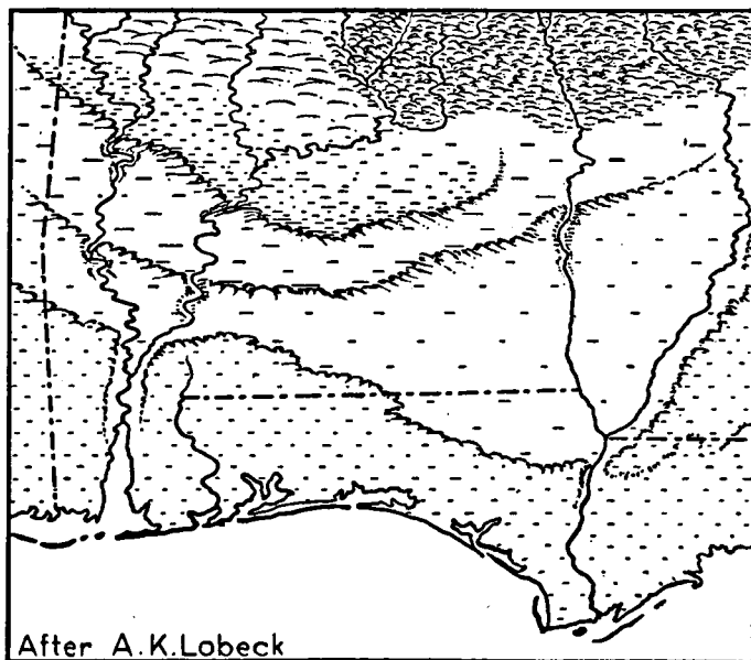
FIG. 142.—The principal cuesta form ridges of the Alabama Coastal Plain. The escarpments face northward.
