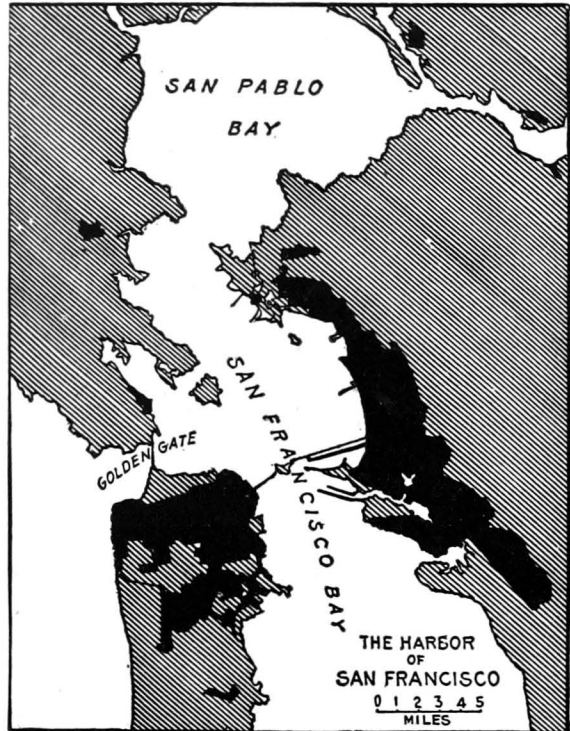
FIG. 416.—San Francisco has an excellent natural harbor, which is entered through the Golden Gate. Urban areas are shown in black.
