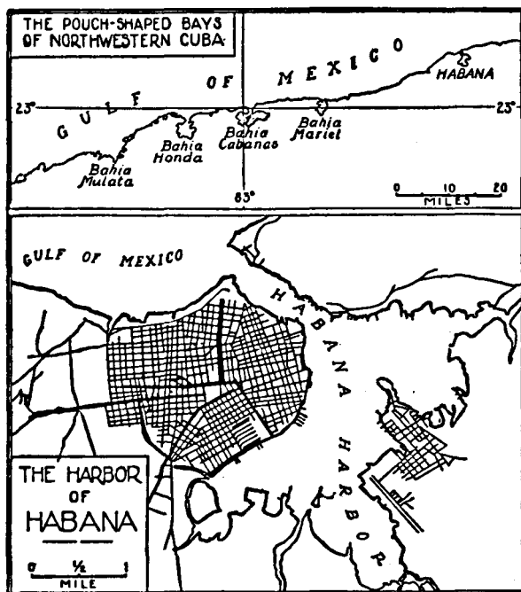
FIG. 226.—A series of pouch-shaped or "bottle-neck" bays in Cuba, and, below, details of outline for that one upon the shores of which the city of Habana is situated.
