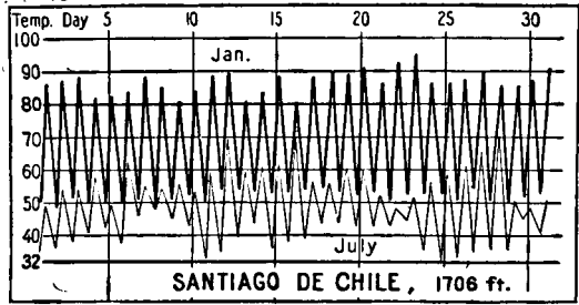
FIG. 88.—Daily maximum and minimum temperatures for the extreme months at a representative dry-summer subtropical station located interior from the coast in Chile ( Csa ). (Courtesy of Mark Jefferson and the Geographical Review .)
