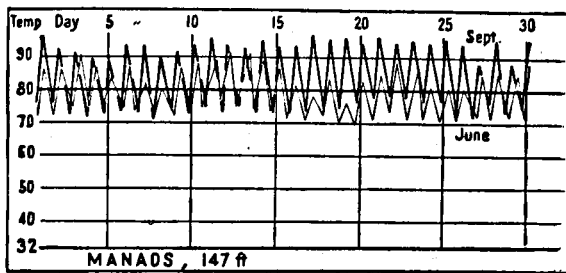
FIG. 72.—Daily maximum and minimum temperatures for the extreme months at a representative tropical rainforest station in the Amazon Valley. (Courtesy of Mark Jefferson and the Geographical Review.)
