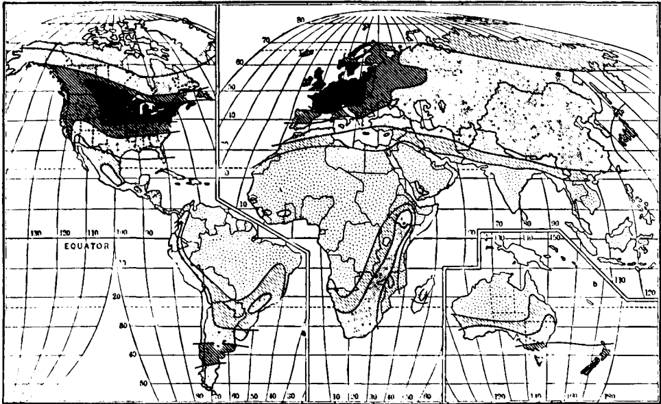
FIG. 354.—Distribution of climatic energy according to Huntington. The density of shading is roughly proportional to the degree of climatic energy. (From Huntington, "Principles of Human Geography," by permission of John Wiley & Sons, Inc.)
