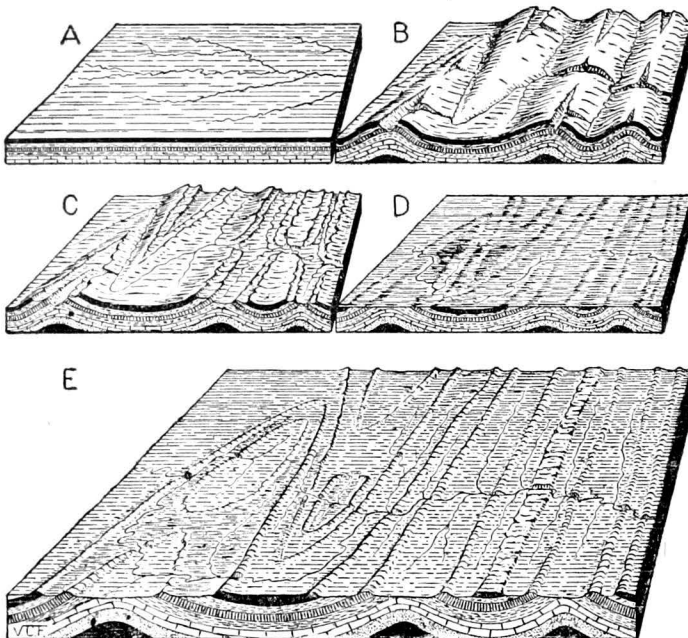
FIG. 241.—A series of diagrams in chronological sequence to illustrate the development of linear ridges, parallel valleys, and enclosed valleys. (A) horizontal strata; (B) anticlinal and synclinal folding, with pitching anticlines; (C) erosional mountains cut in the folded structures; (D) the region baseleveled; (E) the peneplain slightly elevated and re-eroded. Linear ridges, broad valleys, enclosed or canoe-shaped valleys, and water gaps are shown. They are of the types seen in the folded Appalachians.
