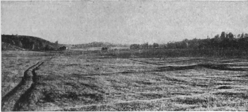
FIG. 203.—The flat-bottomed channel of a former glacial spillway, not now occupied by any stream. ( Wisconsin Geological Survey Photograph. )
