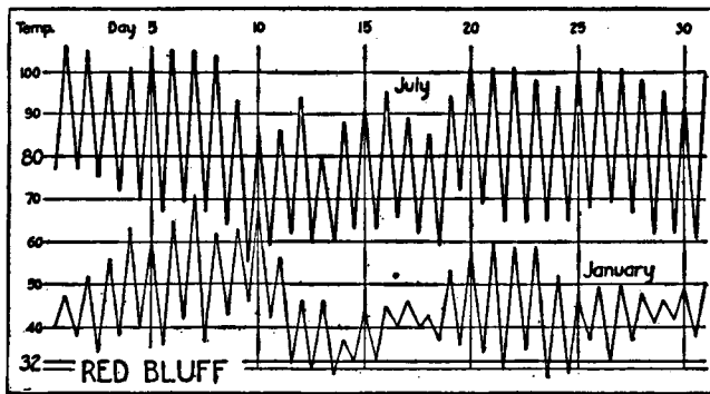
FIG. 89.—Daily maximum and minimum temperatures for the extreme months at a representative dry-summer subtropical station located interior from the coast in California ( Csa ).
