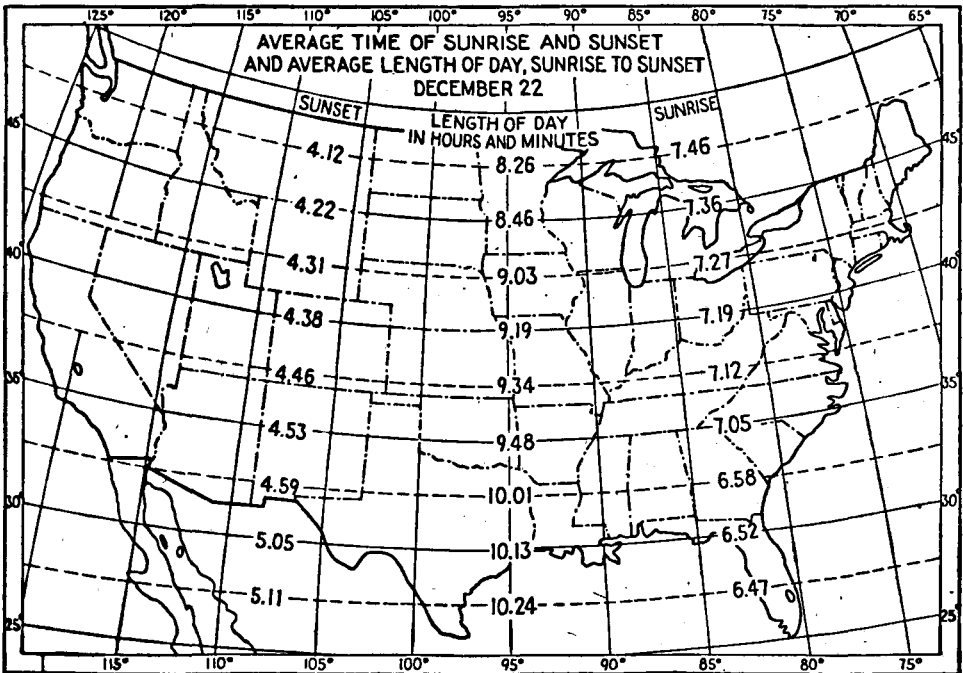
FIG. 14.—At the time of the winter solstice, days are about 2 hr. shorter in northernmost United States than they are in the extreme south. Length of day decreases with latitude until north of the Arctic Circle the sun on Dec. 22 does not rise above the horizon. (After Kincer.)
