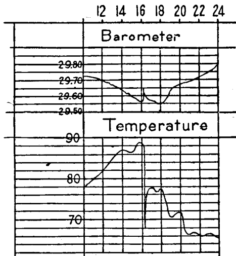
FIG. 67.—Record of pressure and temperature at the Naval Air Station, Anacostia, D. C., during the approach and passage of the squall-line storm shown in Fig. 66. Hours indicated at top.
