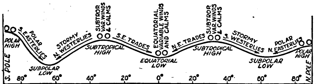
FIG. 28.—A very diagrammatic representation of a profile of surface pressure and wind belts as they might appear on an earth with a homogeneous surface. Compare with Fig. 39.
