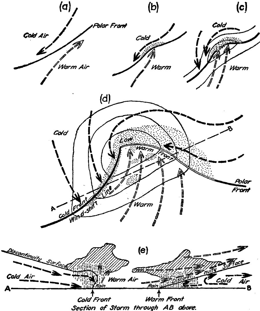
FIG. 54.—Growth and structure of a middle-latitude cyclone. (a), (b), and (c) Stages in the development of a cyclone. (d) The fully developed cyclone on a somewhat larger scale and in more detail. (e) A cross section of the same storm. (Modified after Namias.)
