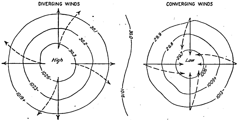
FIG. 51.—Surface wind systems in stationary cyclones and anticyclones diagrammatically represented. Solid arrows indicate direction of air flow on a nonrotating earth; dashed arrows, the deflected winds on a rotating earth. Pressure readings in inches and millibars.
