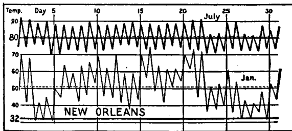
FIG. 92.—Daily maximum and minimum temperatures for the extreme months at a representative station in the humid subtropics. Note the greater irregularity in winter. (Courtesy of Mark Jefferson and the Geographical Review.)
