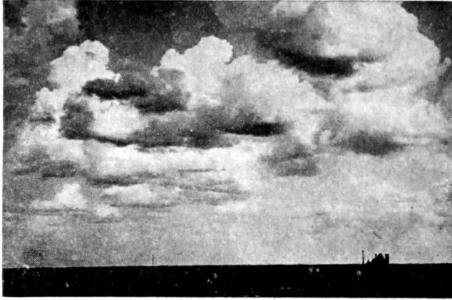
FIG. 47A.—Cumulus clouds. ( U. S. Weather Bureau Photograph. )
