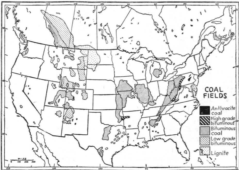
FIG. 330.—The principal coal fields of the United States and Canada distinguished as to location, extent, and principal types of coal.
