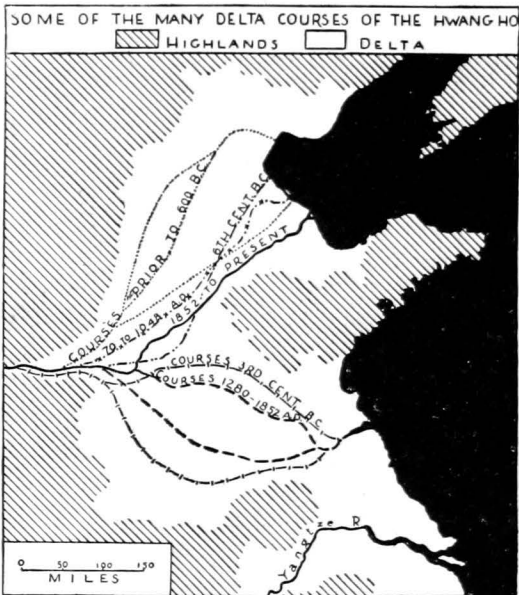
FIG. 162.—The great delta of North China, its relation to the Shantung Peninsula, and some of the many channels the river has occupied within historic times. (After maps by G. B. Cressey and D. W. Mead.)
