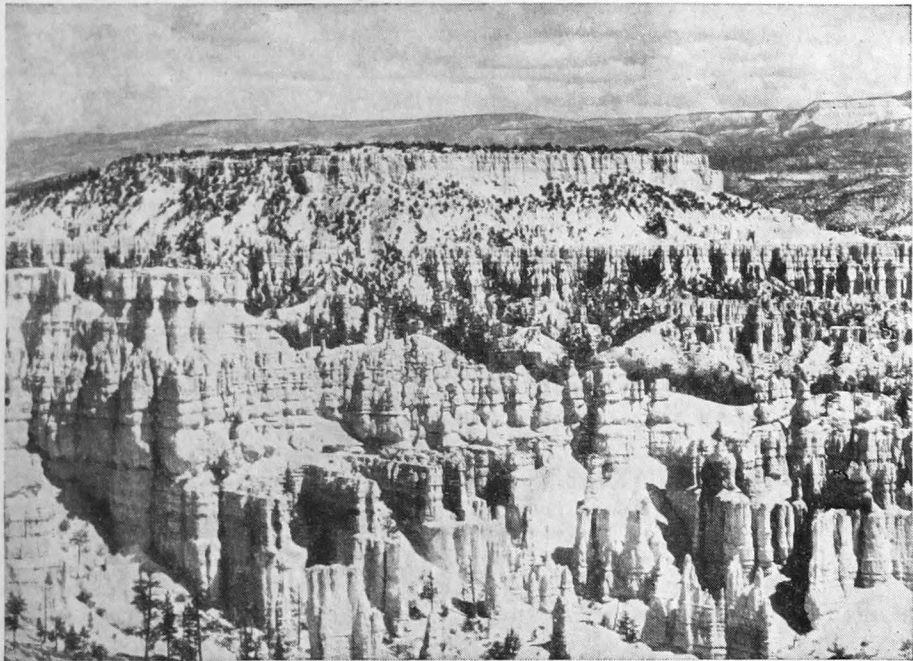
FIG. 233.—Fantastic details resulting from the differential weathering and erosion of a dry-land escarpment in Bryce Canyon, Utah. The steep sides and flat top of the mesa in the middle distance are well shown. ( National Park Service, U. S. Department of the Interior. )
