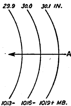
FIG. 32.—Gradient is represented by a line drawn at right angles to the isobars.
