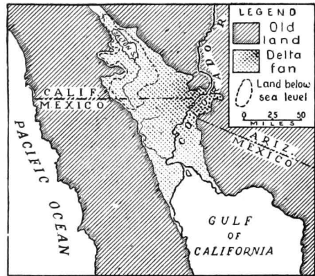
FIG. 163.—The apex of the delta fan of the Colorado River is at the east side of the long embayment into which it is built. The location and extent of Salton Sink are indicated by the broken line. Salton Sea lies in its lowest portion, its bottom 274 ft. below sea level.
