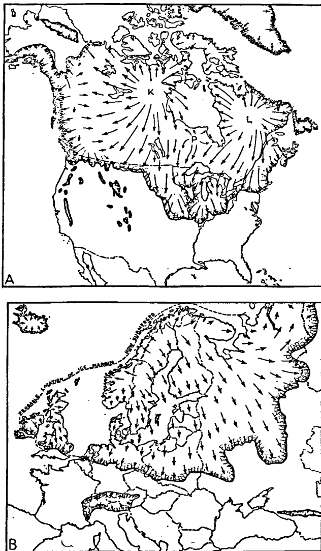
FIG. 134.—The maximum extent of the continental glaciers of North America and Europe. (A) The letters indicate the Keewatin, Patrician, and Labradorian centers of glacial movement. (B) The principal center of European glaciation was in the highlands of Scandinavia.
