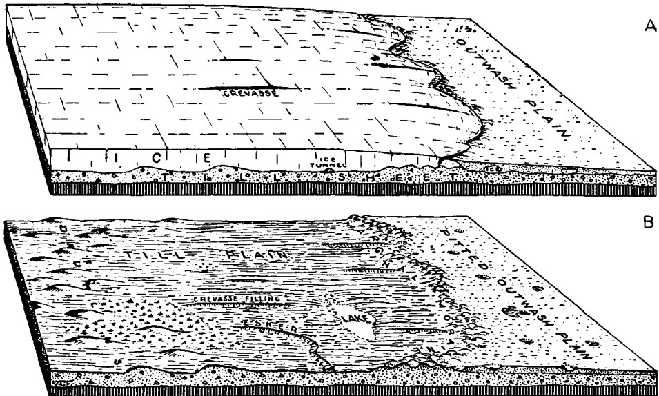
FIG. 181.—A diagram to illustrate the relationship of several classes of glacial and glaciofluvial deposits to the parts of the glacier by which they were formed. (A) A plain partly covered by the margin of a stagnant glacier; (B) the same plain after the disappearance of the ice by melting.
