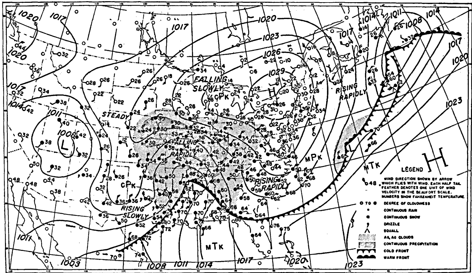
FIG. 51A.—The principal (surface) United States weather map for 7:30 A.M., Mar. 29, 1939.
