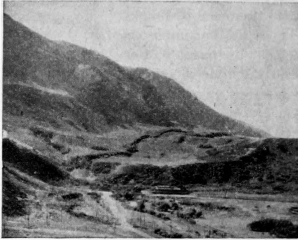
FIG. 116.—The latest step in the growth of a great fault-line scarp. front of the Wasatch Mountains, a fault-line scarp. Parallel to it, the low scarp of a recent fault is shown by the dark line that traverses the piedmont alluvium. ( U. S. Geological Survey Photograph. )
