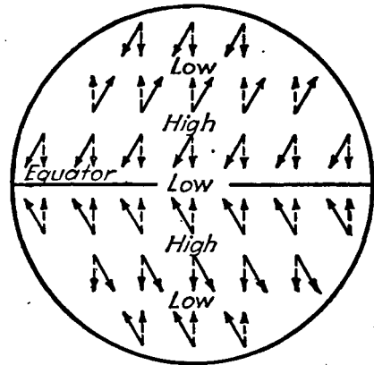
FIG. 35.—Dashed arrows show wind direction as determined by pressure gradient alone and without the effects of earth rotation. Solid arrows show the deflected winds on a rotating earth.
