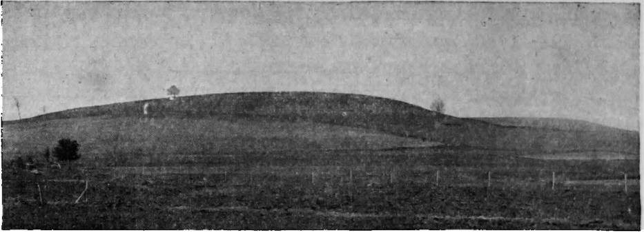
FIG. 186.—A pair of drumlins on the till plain of central New York. Their shapes indicate that the direction of glacier movement was from right to left. (cf. Figs. 181, 187.) (U. S. Geological Survey Photograph.)
