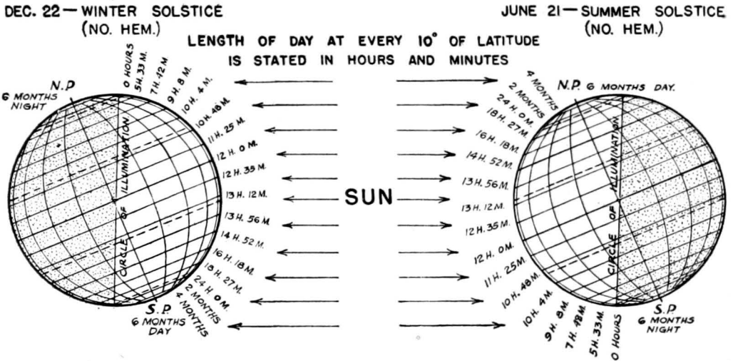
FIG. 15.—On the equinoxes, when the sun's vertical rays are at the equator, the circle of illumination cuts all the parallels in half, and days and nights are equal in length over the entire earth. At this time insolation decreases regularly from equator to poles. At the times of the solstices the sun's vertical rays have reached their greatest poleward migration. The circle of illumination cuts all the parallels (except the equator) unequally so that days and nights are unequal in length except at latitude 0°.
