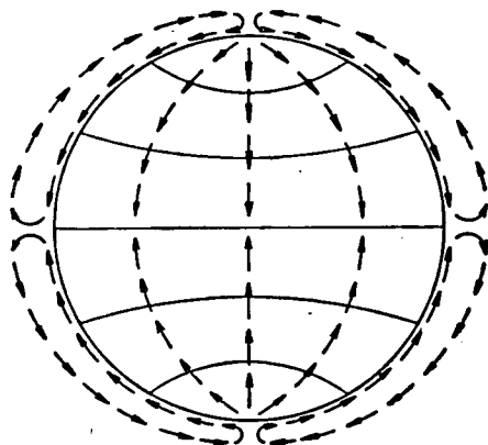
FIG. 34.—System of winds as it might develop on a homogeneous nonrotating earth with the maximum solar energy received at the equator.
