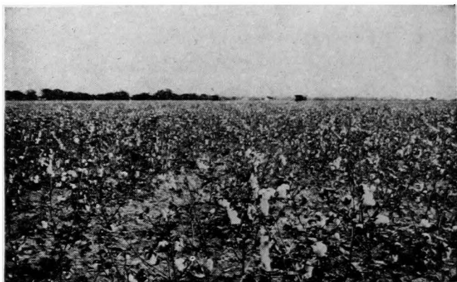
FIG. 138.—Flat but well-drained coastal plain in Texas.
