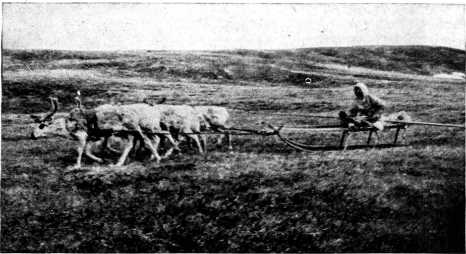
FIG. 316.—Moss tundra in summer along the lower Yenisei River in western Siberia. (Photograph by H. U. Hall, courtesy of the Geographical Review , published by the American Geographical Society of New York. )
