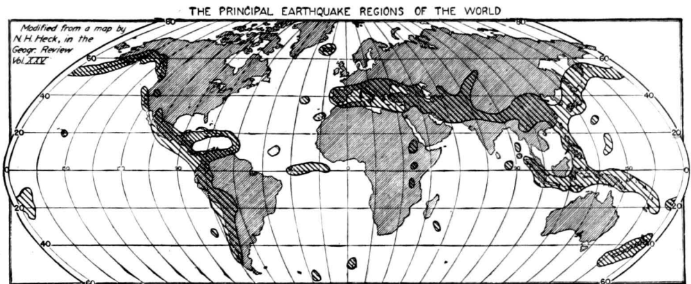
FIG. 123.—(Denoyer's Semielliptical Projection.)
