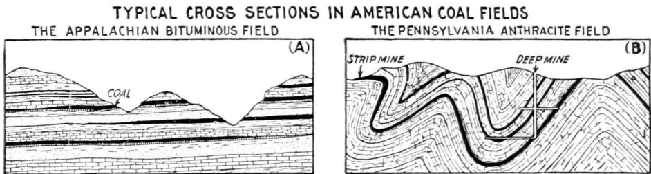
FIG. 328.—Diagrams to show in contrast the common relationships of surface and structure in the bituminous and anthracite fields of the Appalachian coal regions.
