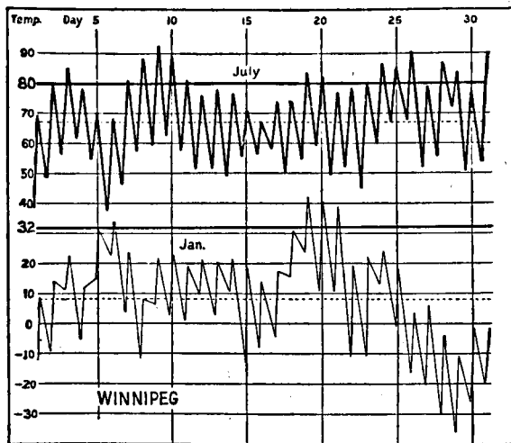
FIG. 104.—Daily maximum and minimum temperatures for the extreme months at a representative station in humid continental climate with short summers. (Courtesy of Mark Jefferson and the Geographical Review .)
