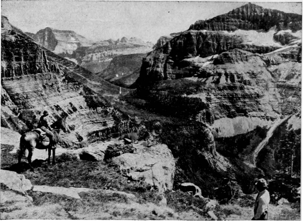
FIG. 261.—Brown Pass, in Glacier National Park, viewed from a higher one. The saddle shape of this notch is distinct. The white arrow point touches the crest of the pass, which also is a part of the continental divide. ( National Park Service, U. S. Department of the Interior. )
