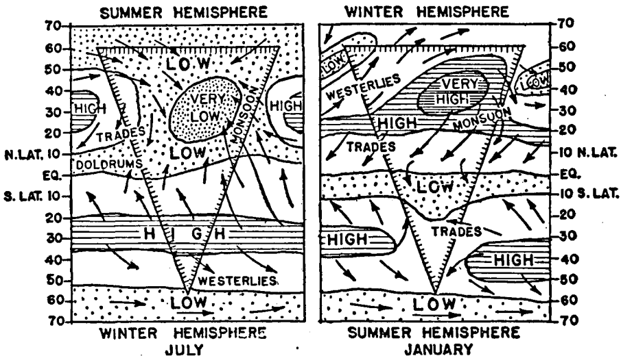
FIG. 31.—Seasonal pressure and wind systems as modified by land and water areas. The triangle represents a landmass. (Modified from Kendrew and Hettner.)
