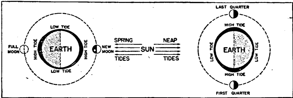
FIG. 227.—A diagram to illustrate the relation of the moon in its different phases and of the sun to the occurrence of ocean tides.
