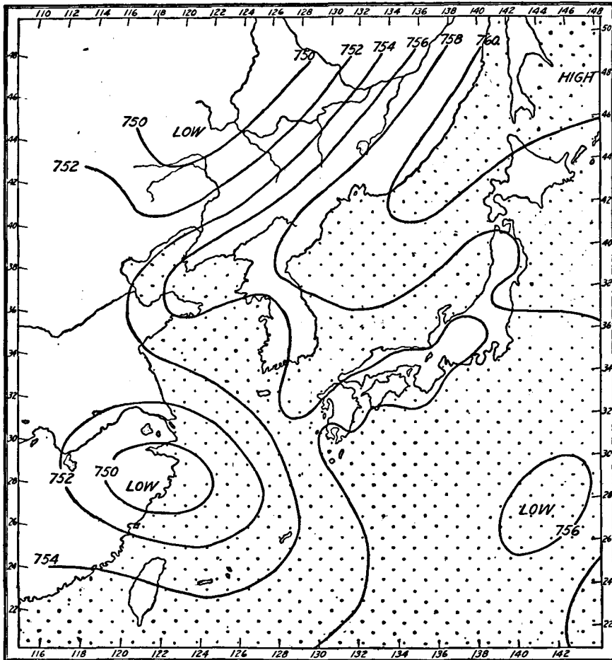
FIG. 64.—A weak summer low emerging from the Yangtze Valley. This type of storm is common in the wet tropics, and in the humid subtropics as well during the summer season. Pressure in mm. From the Japanese weather map, 6 p.m., June 21, 1927.
