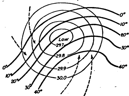
FIG. 58.—Characteristic arrangement of isotherms in a winter cyclone over central and eastern United States. The front is usually warmer than the rear.
