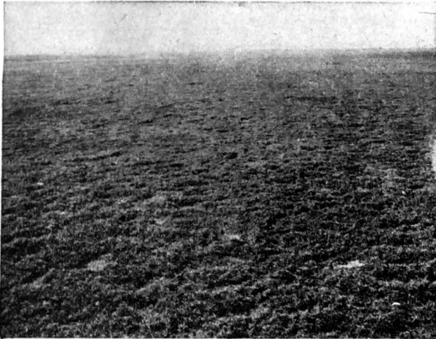
FIG. 311.—Short-grass steppe, Colorado. ( U. S. Department of Agriculture. )
