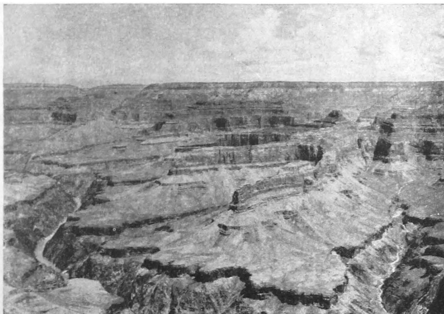
FIG. 230.—The Grand Canyon of the Colorado River. The narrow inner gorge, cut in crystalline rock, is in striking contrast with the intricately carved steps eroded in the sedimentary rocks above. Note the flatness of the distant plateau surface.
