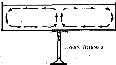
FIG. 17.—Representation of a convectional circulation.
