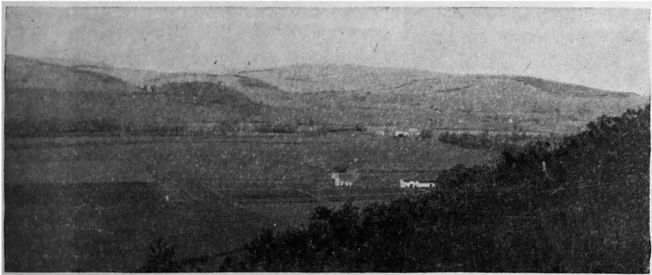
FIG. 249.—A valley in the glaciated hill region near the Finger Lakes of western New York. The hills are ice scoured, but the flat valley floor is deeply underlain by drift.
