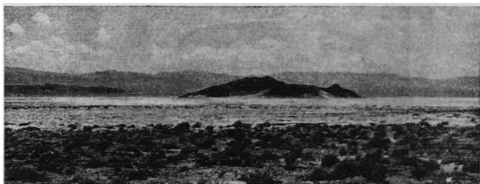
FIG. 207.—A playa basin in Nevada. Its deep alluvial filling has a glistening white crust of salt, and wind-blown salt clings to the rocky island included within it. (Photograph by John C. Weaver.)
