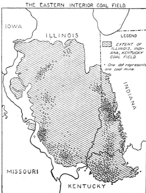
FIG. 333.—Most of the coal mines in the synclinal Eastern Interior Field are located upon its shallower margins.
