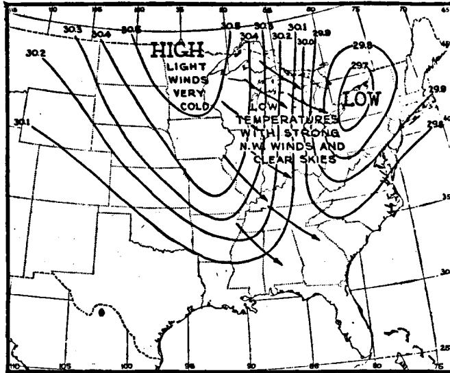
FIG. 57A.—A winter anticyclone advancing southeastward as a mass of cold polar air.
