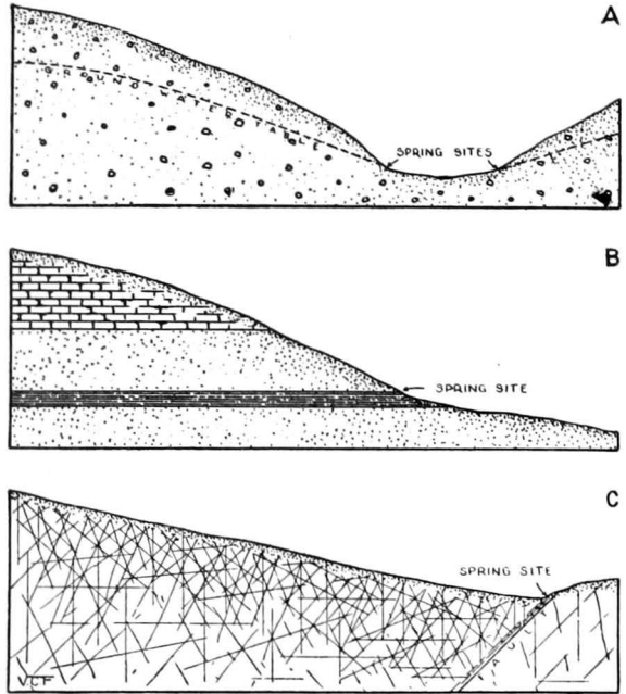
FIG. 275.—Diagrams to illustrate some of the many possible conditions of surface, material, and structure that are related to the occurrence of springs.
