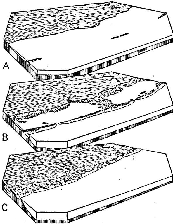
FIG. 220.—Diagrams illustrating stages in the development of an offshore bar on a shore of low relief and shallow water. (A) The beginning of a submarine ridge by wave deposition near the line of breakers; (B) the growth of an offshore bar flanked by lagoons; (C) under wave pounding the bar migrates shoreward and the lagoons narrow, fill, or disappear.
