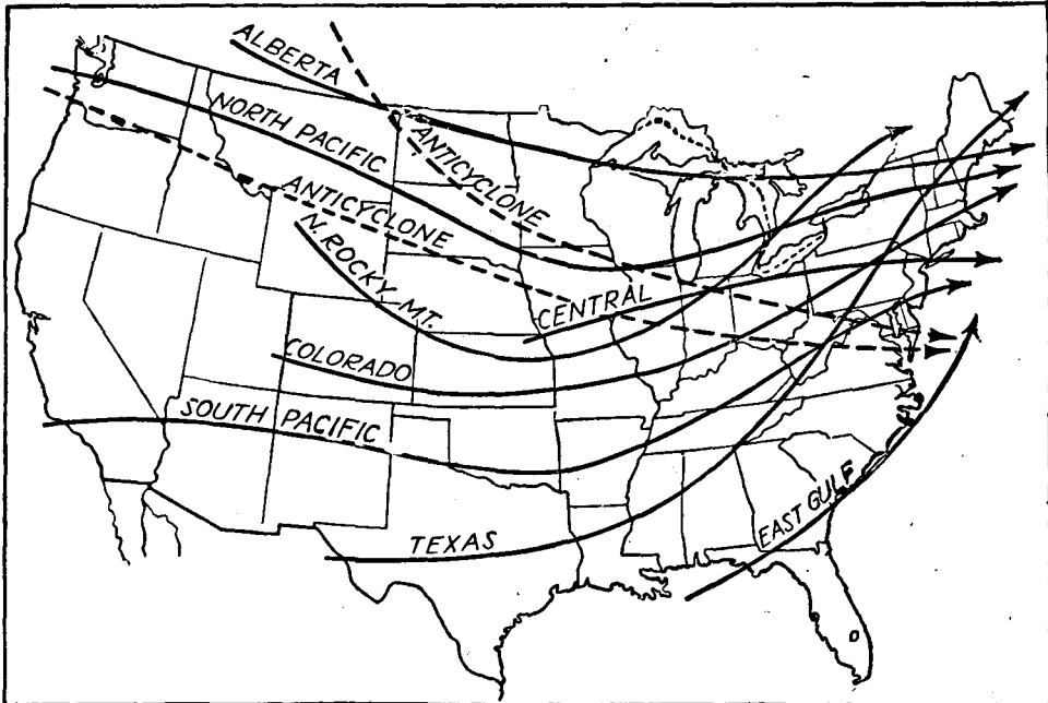
FIG. 62.—Solid lines show principal tracks of cyclones; broken lines are the principal tracks of anticyclones. Note how the cyclone tracks converge on the northeastern part of the United States. Anticyclones moving south from northern Canada ( Pc air) bring severe cold in winter; those from the Pacific northwest ( Pp air) bring only moderate cold.
