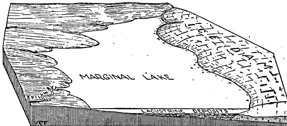
FIG. 199.—A diagram to illustrate the formation of a temporary lake between the margin of a glacier and a low divide across which the surplus drainage escapes. Glacio-lacustrine deposits are seen in the lake bottom.
