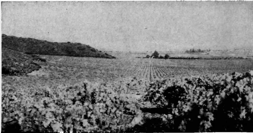
FIG. 173.—A profile view of a series of alluvial fans merged into a small piedmont alluvial plain which borders low mountains in the San Fernando Valley, California. The steeper upper slope of one fan, seen at the left center where it heads between the mountain spurs, may be contrasted with its more gentle lower slope toward the right.
