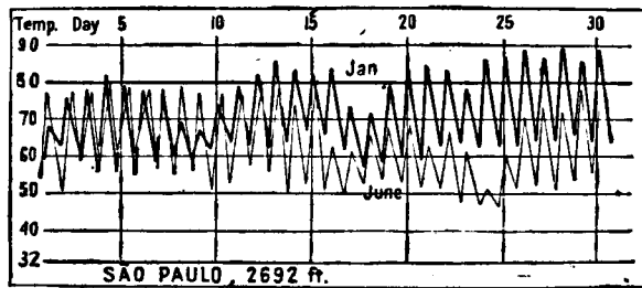
FIG. 78.—Daily maximum and minimum temperatures for the extreme months at an upland savanna station on the Brazilian Plateau. (Courtesy of Mark Jefferson and the Geographical Review .)
