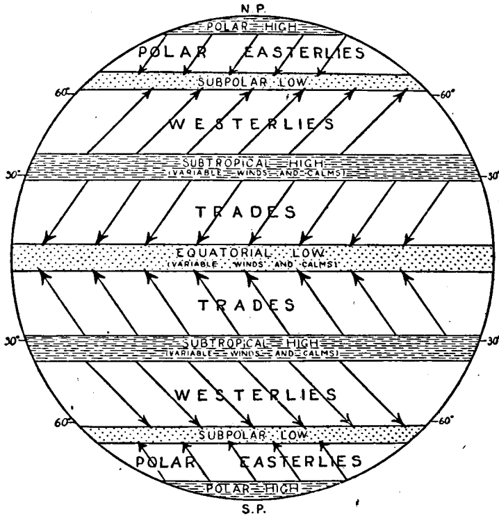
FIG. 27.—A very diagrammatic representation of pressure and wind arrangements as they might appear on an earth with a homogeneous surface.
