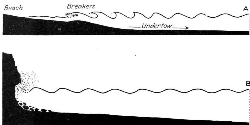
FIG. 135.—Diagrams to illustrate wave forms and action in both shallow and deep shore waters. (A) Waves drag in shallow water, change form, topple, and break some distance from shore. (B) In deep water they break directly on shore.
