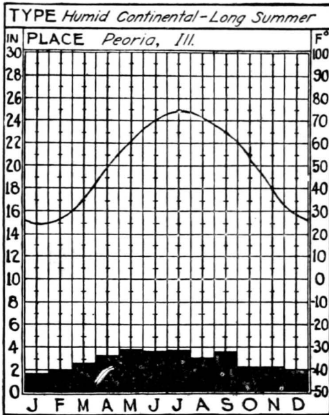
FIG. 100.—Average monthly temperatures and precipitation for a representative station in humid continental climate with long summer.
