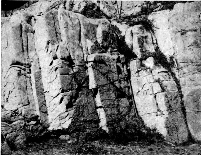
FIG. 113.—Jointing in granite. Joint planes commonly occur in sets all the members of which trend in the same direction. The sets may be vertical, inclined, or horizontal. ( U. S. Geological Survey Photograph. )
