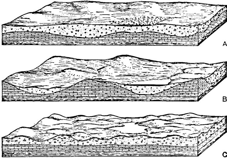
FIG. 180.—Different effects of glacial deposits upon previous rock surfaces. ( A ) A hilly rock surface made more smooth by drift; ( B ) a rock surface of considerable relief partly buried by drift; a rock-controlled drift surface; ( C ) a smooth rock surface made irregular by the deposition of rough moraine.
