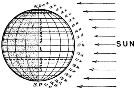
FIG. 15.—On the equinoxes, when the sun's vertical rays are at the equator, the circle of illumination cuts all the parallels in half, and days and nights are equal in length over the entire earth. At this time insolation decreases regularly from equator to poles. At the times of the solstices the sun's vertical rays have reached their greatest poleward migration. The circle of illumination cuts all the parallels (except the equator) unequally so that days and nights are unequal in length except at latitude 0°.
