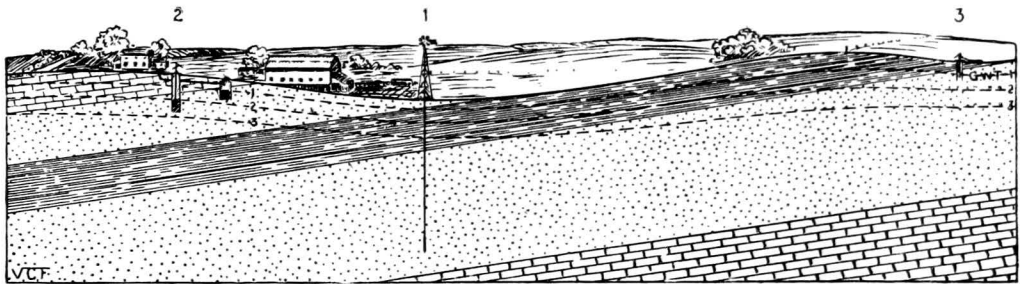
FIG. 279.—Well No. 2 is higher than No. 1 and appears to be a safer water supply but, in fact, it is not so because of the rock structures concerned. The stippled horizons indicate porous, water-bearing formations. The dashed lines show positions of the ground-water table; 1, in wet seasons; 2, ordinary level; 3, in dry seasons.
