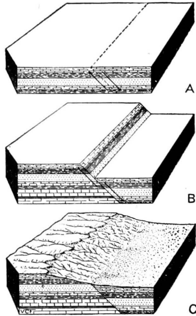
FIG. 114.—Diagram to show the development of a tensional fault in sedimentary rock. (A) The strata before faulting; (B) fault, showing direction of displacement and the fault scarp; (C) the reduction of the fault scarp by erosion to a dissected fault-line scarp.
