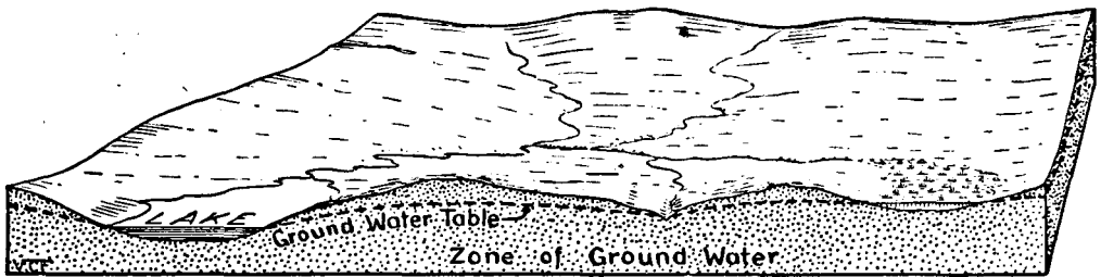
FIG. 125.—A diagram to illustrate the undulating surface of a ground-water table and its relation to the land-relief and drainage features.
