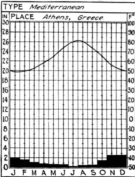
FIG. 86.—Average monthly temperatures and precipitation for a representative station with Mediterranean climate.
