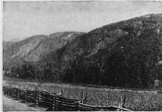
FIG. 244.—Rounded forms resulting from weathering and erosion in massive granites. A valley in the crystalline Appalachians of North Carolina. ( U. S. Geological Survey Photograph. )
