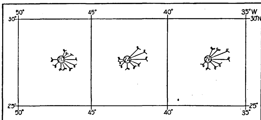
FIG. 38.—The subtropical "belt" of variable winds and calms, or horse latitudes, over the North Atlantic Ocean, June, 1922. For explanation of symbols see Fig. 37. ( U. S. Hydrographic Office Pilot Chart. )
