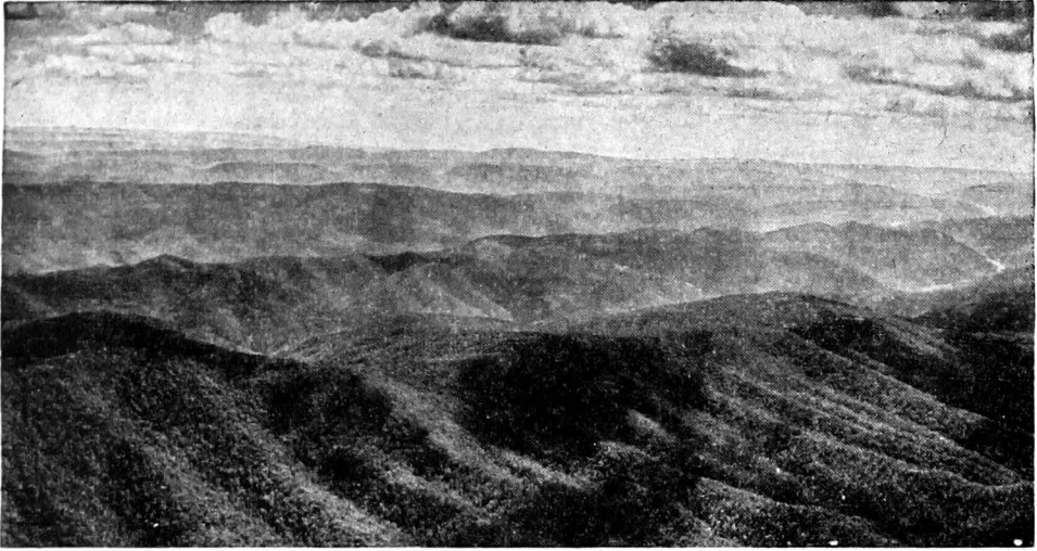
FIG. 240.—A view across the parallel ridges and valleys of one section of the folded Appalachians. Water gaps cut two of the ridges at the extreme right. In many parts of the ridge-and-valley region the valleys are much wider than those shown here and contain large areas of farm land (see Fig. 242). (Photograph by Fairchild Aerial Surveys, Inc.)
