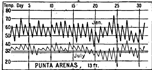
FIG. 98.—Daily maximum and minimum temperatures for the extreme months at a cool marine station in extreme southern Chile. The average temperature of the warmest month at Magallanes (Punta Arenas) is about 50°, but since its average annual temperature is above 32° it is scarcely genuine tundra. (Courtesy of Mark Jefferson and the Geographical Review .)
