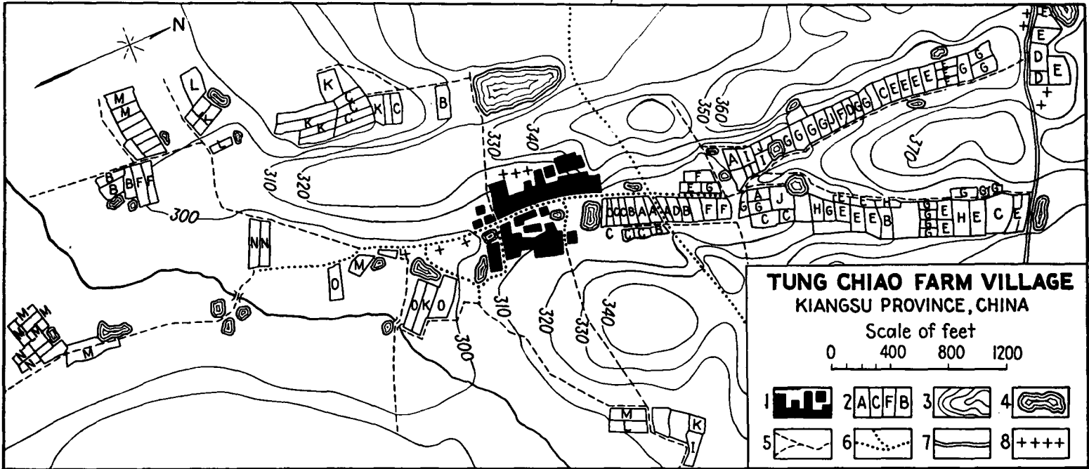
FIG. 380.—A representative Chinese rural village and its associated fields. (1) The village. (2) Field plots; all marked A are tilled by Farmer A ; those marked B by Farmer B , etc. (3) Hill lands, usually in grass and graves; contour figures are in feet. (4) Ponds for irrigation and fish. (5) Earth paths. (6) Paths paved with stone slabs. (7) Paved road seven feet wide. (8) Buddhist temples. (Original map by John L. Buck. From Jones, "Economic Geography," by permission of The Macmillan Company.)
