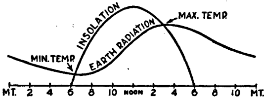
FIG. 18.—Representation of incoming solar radiation and outgoing earth radiation for a period of 24 hr. at about the time of an equinox.
