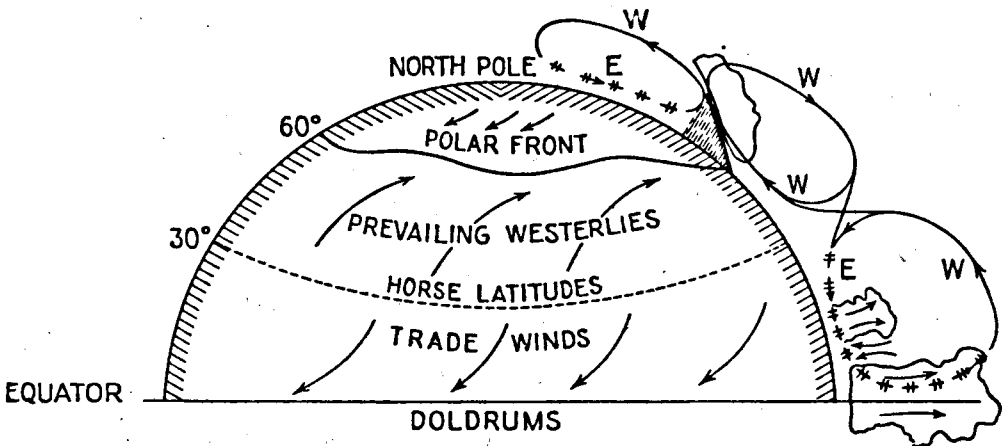
FIG. 36.—General zonal circulation of the atmosphere on a rotating earth with a homogeneous surface. (After Rossby.)
