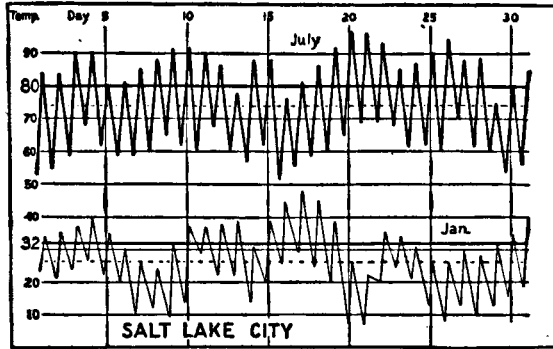
FIG. 84.—Daily maximum and minimum temperatures for the extreme months at a representative middle-latitude steppe station. (Courtesy of Mark Jefferson and the Geographical Review .)
