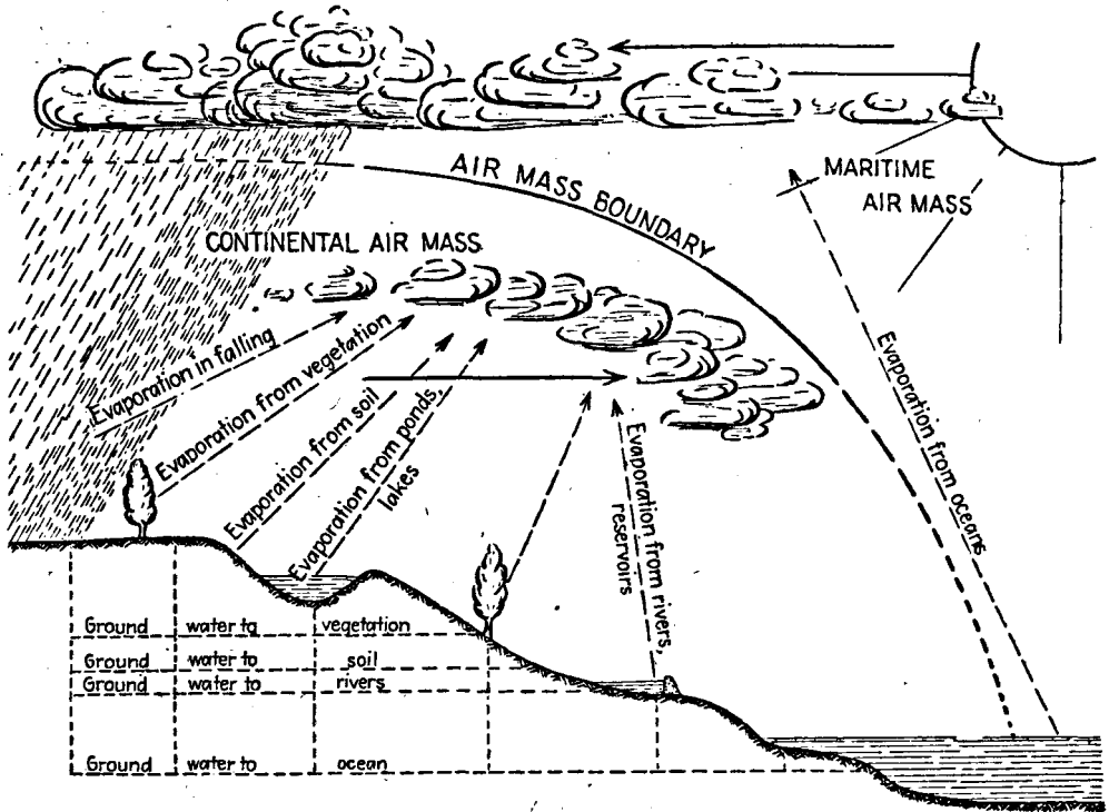
FIG. 45.—The hydrologic cycle correlated with the air-mass cycle. (After Holzman; courtesy of George Jenkins and the Journal of Geography .)
