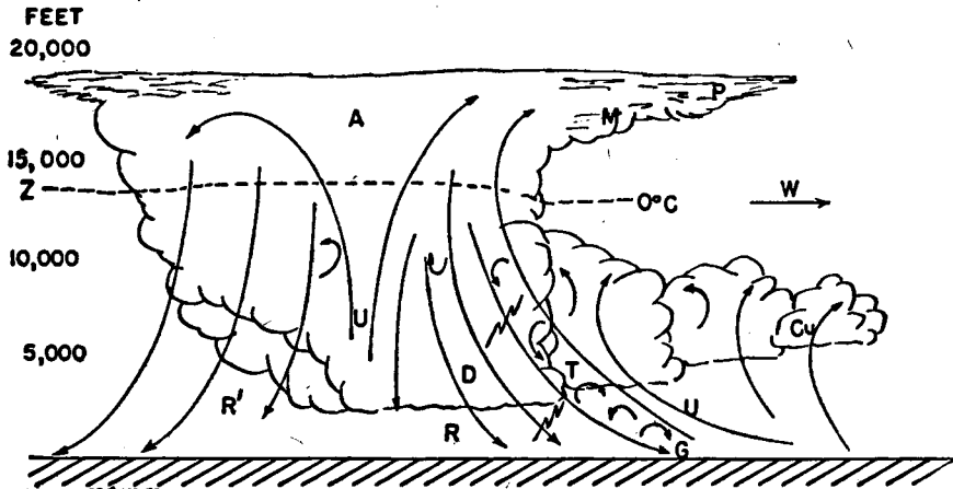
FIG. 65.—Vertical section through a local heat thunderstorm. (A) anvil top of cumulo-nimbus cloud; (C) roll cloud; (Cu) advance cumulus cloud; (D) descending air; (G) strong gusts; (M) mammato-cumulus; (P) protruding portion of anvil cloud; (R) primary rain or hail area; (R') secondary rain; (T) severe turbulence; (U) updraft; (W) wind direction; (w) zero isotherm (centigrade) or freezing level. (From Haynes.)
