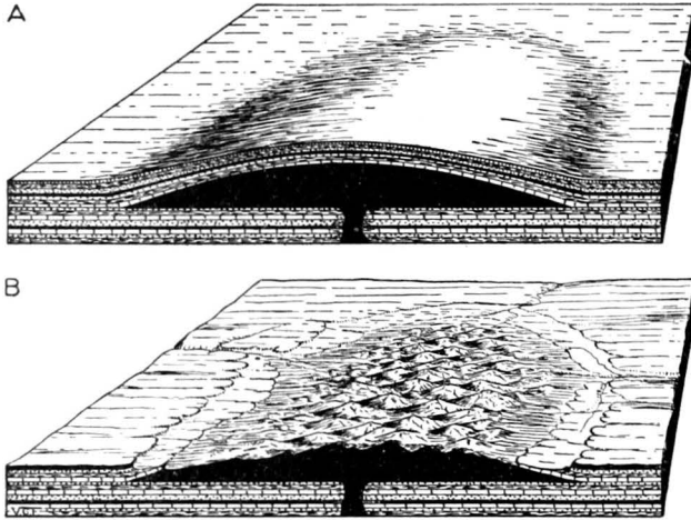
FIG. 121.—A diagram to illustrate the effects of the intrusion of a giant laccolithic mass into sedimentary rocks (A), and features resulting from its subsequent erosion by streams (B).
