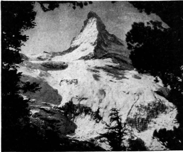
FIG. 268.—The Matterhorn, a roughly quadrangular peak resulting from the headward encroachment of four glaciers. ( Photograph by Ewing Galloway. )
