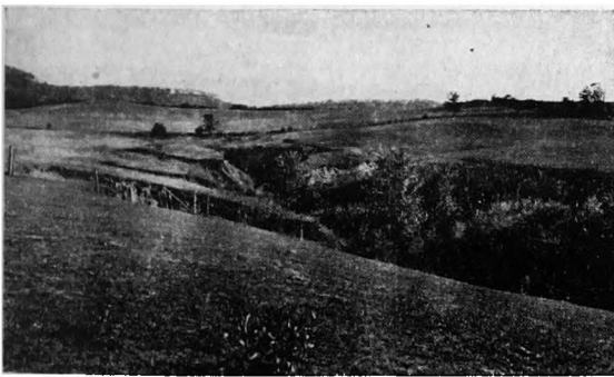
FIG. 128.—As a gully grows in length by headward erosion, tributary gullies branch from its sides and grow in like manner. (Photograph by F. W. Lehmann, C. B. & Q. Railroad Company.)
