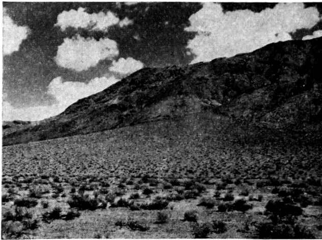
FIG. 133.—The conformation of a small and fairly steep alluvial fan in Nevada. The apex of the fan lies at the mouth of the gully from which the material was eroded. (Photograph by John C. Weaver.)
