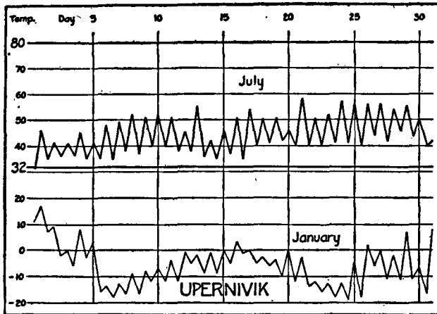
FIG. 109.—Daily maximum and minimum temperatures for the extreme months at a representative tundra station in Greenland.
