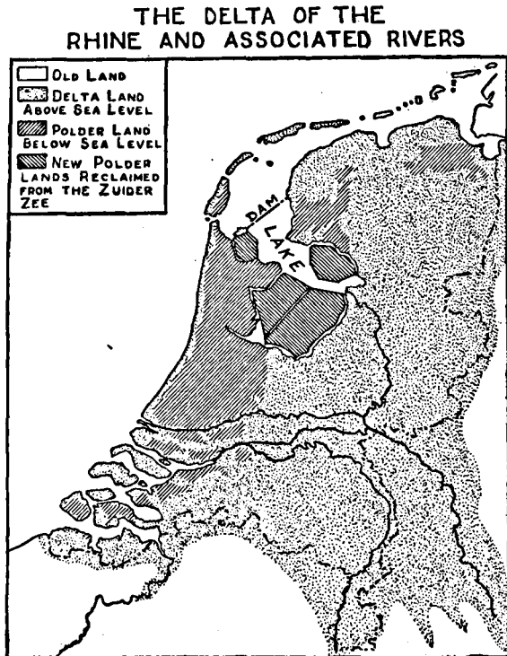
FIG. 161.—The extent of reclaimed land in the Netherlands in relation to the area of the Rhine Delta. (After K. Jansma.)
