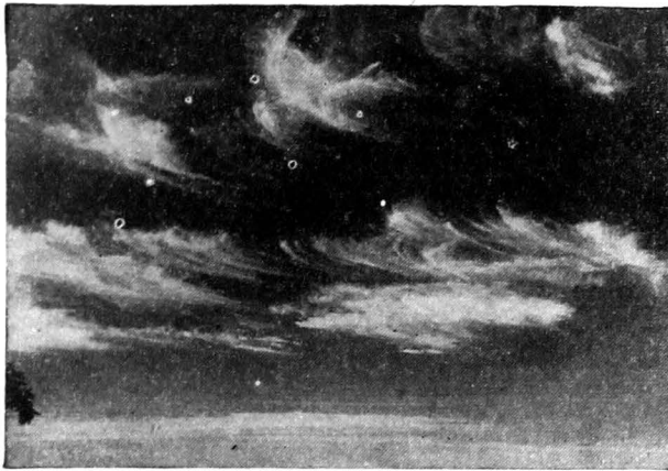
FIG. 48.—Cirrus clouds. ( U. S. Weather Bureau Photograph. )
