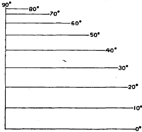
FIG. 3.—The comparative lengths of the radii of the parallels.
