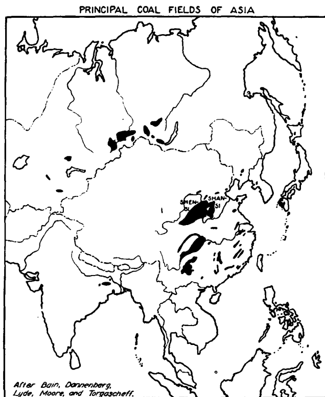
FIG. 336.—The fields of Shensi and Shansi, China, dominate the coal resources of Asia.
