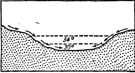
FIG. 22.—Cold air, because it is denser, tends to settle into the valley bottoms. For this reason frost is more prevalent in low places than it is on adjacent slopes.
