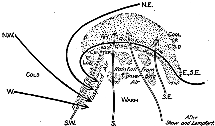
FIG. 55.—Diagrammatic representation of the wind system and rainfall areas (dotted) in a middle-latitude cyclone.
