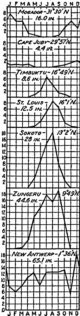
FIG. 77.—Illustrating rainfall regimes in the low latitudes; Africa north of the equator. Stations are arranged according to latitude with Nouvelle Anvers (New Antwerp) closest to the equator.
