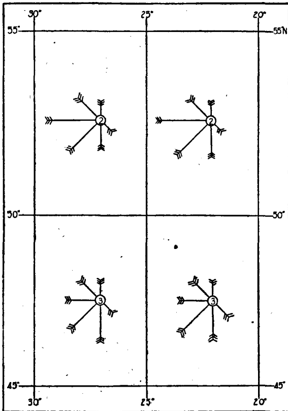
FIG. 39.—The westerlies over the North Atlantic Ocean, January 1922. For explanation of symbols see Fig. 37. ( U. S. Hydrographic Office Pilot Chart. )
