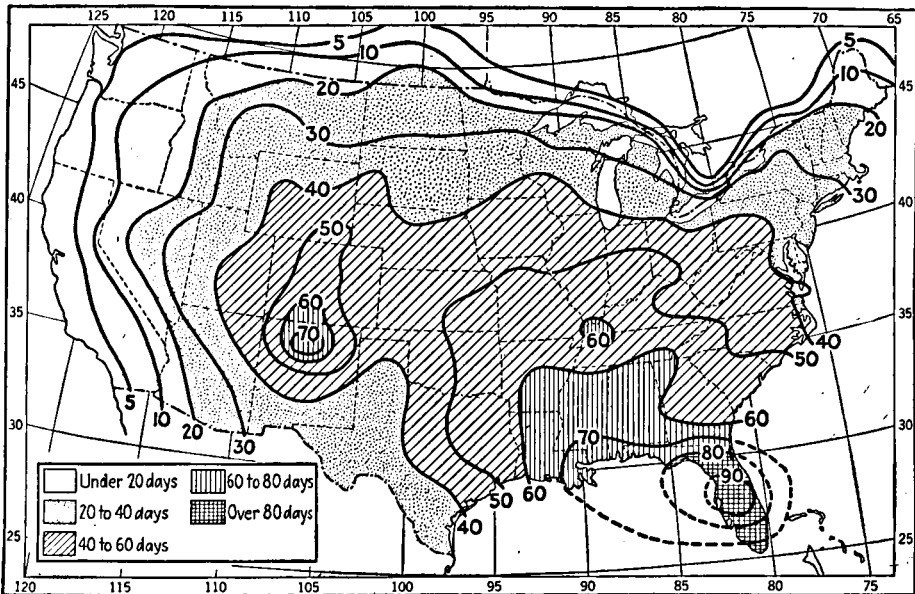
FIG. 68.—Average annual number of days with thunderstorms.
