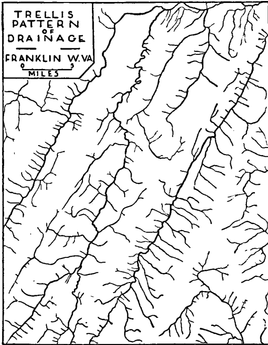
FIG. 242.—The type of drainage pattern developed in association with relief features and rock structures like those shown in Fig. 240.
