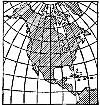
FIG. O.—A polyconic projection.
