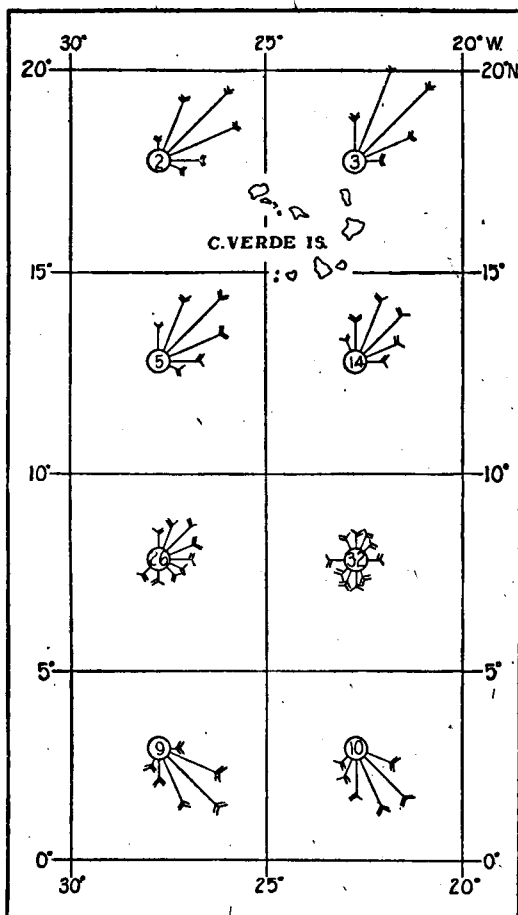
FIG. 37.—Northeast and southeast trades and doldrums over the Atlantic Ocean, June, 1922. The wind rose is given for each 5-degree square. Arrows fly with the wind. The length of the arrow is proportional to the frequency of winds from that direction. The number of feathers on the arrow indicates the average force of the wind on the Beaufort scale. The figure in the center gives the percentage of calms, light airs, and variable winds. (U. S. Hydrographic Office Pilot Chart.)
