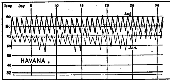
Fig. 76.—Daily maximum and minimum temperatures for the extreme months at a representative savanna station with a marine location. (Courtesy of Mark Jefferson and the Geographical Review.)
