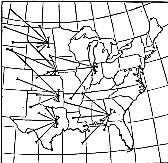
FIG. 43B.—Prevailing direction of upper winds in winter. They are more northwesterly in the cold season. ( U. S. Weather Bureau. )
