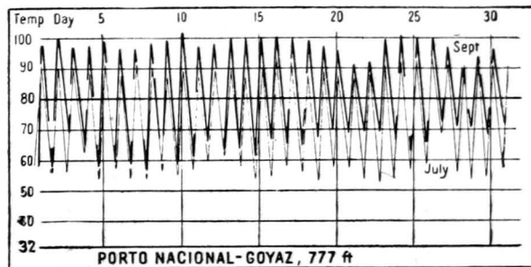
FIG. 75.—Daily maximum and minimum temperatures for the extreme months at a representative savanna station in Brazil. (Courtesy of Mark Jefferson and the Geographical Review .)
