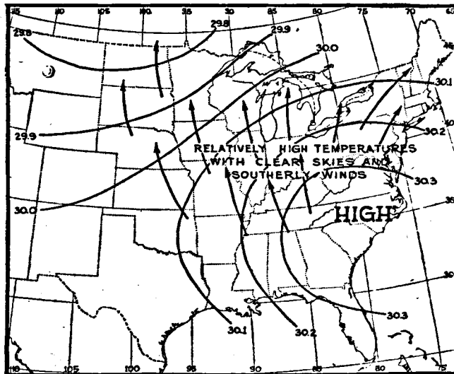
FIG. 57B.—A relatively stagnant anticyclone over southeastern United States producing unseasonably warm weather over the central and eastern parts of the country.
