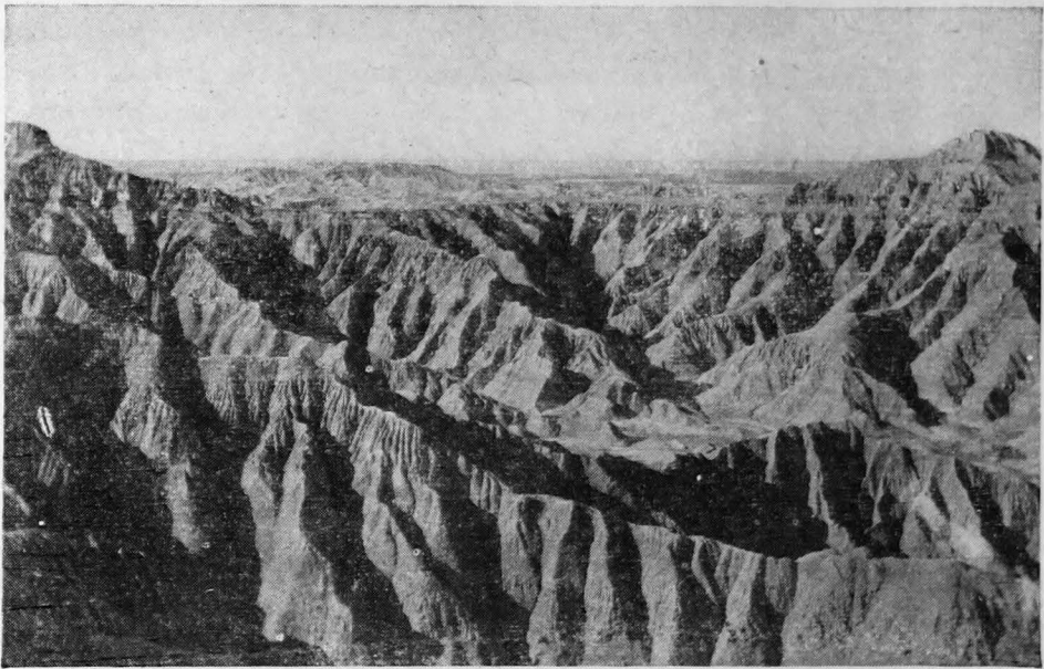
FIG. 239.—The features of badlands in western North Dakota. ( U. S. Geological Survey Photograph. )
