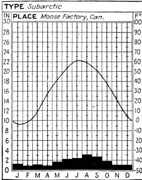
FIG. 105.—Average monthly temperatures and precipitation for a representative subarctic station.
