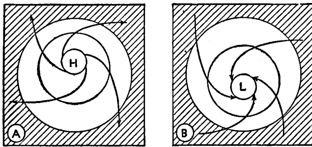
FIG. 40.—Shaded areas represent oceans; white areas are continents. In winter (A) pressure is high over the cold continents, while in summer (B) it is low. The result is an outflow of continental air in winter and an inflow of ocean air in summer. This is a monsoon system. (From Petterssen.)
