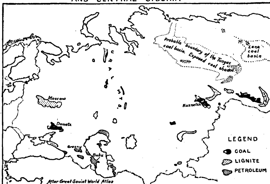
FIG. 343.—The relative importance of the Russian coal and oil fields is as much dependent upon their location as upon their size.
