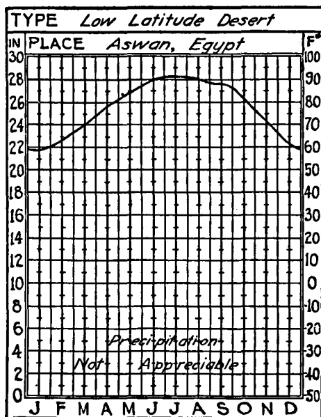
FIG. 80.—Average monthly temperatures at a representative station in a low-latitude desert.
