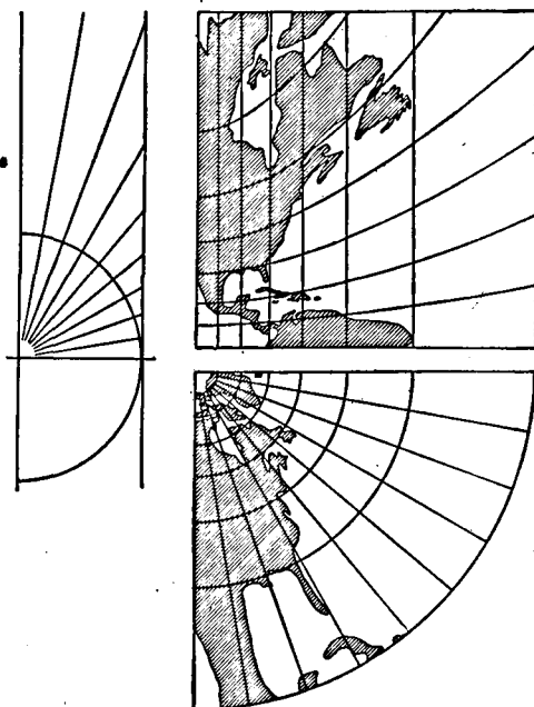
FIG. J.—The gnomonic projection; the manner of obtaining the basic spacings of its grid, and segments of its meridional and polar forms.
