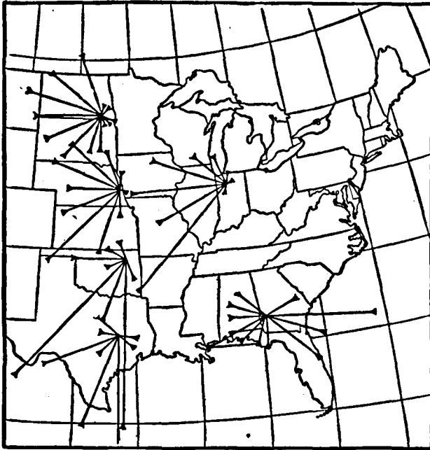
FIG. 43A.—Prevailing direction of upper winds in summer. They are more southwesterly in the warm season. ( U. S. Weather Bureau. )
