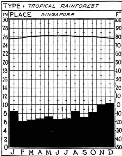
FIG. 70.—Average monthly temperatures and precipitation for a representative tropical rainforest station. Monthly temperatures are much more uniform than monthly precipitation.
