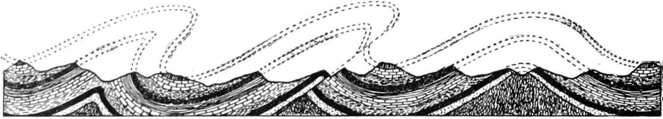
FIG. 118.—Synclinal and anticlinal mountains. The complicated folds and faults of some mountains have been studied and from the eroded remnants which make up the present mountains great structures have been projected. These probably never existed, as such, because they were eroded as they were formed. (See also Fig. 241.)
