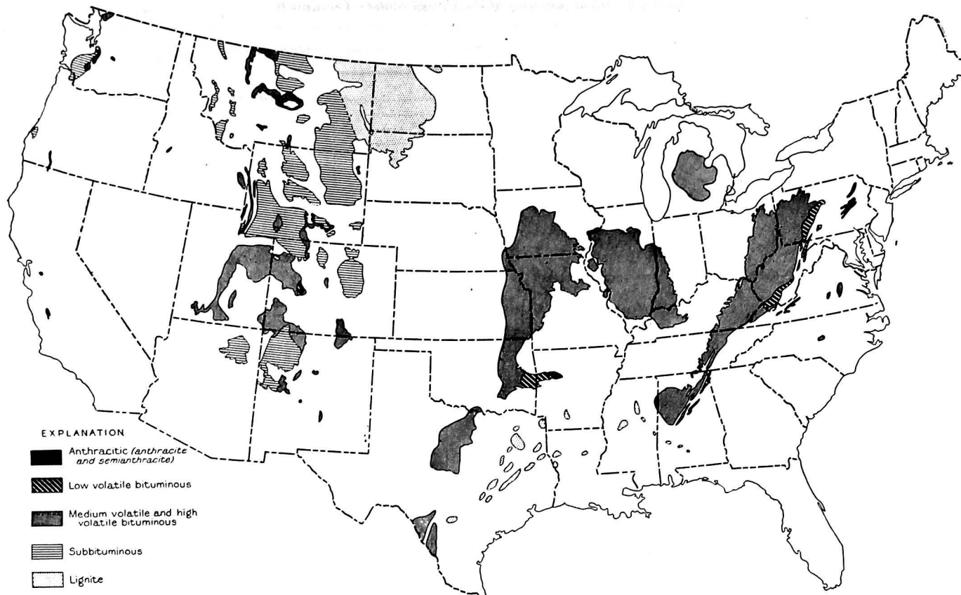
FIGURE 2.—Coal Fields of the United States. Prepared by the Geological Survey, Department of the Interior.
