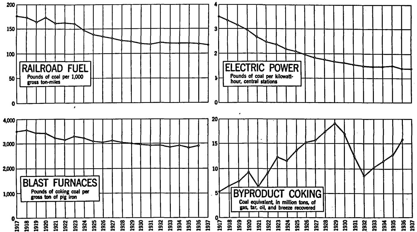
FIGURE 25.—Tendencies in Fuel Efficiency in the United States, 1917–37. (Reproduced from Minerals Yearbook , 1938, p. 716.)
