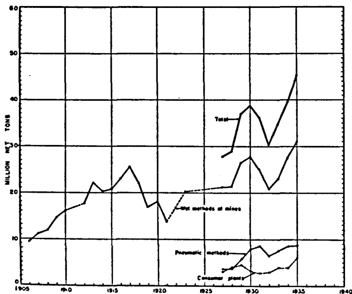
FIGURE 24.—Tonnage of Bituminous Coal Mechanically Cleaned in the United States, 1906-35. (Reproduced from Minerals Yearbook, 1937 , p. 837.)
