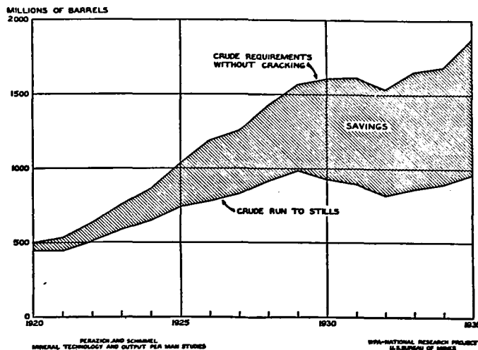
FIGURE 11.—Crude Petroleum Conserved by Use of the Cracking Process.
