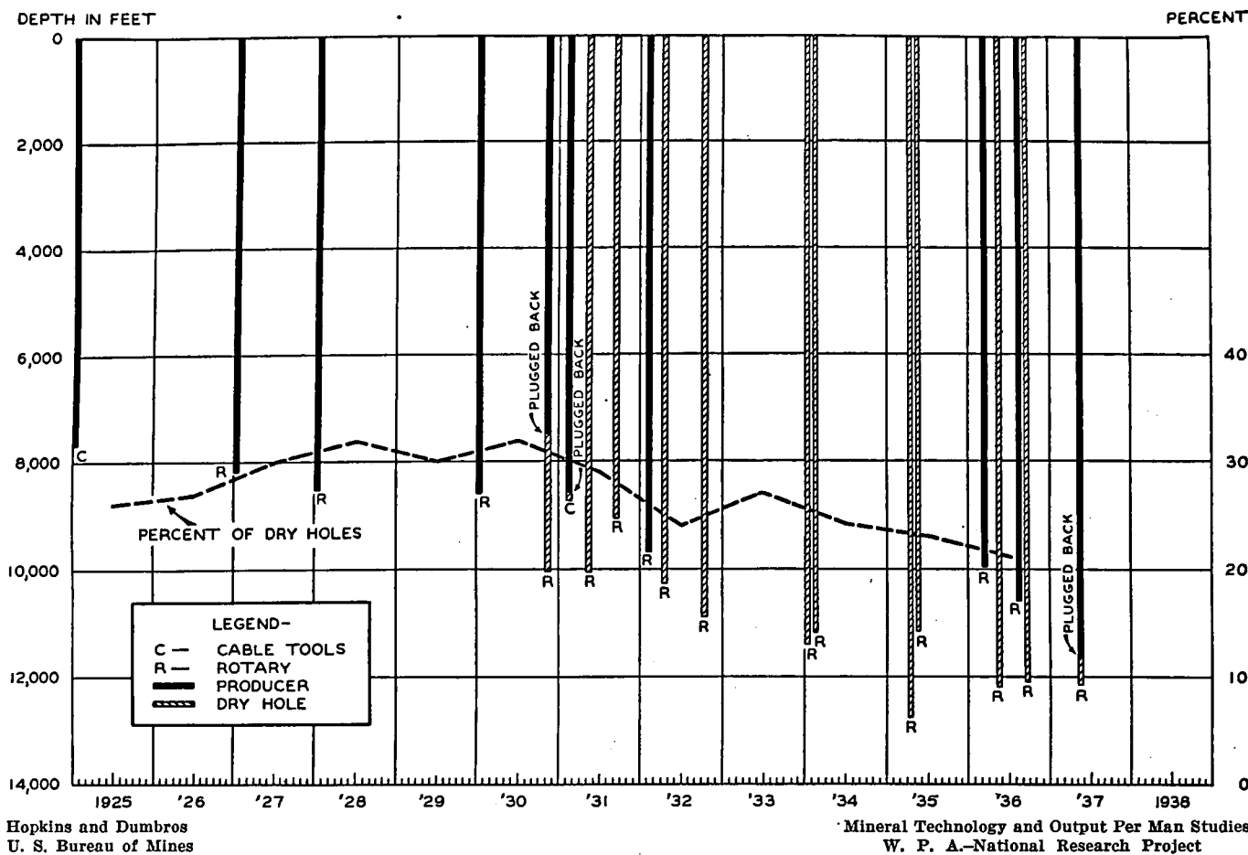
FIGURE 6A.—Record of Increasing Depth of Drilling in the United States, 1925-37.
