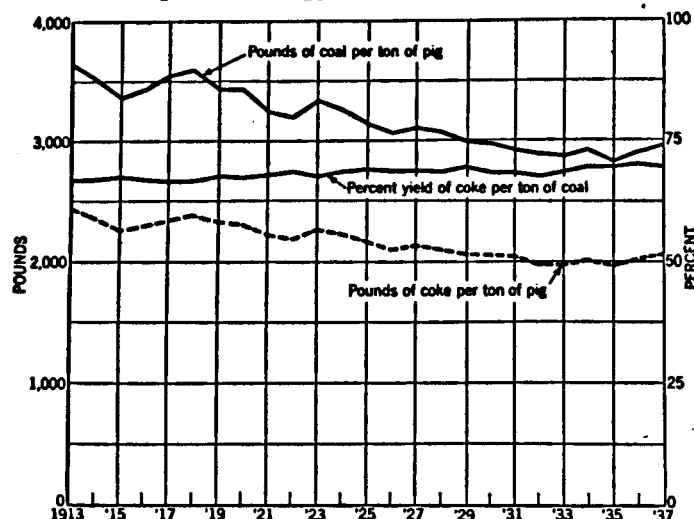
FIGURE 26.—Pounds of Blast-Furnace Coke Consumed Per Gross Ton of Pig Iron, 1913-17. (Reproduced from Minerals Yearbook , 1938, p. 788.)
