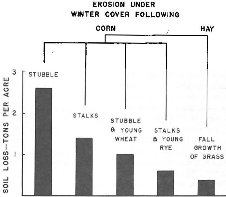
Figure 8.—Effect of cover on erosion after corn harvest on Sept. 29 to soybean seedbed preparation, May 9. Missouri Soil Conservation Experiment Farm, McCredie.
