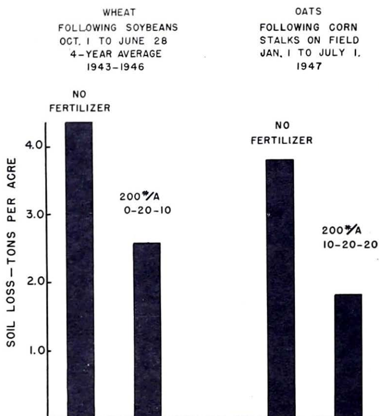
Figure 6.—Effect of fertilizer on erosion under small grain. Missouri Soil Conservation Experiment Farm, McCredie.
