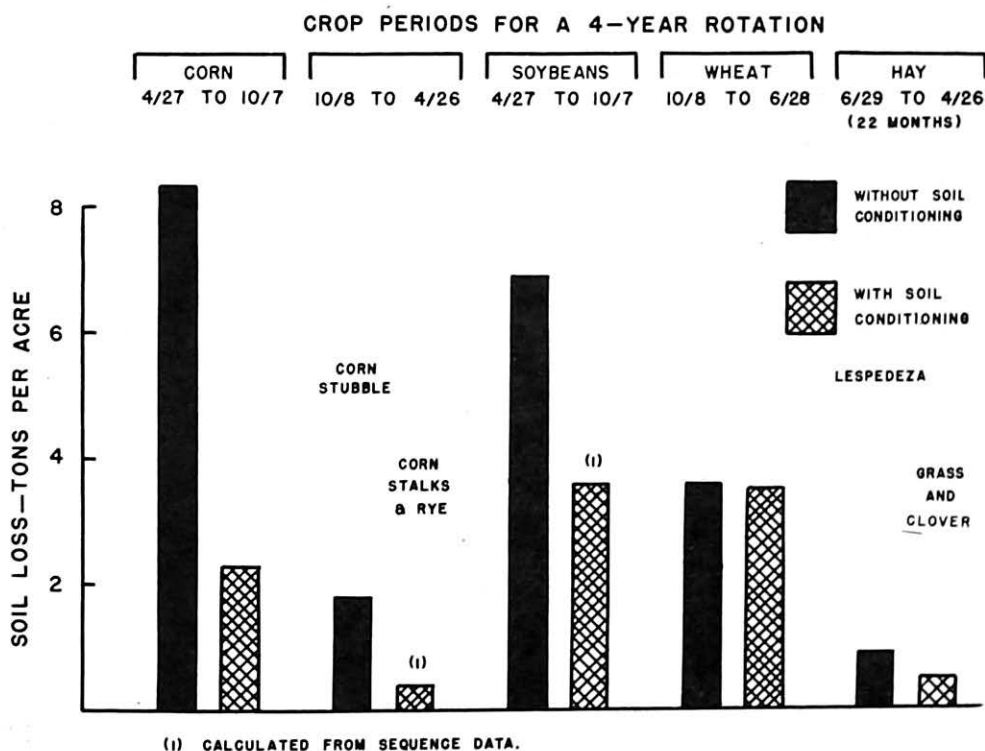
Figure 12.—Erosion losses by crop periods for a 4-year rotation without and with soil conditioning and maximum soil cover. Missouri Soil Conservation Experiment Farm, McCredie, Mo.
