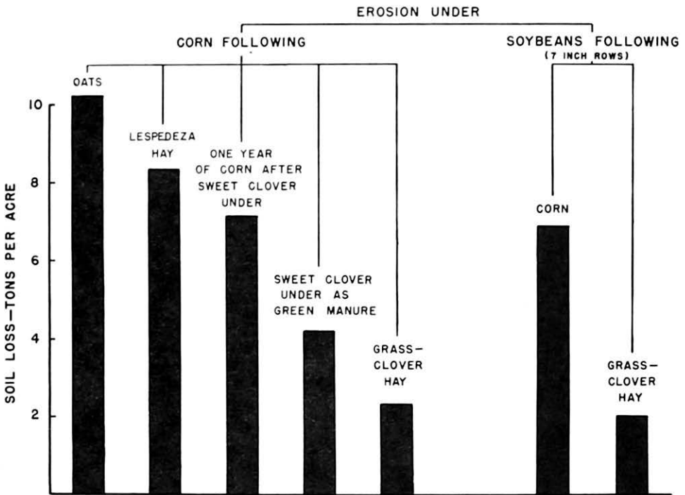
Figure 11.—Effect of preceding crop on erosion under corn and soybeans during the period April 27 to October 7. Missouri Soil Conservation Experiment Farm, McCredie.
