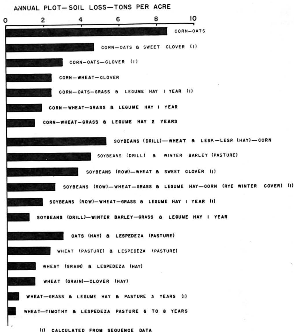
Figure 13.—Erosion under different rotations from small plots on rolling Putnam silt loam soil of 3% slope. Missouri Soil Conservation Experiment Farm, McCredie, Mo.
