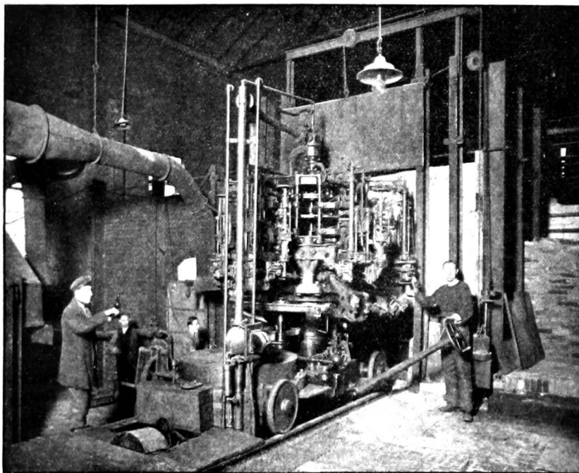
Making bottles by machinery. "Ovens" machine in the Glassworks of Fischmann & Sons, Malý Újezd.
