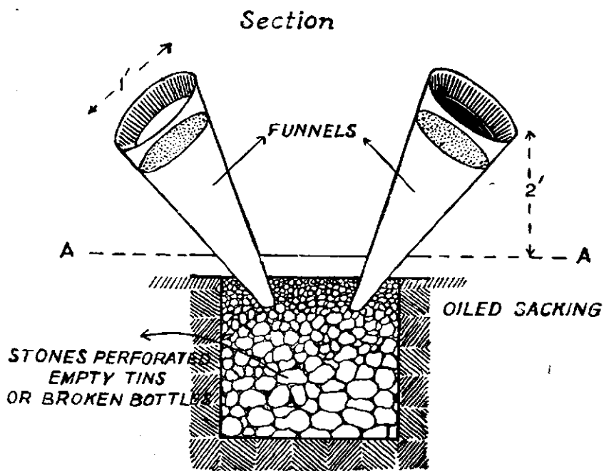
FUNNEL URINE PIT
