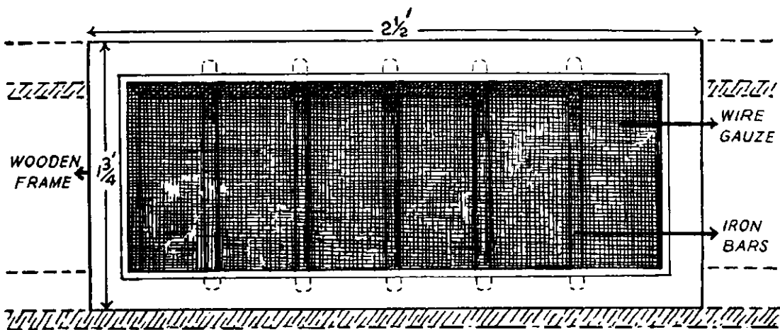
A VENTILATOR DESIGN
