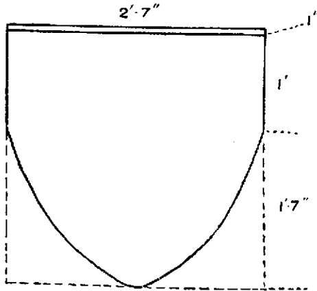
FIG. D. Muslin piece for bag. (Cut two pieces to shape shown and join along curved edges.)
