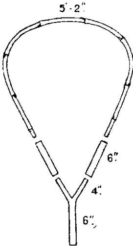
FIG. C. Rough net frame in pieces.
