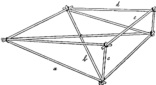
FIG. B. Bamboo frame.
