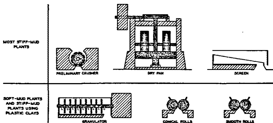
Figure 5.- CLAY PREPARATION
