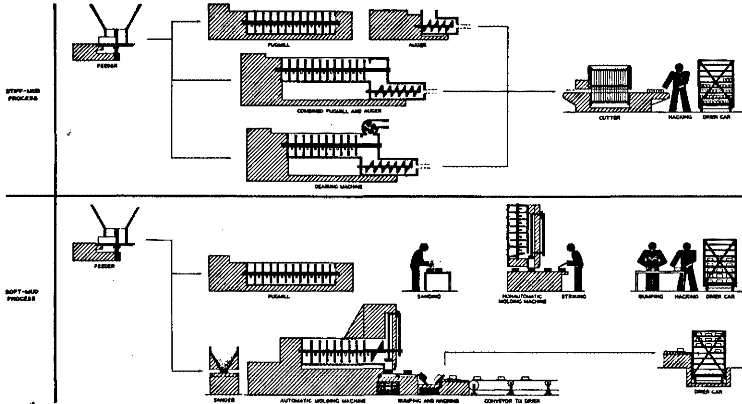
Figure 7.- MACHINE HOUSE
