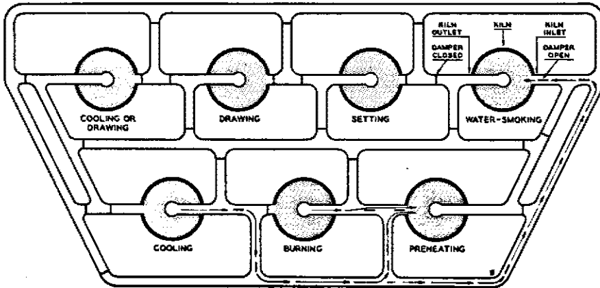
Figure 15.- CONTINUOUS MINTER SYSTEM OF BEEHIVE KILNS
