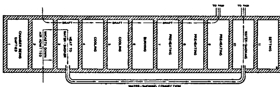
Figure 14.- CONTINUOUS SYSTEM OF RECTANGULAR KILNS
