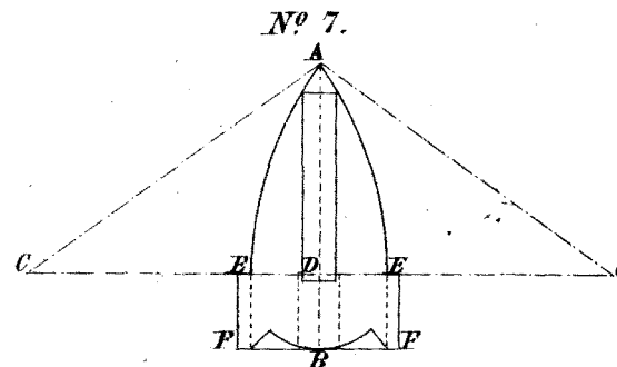
Rifle Shell formed exactly as Ball N° 6, but cast with a deep hole at the smaller end in which is fixed a Copper Tube filled with detonating powder.
