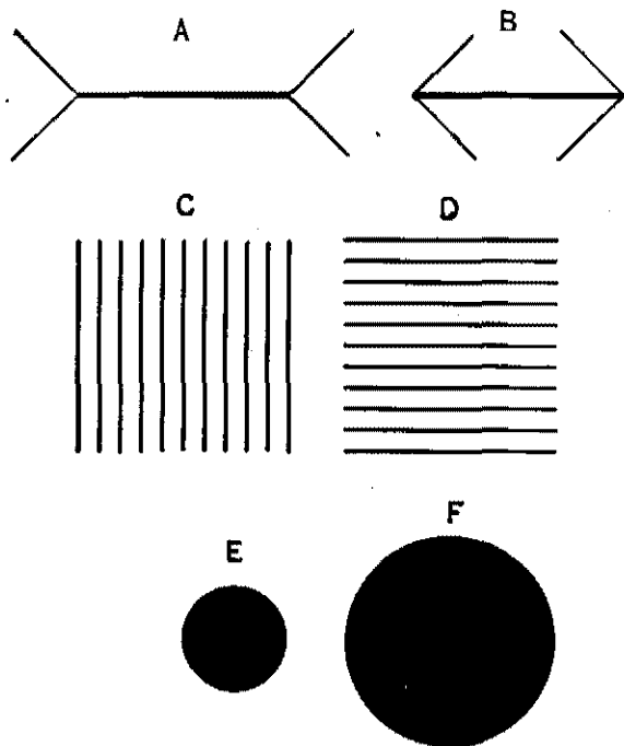
FIG. 9. — Optical Illusions.
