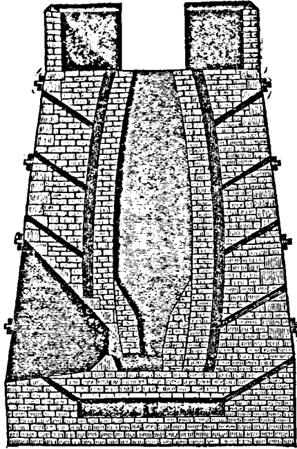
FIG. 8. A NORWEGIAN BLOOMERY FURNACE (Eighteenth century)
