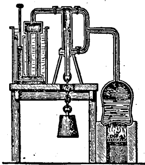
FIG. 11. APPARATUS USED BY WATT IN EXPERIMENTS TO DEMONSTRATE THE ADVANTAGES OF A SEPARATE CONDENSING CHAMBER
