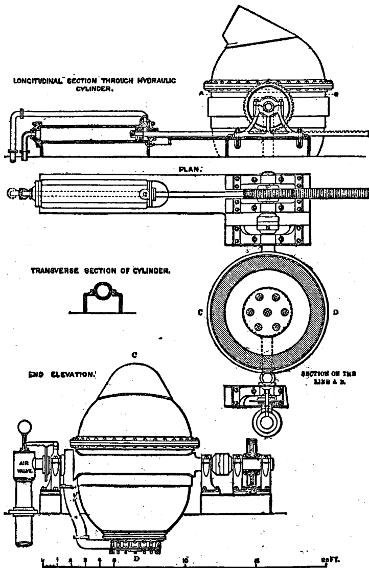
FIG. 16. BESSEMER CONVERTING VESSEL
