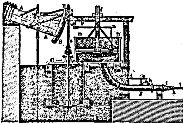
FIG. 10. DEVELOPED CYLINDRICAL BLOWING ENGINE
