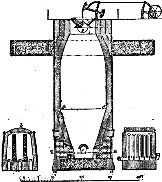
FIG. 9. BLAST FURNACE ( Ebbw Vale, Monmouthshire, 1850-60 )
