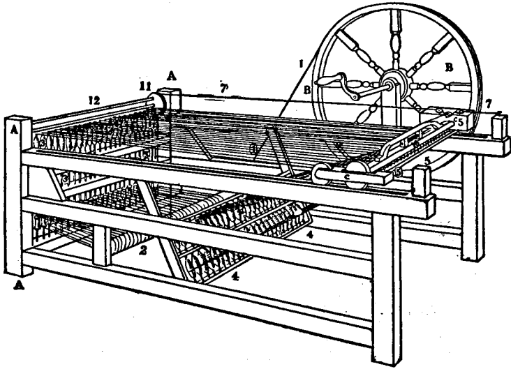
FIG. 3. IMPROVED MODEL OF HARGREAVES'S SPINNING JENNY
