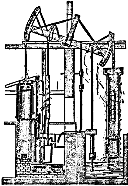
FIG. 12. SECTION OF AN ENGINE SET UP BY WATT AT CHACEWATER IN CORNWALL, 1777 Embodying various improvements over the first model of the engine.
