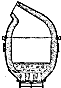
FIG. 17. VERTICAL SECTION OF THE BESSEMER CONVERTER
