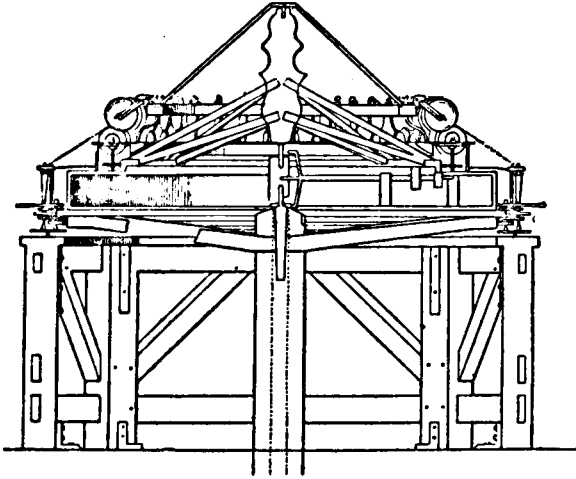
FIG. 2. PAUL'S SPINNING MACHINE, 1758
