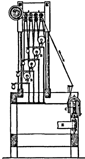
FIG. 1. THE THROSTLE
