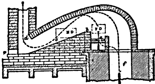
FIG. 13. THE REVERBERATORY FURNACE
