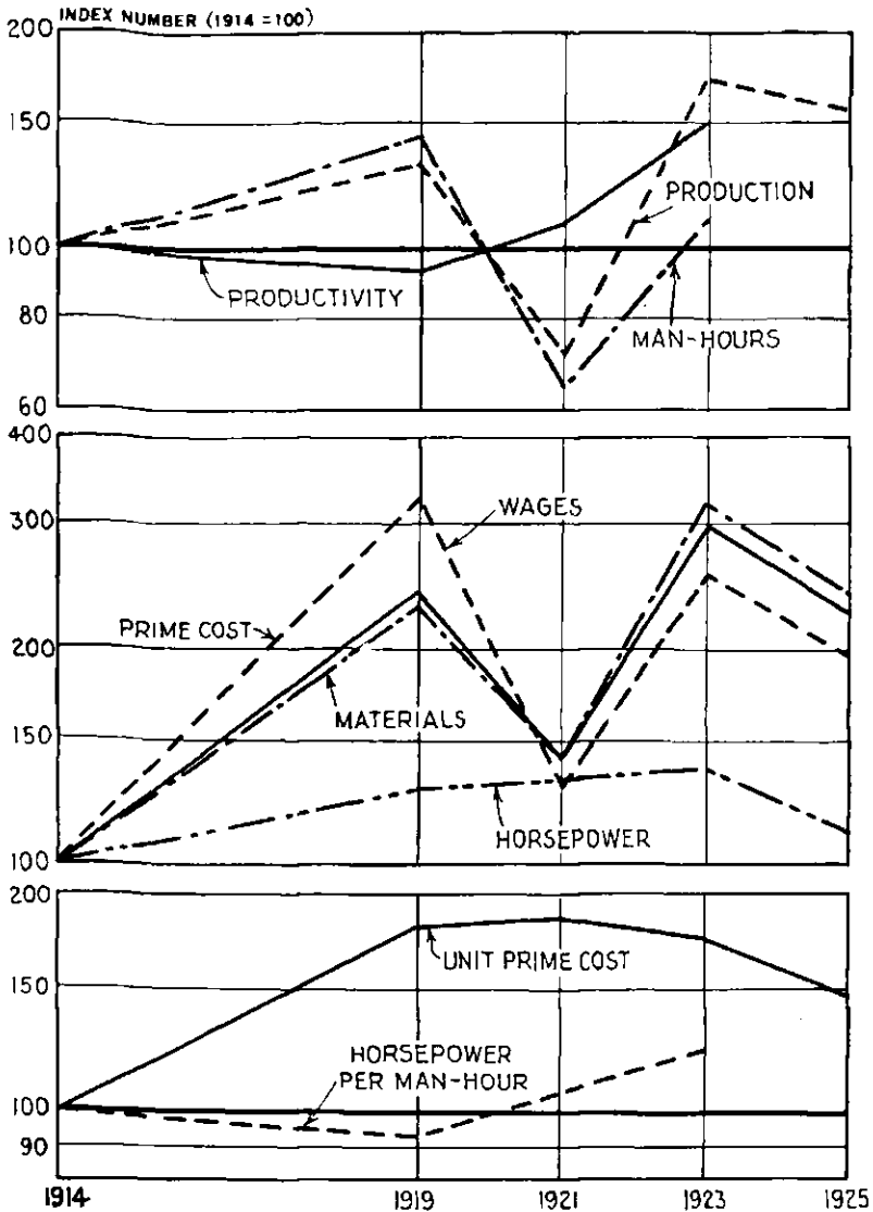
CHART 21.—FLUCTUATIONS IN THE RECORD OF BLAST FURNACE OPERATIONS
