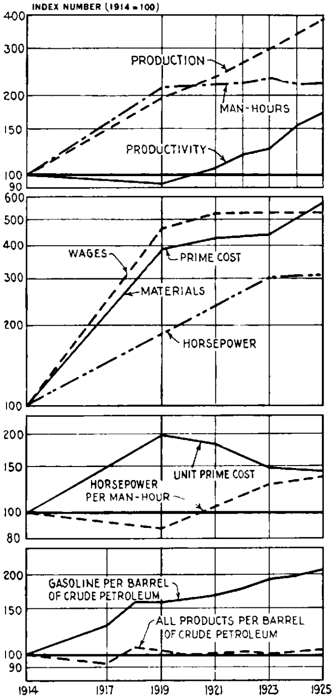
HART 19.—FLUCTUATIONS OF PRODUCTION FACTORS OF THE PETRO-LEUM REFINING INDUSTRY
