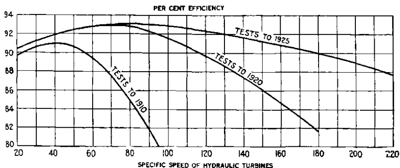
CHART 13.—INFLUENCE OF IMPROVEMENTS IN HYDRAULIC TURBINES ON THEIR EFFICIENCIES AT VARIOUS SPEEDS
