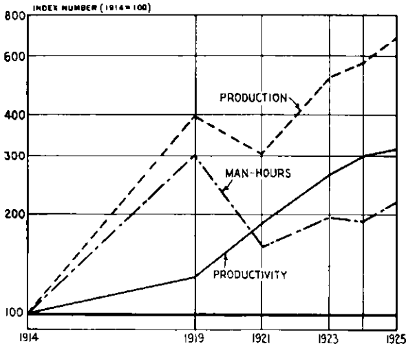
CHART 18.—FLUCTUATION OF PRODUCTION FACTORS OF THE RUBBER TIRE INDUSTRY
