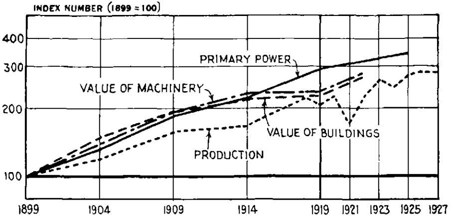
CHART 5.—RELATIONSHIP OF PRIMARY POWER, VALUE OF MANUFACTURING BUILDINGS AND MACHINERY, AND PHYSICAL VOLUME OF PRODUCTION
