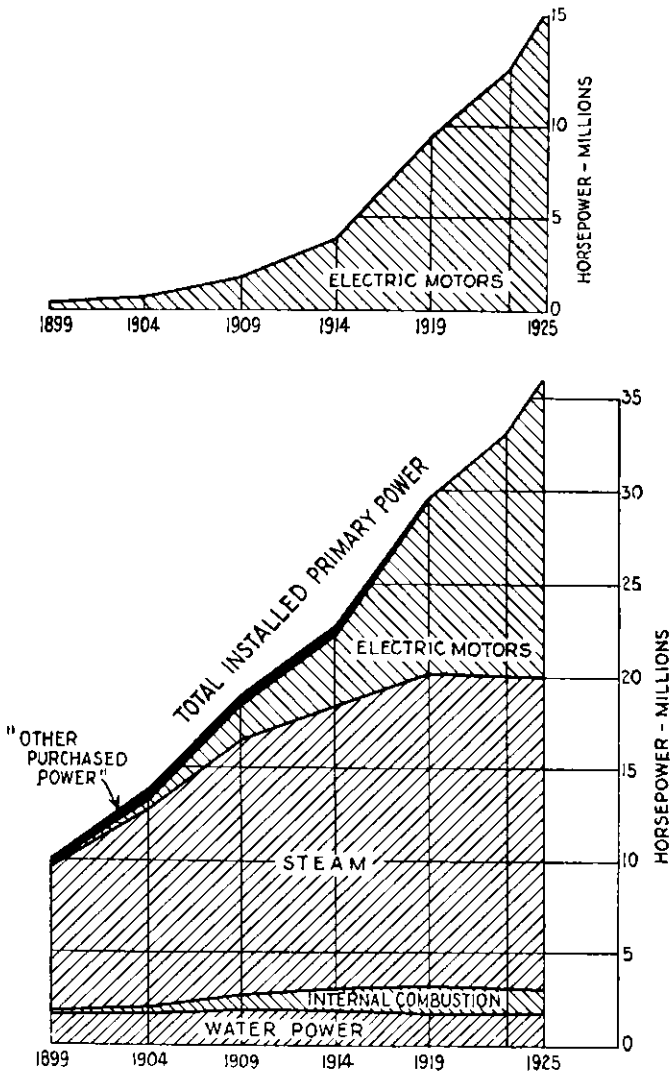
CHART 9.—POWER SUPPLIED BY FOUR KINDS OF PRIME MOVERS
