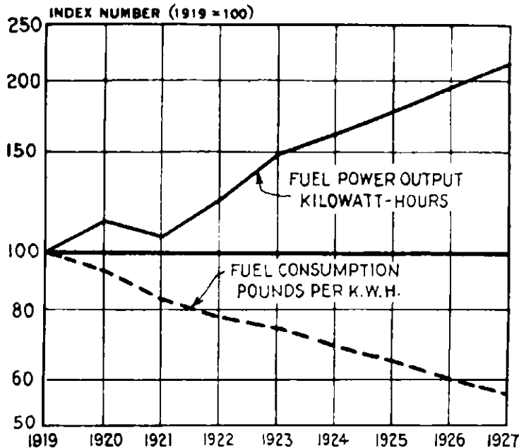
CHART 11.—RELATIONSHIP BETWEEN FUEL CONSUMPTION PER KILOWATT-HOUR AND TOTAL OUTPUT OF ELECTRICAL ENERGY
