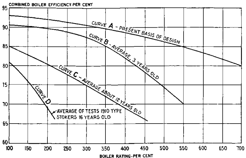
CHART 12.—IMPROVEMENT OF BOILER EFFICIENCY IN RECENT YEARS
