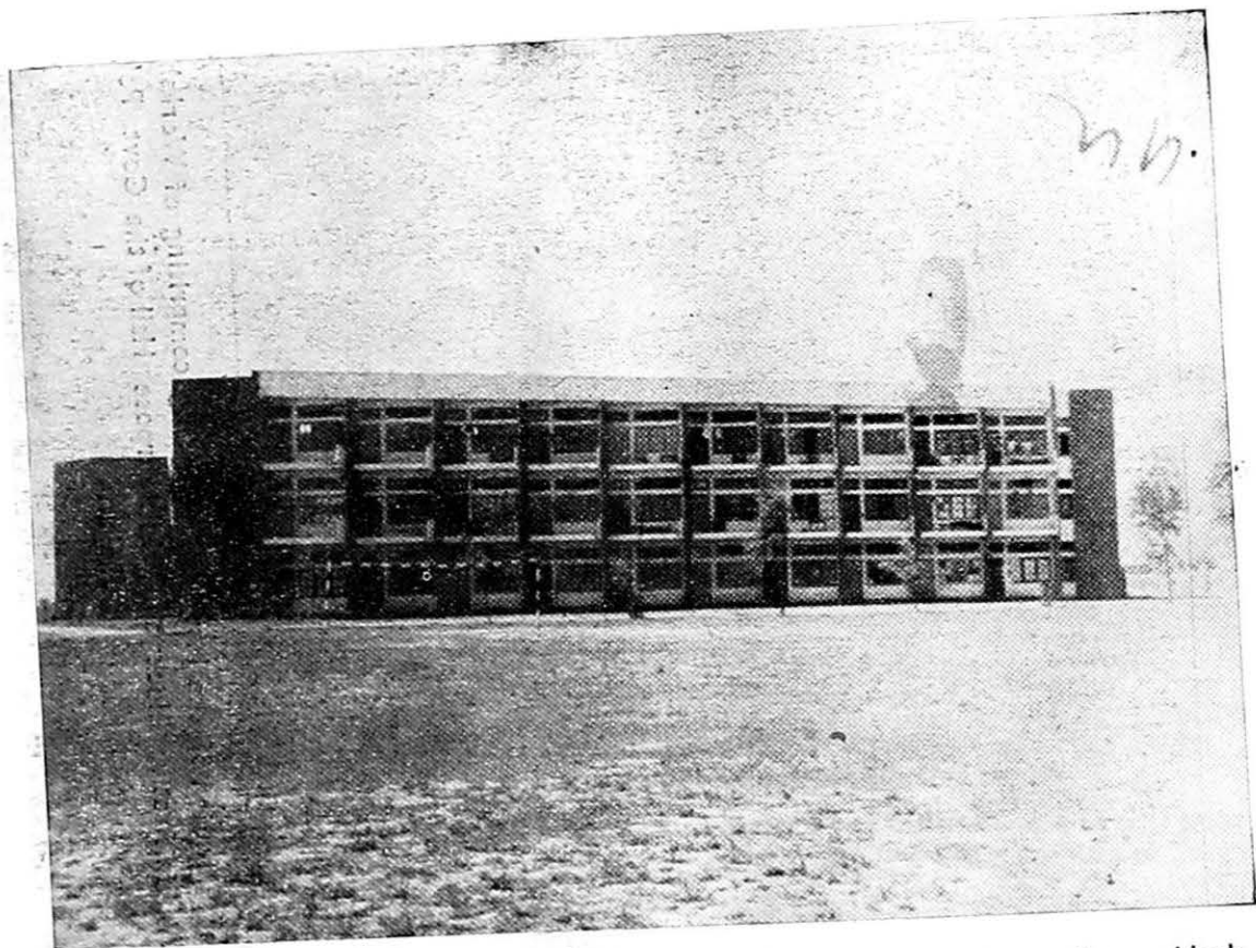
Photograph showing both the blocks of the Hostel with back elevation of one block facing the main road Govt. Polytechnic, Jhajjar.
