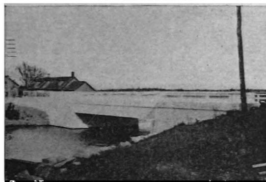
ABOVE: FAILURE OF THE OLD ONECA BRIDGE BELOW: THE NEW BRIDGE AT ONECA IN THE TOWN OF STERLING
