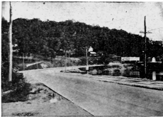
A SECTION OF THE BRIDGEPORT-WATERBURY-THOMASTON ROUTE IN THE TOWN OF SEYMOUR. THIS ROAD WHICH IS SURFACED WITH TOPEKA MIX BITUMINOUS CONCRETE IS CLASSIFIED AS A CLASS A HIGHWAY
