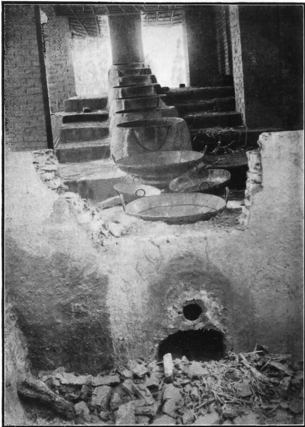
The Bhopal Bel for juice boiling. (with front wall partially removed).
