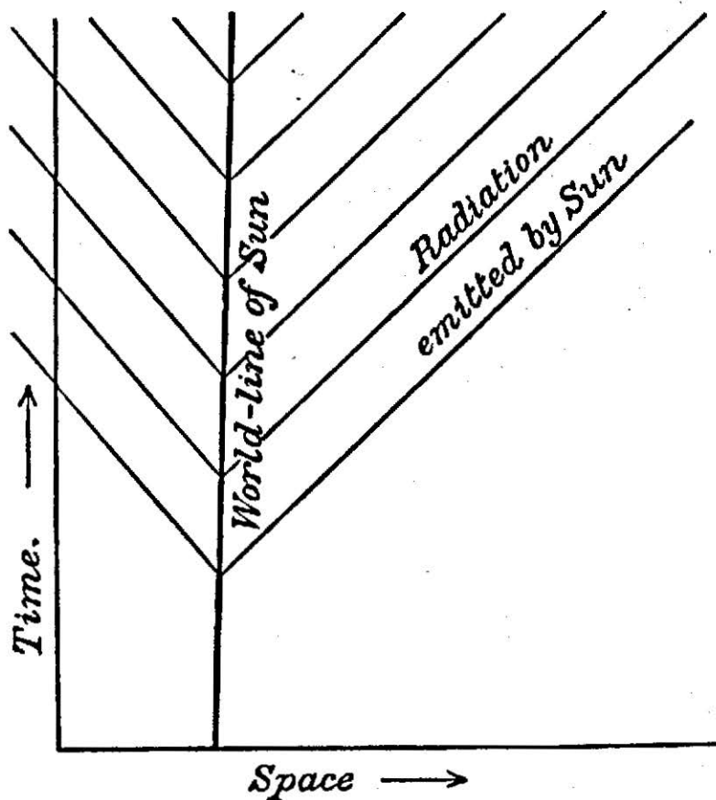
Fig. 8. Diagram to illustrate the motion of the Sun and its radiation in space and time (cf. Fig. 2 on p. 100)
