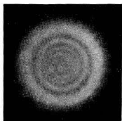
Fig. 1. Diffraction rings produced by light passing through a minute aperture (a pinhole) in an opaque screen (N. R. Fowler)
