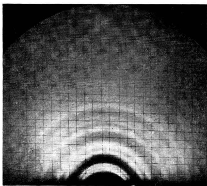
Fig. 3. Diffraction rings produced by electrons reflected off a minute area of a gold surface (G. P. Thomson)
