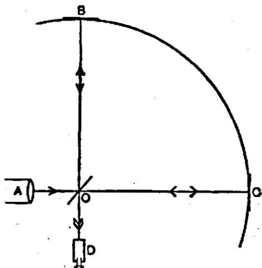
Fig. 1. Diagram to illustrate the Michelson-Morley experiment
