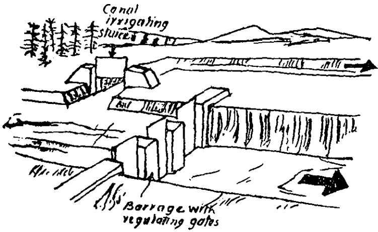
Sketch representation of small diversion weirs.
