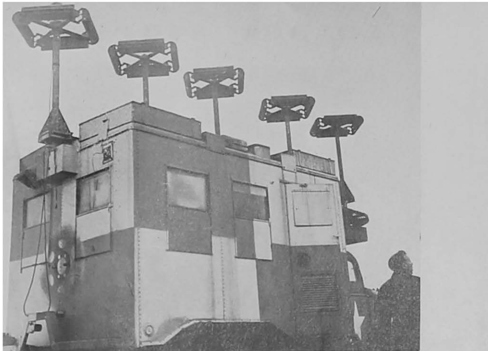
A part of the equipment used to help pilots to land. This is the Localizer Truck of the Instrument Landing System.
