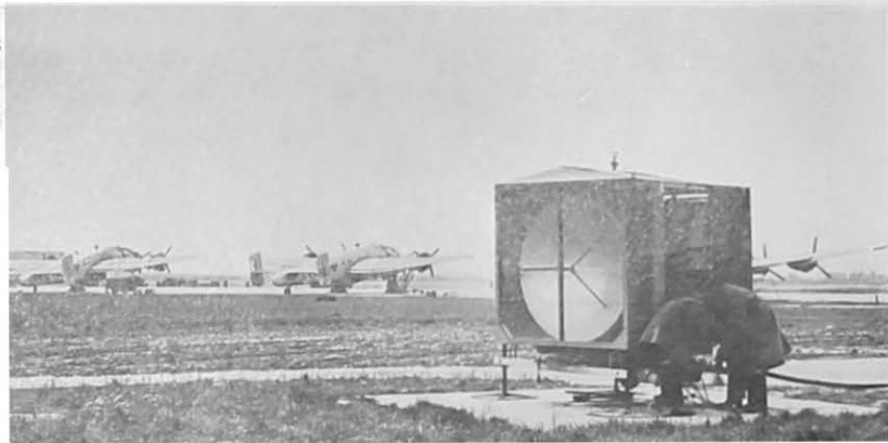
The rotating aerial head of the Airfield Control Radar equipment which can locate aircraft 25 miles away from London Airport.
